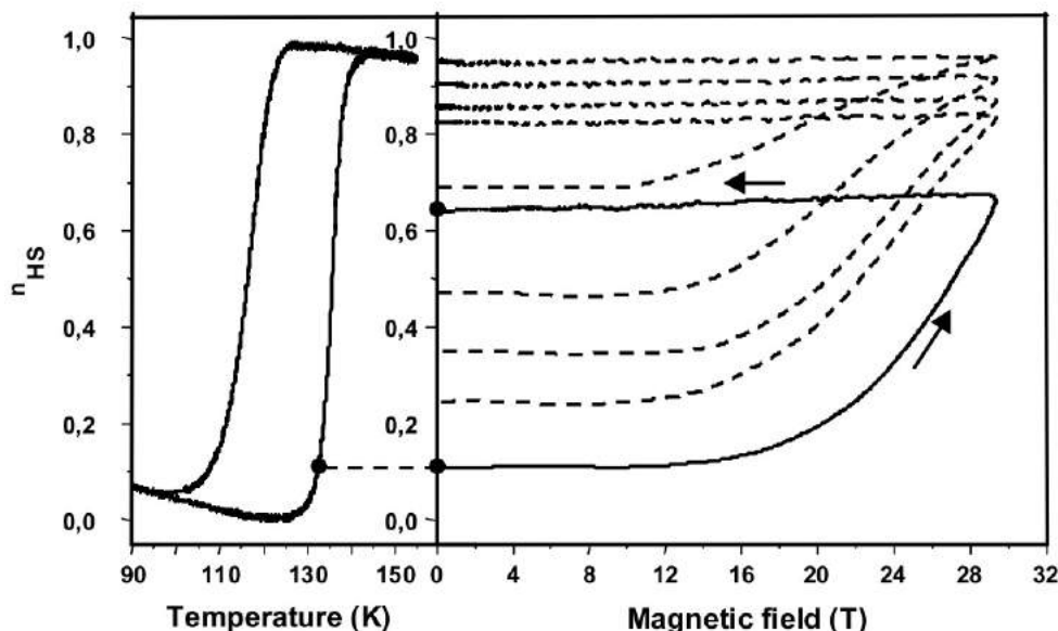
Figure 1.7: Irreversible triggering effect of \text{Co}(\text{H}_2(\text{f}sa)_2en)(py)_2 in a pulsed magnetic field in the metastable LS state [48]
