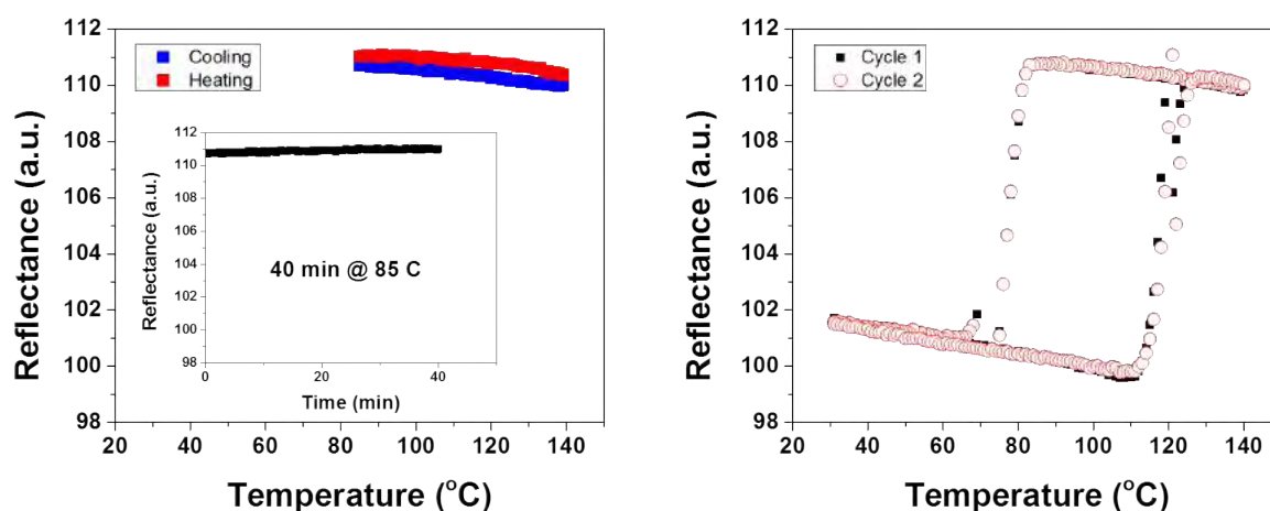
Figure 3.23: Reflectance variation in the cooling and heating modes between 140\text{ }^{\circ}\text{C} and 85\text{ }^{\circ}\text{C} in the HS state in the absence of any applied electrical field. The inset represents the variation of the optical reflectance as a function of time in isothermal conditions. No sign of the HS to LS spin transition can be inferred from these data. Two consecutive hysteresis loops are presented in the second panel (transition temperature are slightly shifted due to the fact that these measurements were performed on another synthesis batch).
