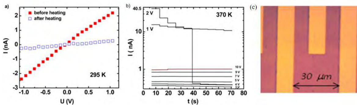
Figure 1.30: (a) Current-voltage characteristic of the ROM device with [ Fe(HB(pz)_3)_2 ] recorded at 295 K before and after heating the device to 408 K. (b) Reading and writing process of the ROM device performed at 370 K. (c) Bright field microscopy picture of the micro-electrodes after the deposition of the [ Fe(HB(pz)_3)_2 ] film [30].
