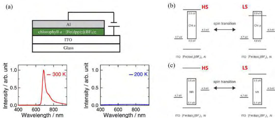
Figure 1.29: (a) Scheme of the OLED device ITO/[ Fe(dpp)_2 ]( BF_4 ) 2 :Chl- a /Al and its electroluminescence intensity in the HS and LS states. (b) Schematic representation of the mechanism proposed for the switching of EL intensity upon SCO. (c) Energy level diagram for an analog device with NR dye [86].
