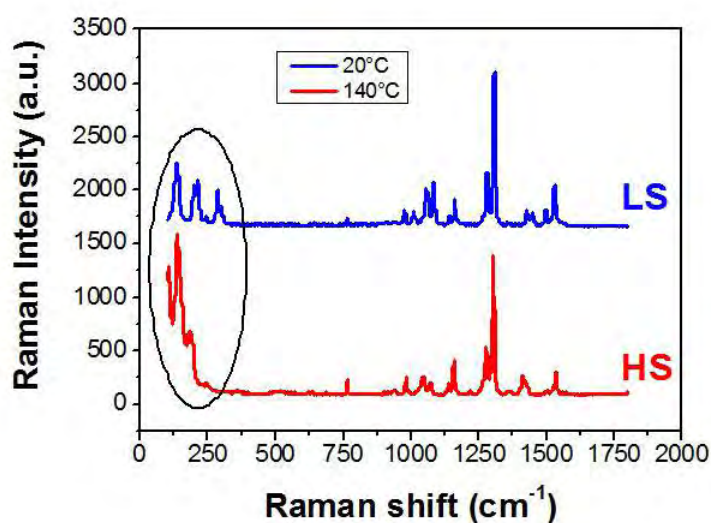
Figure 1.16: Raman spectra of the [Fe(Htrz)_2(trz)](BF_4) SCO compound in the LS and HS states.
