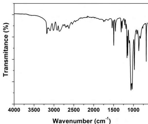
Figure 2.6: IR-ATR spectra of the bulk sample at room temperature.
