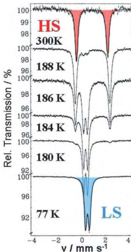
Figure 1.19: Mössbauer spectra of [\text{Fe}(\text{phen})_2(\text{NCS})_2] at different temperatures [68].
