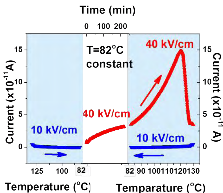
Figure 3.26: Electric field switch experiment performed at 82^\circ C . The left panel shows the current recorded when cooling the device from 130 to 82^\circ C under 10\text{ kV/cm} . The middle panel depicts the temporal evolution of the current at fixed temperature ( 82^\circ C ) and bias ( 40\text{ kV/cm} ) followed by a complete thermal cycle (right panel) between 82 and 130^\circ C .
