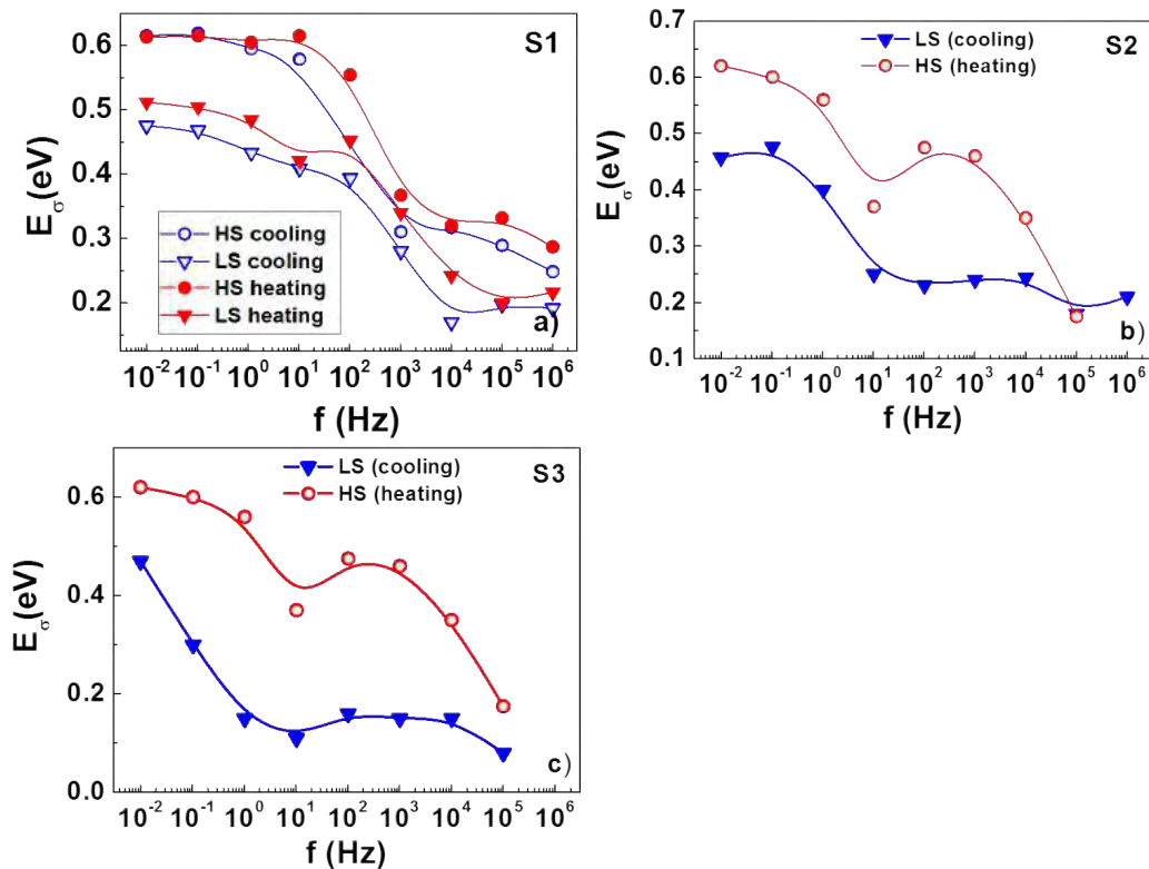
Figure 2.21: Frequency dependence of the conductivity activation energy for samples S1 - S3 in the two spin states.
