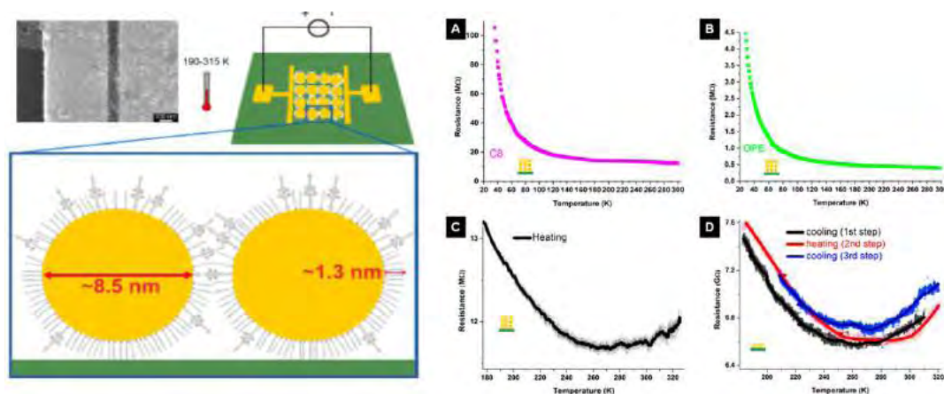
Figure 1.41: Left panel: SEM image and schematic drawing of the SCO molecule-gold nanoparticle 2D array for single molecule conductance studies. Right panel: Resistance as a function of temperature of a gold nanoparticle network with (a) octanethiol molecules, (b) dithiolated oligo(phenylene ethynylene) molecules, (c) SCO molecules (three layers) and (d) SCO molecules (monolayer) [97].
