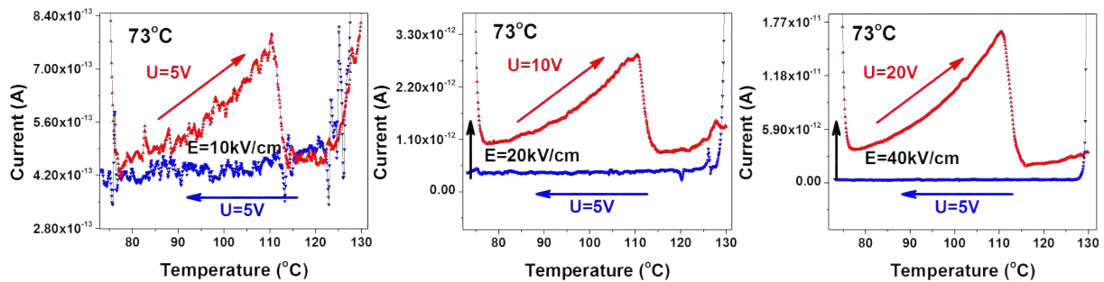
Figure 3.25: Electric-field induced HS-LS transition performed at 73 ^{\circ}C with different electric field strengths.
