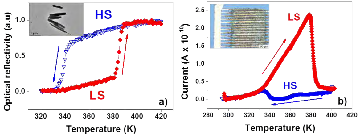
Figure 3.12: (a) Temperature dependence of the optical reflectivity ( \lambda = 540 nm) of the powder sample [Fe(Htrz)_2(trz)](BF_4) in the heating and cooling modes. The inset shows a TEM image of the particles. (b) Temperature dependence of the current intensity (at U = 20 V) in the device in the heating and cooling modes. The inset shows the photo of the interdigitated electrode device with the particles.
