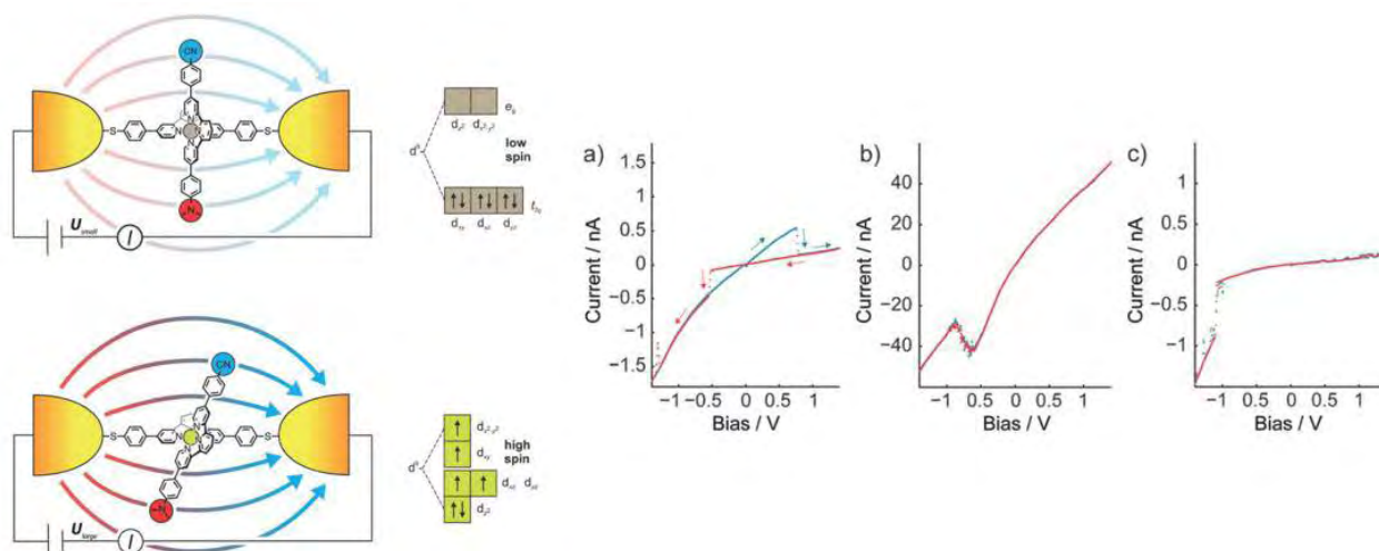
Figure 1.42: Schematic representation of the voltage triggered spin transition of the [Fe^{II}(tpy)_2] complex. I-V characteristic showing (a) hysteresis, (b) negative differential conductance and (c) a jump in current [98].
