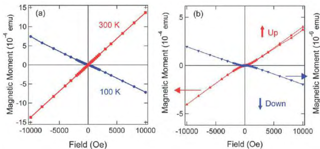
Figure 1.32: (a) Magnetic properties of [Fe(H_2B(pz)_2)_2(bipy)] powder at 100 K (LS) and 300 K (HS). (b) Magnetic properties of the films of [Fe(H_2B(pz)_2)_2(bipy)] on the ferroelectric PVDFTrFE substrate for different polarizations [87].
