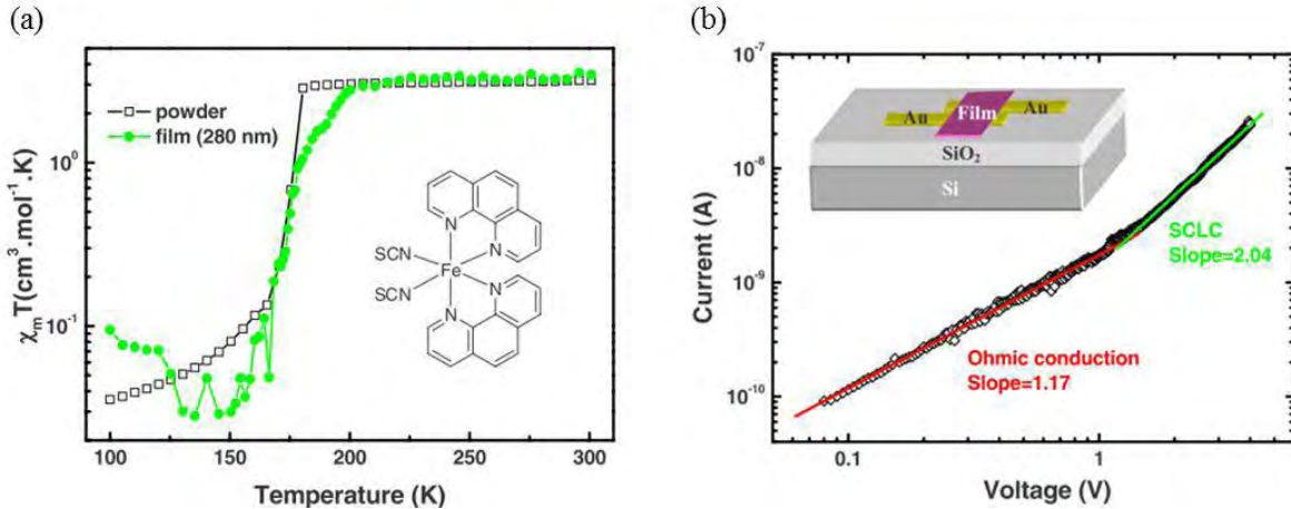
Figure 1.31: (a) \chi_M \cdot T for Fe(phen)_2(NCS)_2 powder and 280 nm thin film on silicon substrate. The inset represents a schematic representation of the molecular structure. (b) I-V characteristic of device and linear fit at room temperature. The inset is a schematic representation of the electronic device [86].
