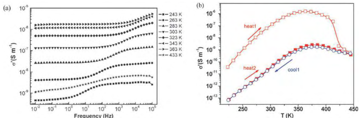
Figure 1.23: (a) Frequency dependency of the real part of ac conductivity of the [\text{Fe}(\text{HB}(\text{pz})_3)_2] complex, recorded between 243 K and 433 K during the first heating. (b) Temperature dependence of the real part of the ac conductivity recorded after two successive thermal cycles for the [\text{Fe}(\text{HB}(\text{pz})_3)_2] complex [29].
