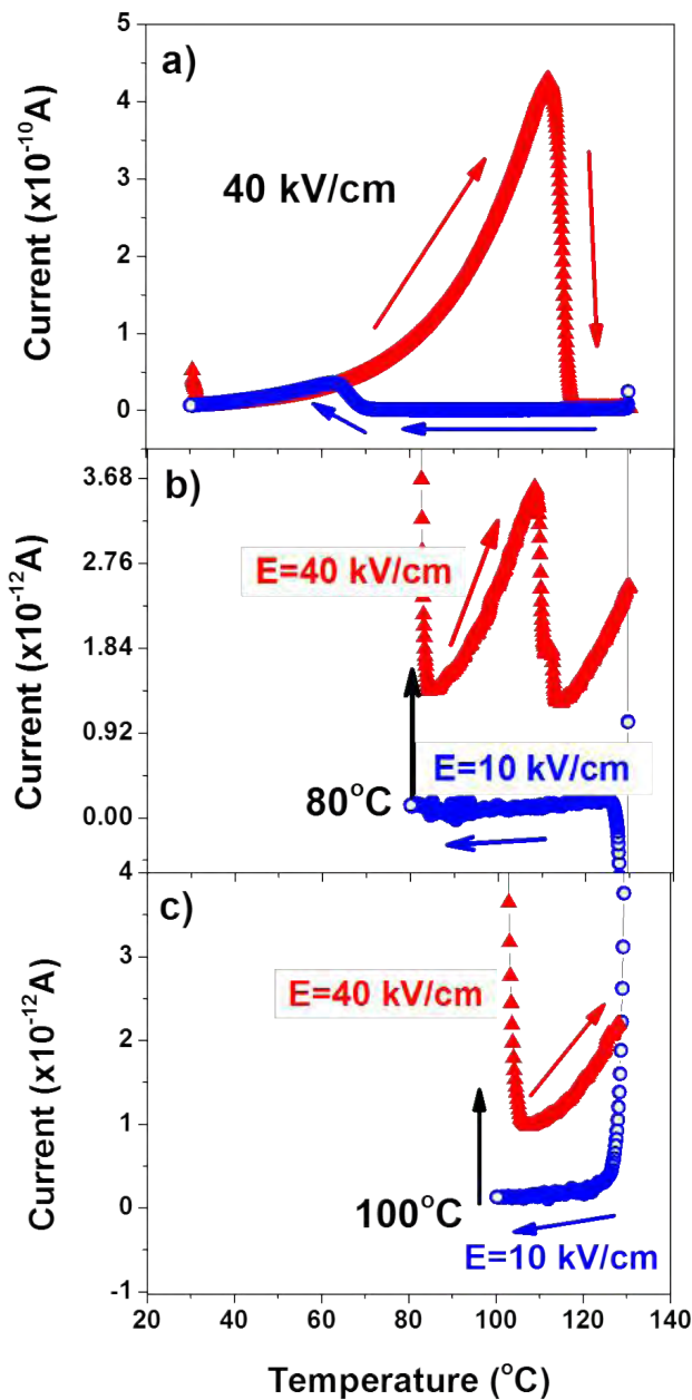
Figure 3.21: Current vs temperature characteristics of the interdigitated electrode device connected with particles of [Fe(Htrz)_2(trz)](BF_4) . Heating and cooling rates are 5 \text{ }^\circ\text{C}/\text{min} . a) Full heating-cooling cycle between 30 and 130 \text{ }^\circ\text{C} under 40 \text{ kV/cm} electric field. b-c) Incomplete thermal cycles: cooling from 130 to 80 \text{ }^\circ\text{C} (b) or to 100 \text{ }^\circ\text{C} (c) under 10 \text{ kV/cm} bias followed by heating back to 130 \text{ }^\circ\text{C} under an electric field of 40 \text{ kV/cm} .
