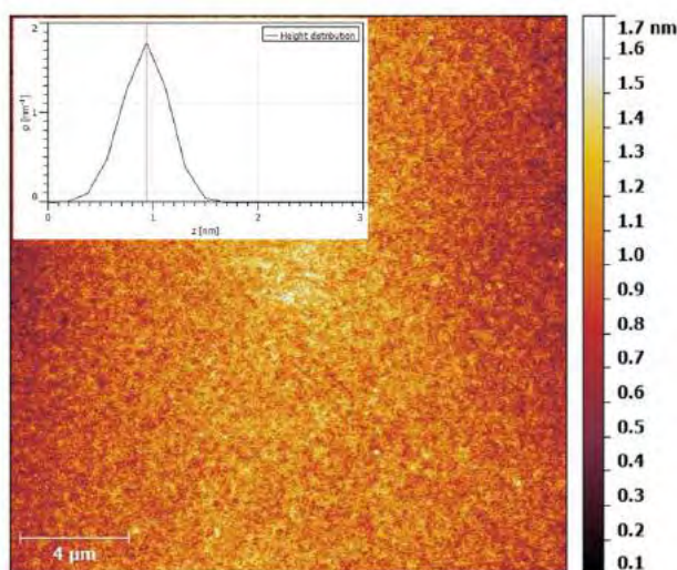
Figure 4.5: AFM topography of an area of 20 \times 20\ \mu m^2 of the deposited thin film of [Fe(bpz)_2(phen)] . The inset represents the height distribution of the measured area.
