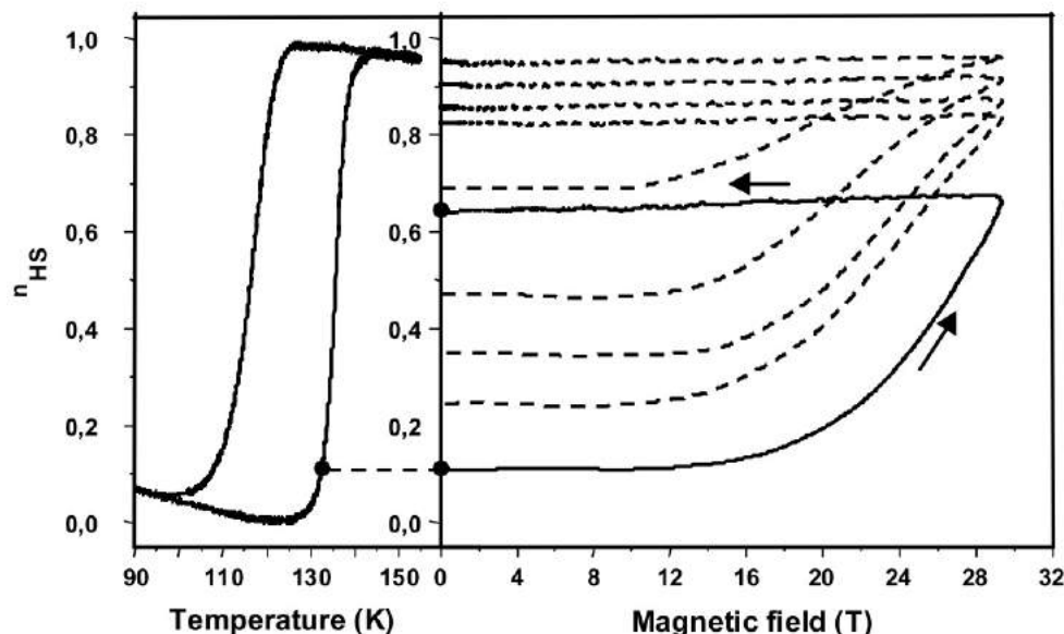
Figure 1.7: Irreversible triggering effect of Co(H_2(fsa)_2en)(py)_2 in a pulsed magnetic field in the metastable LS state [48]
