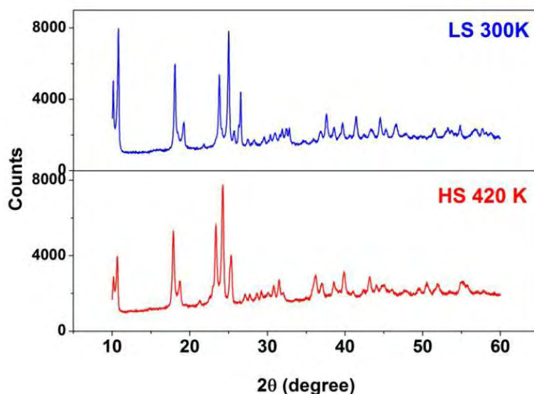
Figure 2.7: Powder XRD patterns obtained on [Fe(Htrz)_2(trz)](BF_4) in the LS and HS states respectively.
