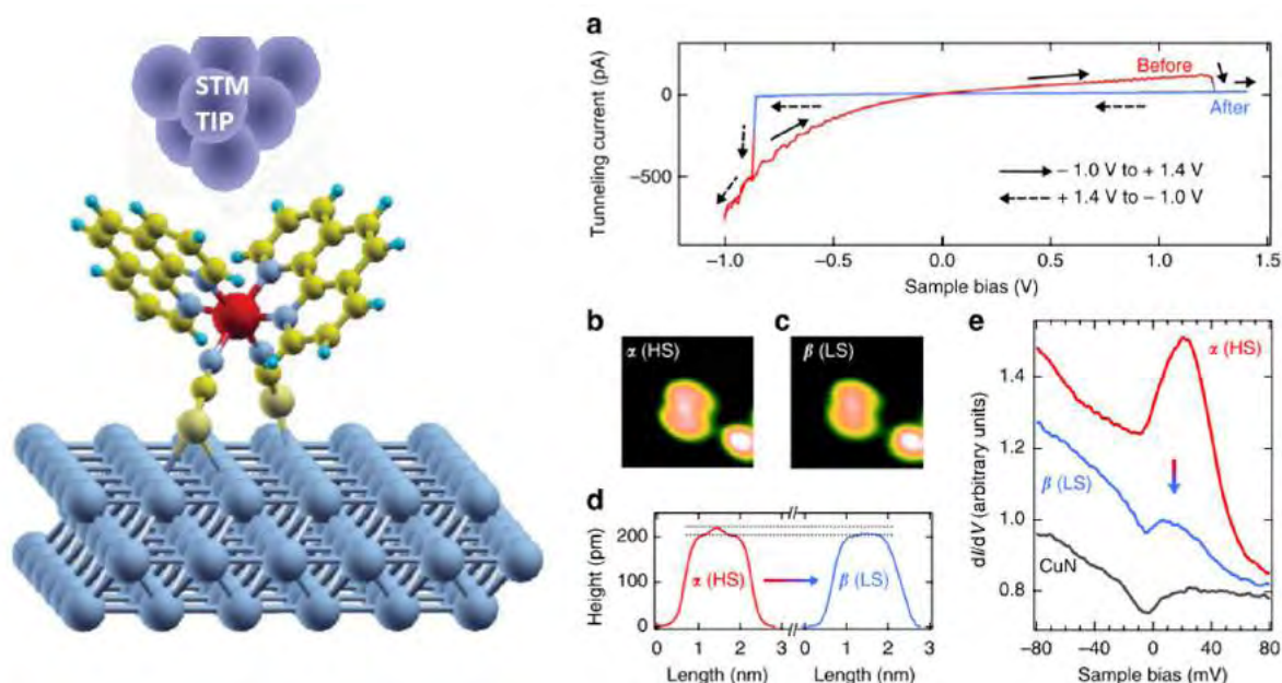
Figure 1.39: (a) I-V characteristic of an isolated Fe(phen)_2(NCS)_2 molecule on CuN/Cu(100) surface. STM image for the (b) HS and (c) LS states with the corresponding (d) height profile. (e) Differential conductivity of the molecule in the HS and LS states as well as that of the CuN insulating layer [93].
