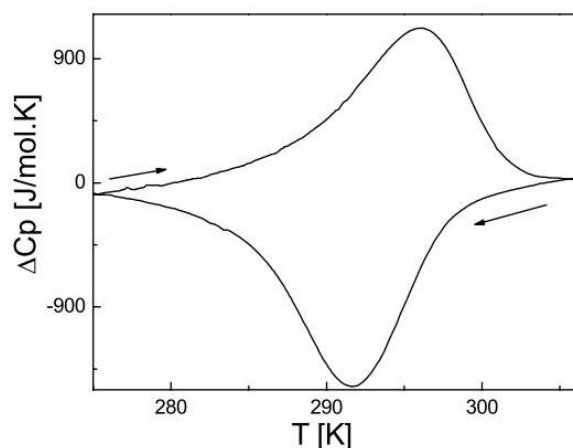
Figure 1.14: Typical calorimetric curve registered on [Fe(\text{Ethyl} - 4H - 1, 2, 4 - \text{triazole} - 4 - \text{yl} - \text{acetate})_3](ClO_4)_2 [62].
