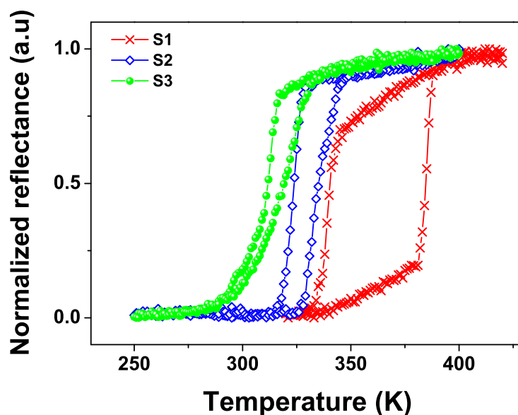
Figure 2.17: Temperature dependence of the optical reflectance at 543 nm for samples S1-S3 presenting hysteresis loops between the heating and cooling modes.
