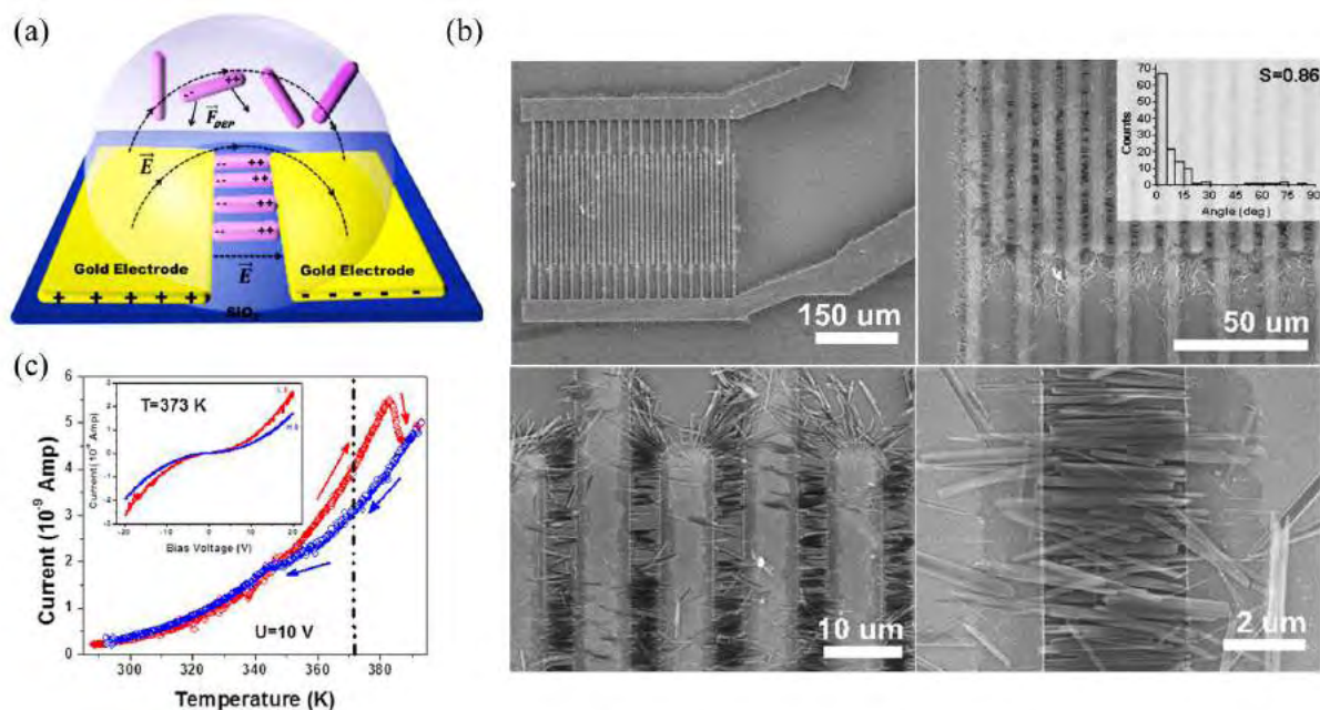
Figure 1.33: (a) Schematic representation of the dielectrophoresis process used to align [Fe(Htrz)_2(trz)](BF_4) particles between electrodes. (b) SEM images of a device with the insert showing the orientation order parameter. (c) Temperature dependence of the measured current in the device over a heating-cooling cycle under 10 V bias. Inset: I-V characteristic recorded at 373 K in the LS and HS states [31].
