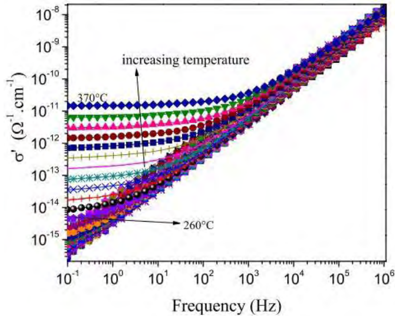
Figure 2.3: Frequency dependency of the real part of conductivity \sigma' at different temperatures for BPDA/ODA.
