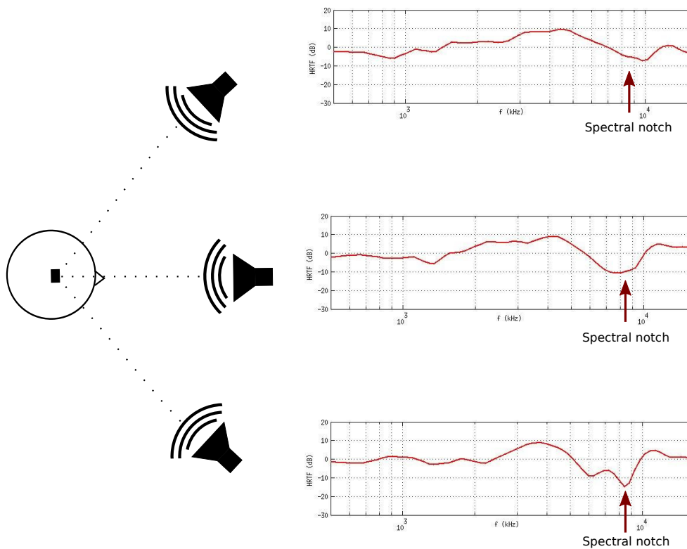
Figure 2.9: The spectral notches in an HRTF, are related to sound source elevation. Data plotted from the Cipic database [ADTA01]
