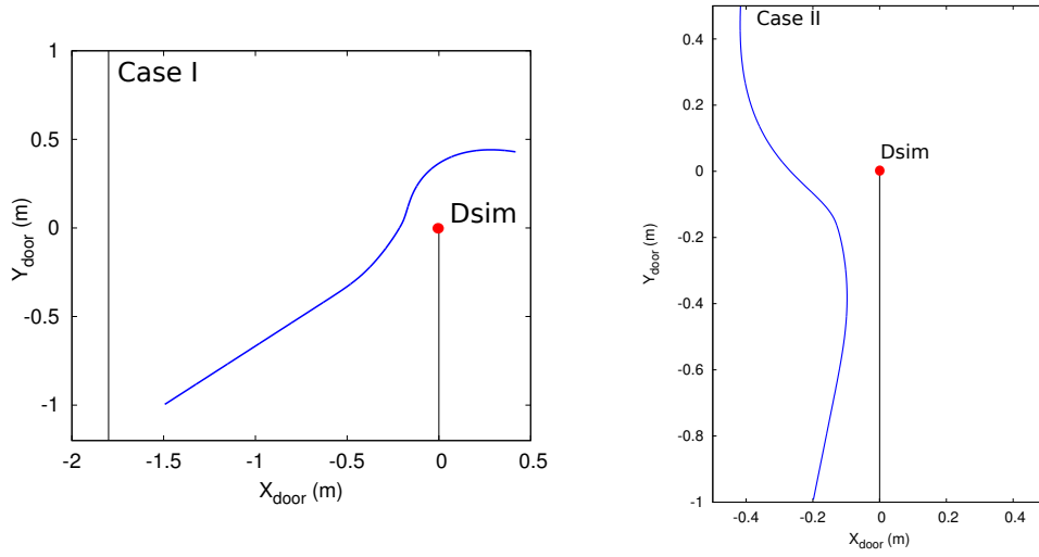
Figure 4.22: The trajectories taken by the robot for Cases I (left) and II (Right).
