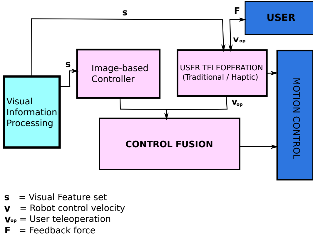
Figure 2.2: The visual feature set \mathbf{s} derived from a scene is used to drive a visual controller that generates a velocity output \mathbf{v} . The robot output is then blended with user teleoperation from a traditional or haptic interface \mathbf{v}_{op} in order to obtain a collaborative shared control system. We also illustrate a possible force feedback loop within the schematic.
