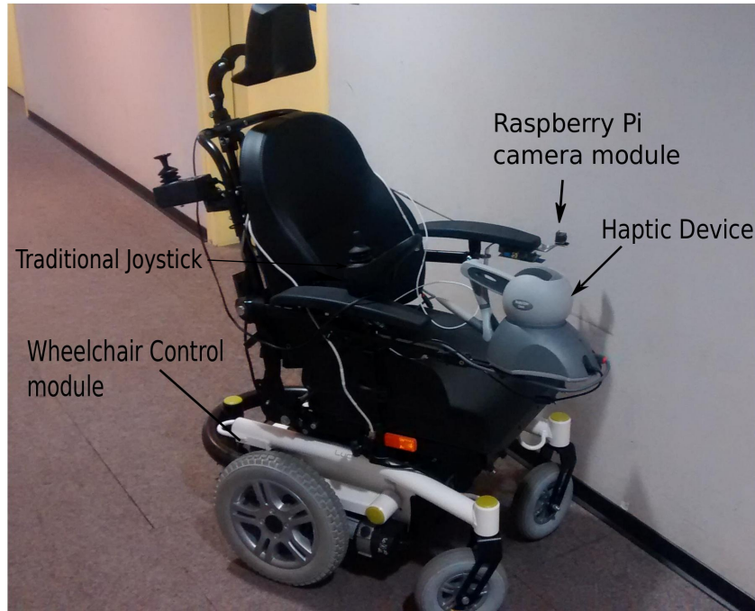
Figure 4.3: Wheelchair test platform
