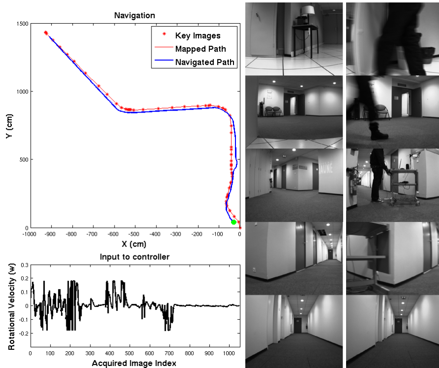
Figure 7.5 – Navigation in between the room and the corridor (left), some key images (middle), and some images during navigation (right).
