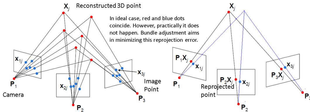
Figure 2.12 – Multiple view SfM.
