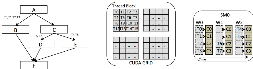
Figure 1.8: SIMT
