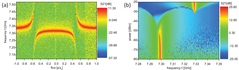
Figure 4.1. Transmission measurement of a cavity resonator coupled to a tunable transmon. a) Anticrossing when sweeping \omega_{ge} across \omega_0 using a flux bias. The two resonance peaks, separated by 2g_0 when \omega_{ge} = \omega_0 , give the coupling strength. b) Transmission around \omega_0 in the dispersive limit as a function of input power. At low power the resonance frequency is shifted due to the coupling to the transmon. When the power is increased the resonance frequency eventually switches back to \omega_0 .
