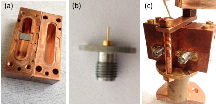
Figure 5.1. Sample and assembly parts. a) Transmon on a Si chip placed in a Cu cavity before it is closed. b) SMA coupling pin. c) Cu cavity closed and mounted on a coil, the axis of which is aligned with the transmon SQUID.
