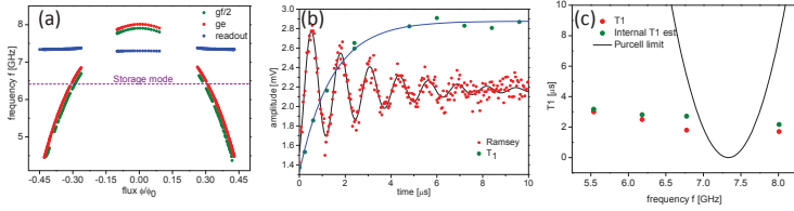
Figure 6.10. Characterization of the fourth preliminary transmon qubit. a) Mapping of f_{ge} , f_{gf}/2 and f_R as a function of flux \phi . b) Relaxation and Ramsey fringe measurements at \phi = 0 , yielding T_1 = 1.5 \mu\text{s} and T_2 = 2.8 \mu\text{s} . c) Measured T_1 (red dots) for different values of f_{ge} . Black line shows the Purcell limit of T_1 whereas the green dots show the intrinsic T_1 after removing the Purcell contribution.
