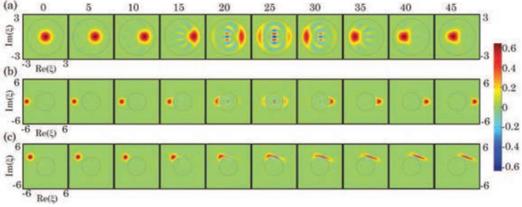
Figure 2.15. Snapshots of numerical simulations of the cavity state undergoing the QZD with \beta = 0.1 and s = 6 , at every fifth step. a) Starting in the vacuum state, the dynamics is periodic inside \mathcal{H}_{<6} , with a period of 50 steps. b) The initial state |\alpha = -5\rangle is in \mathcal{H}_{>6} . It collides with the EC from the outside and creates a superposition state at N = 25 steps. c) Starting in |\alpha = -4 + i\sqrt{6}\rangle the state collides tangentially with the EC resulting in an squeezed state. Figure reproduced from ref. [40]©.
