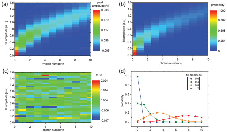
Figure 4.9. Calibration of the photon number probability measurements and the cavity filling rate. a) Raw signal amplitude of the first 11 photon number peaks. b) After a calibration procedure the amplitudes are translated into probabilities and the filling pulse amplitude into cavity field amplitude. c) Difference between the experimental calibrated probabilities and theoretical Poissonian distributions. d) Theoretical Poissonian distributions and calibrated photon number probabilities for a few fillings.
