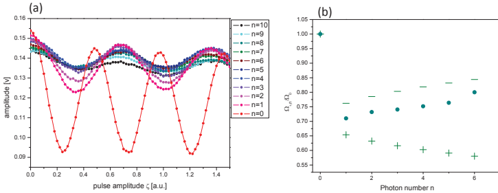
Figure 6.17. Calibration of the Fock state Rabi angles of the +, n transitions for n \in [0, 10] . a) Rabi oscillations using a Gaussian shaped pulse with varying amplitude \zeta . b) The Rabi frequencies \Omega_{+,n} normalized to \Omega_0 from measurements (dots), and numerical simulations of \Omega_{+,n}/\Omega_0 (+) and \Omega_{-,n}/\Omega_0 (-).
