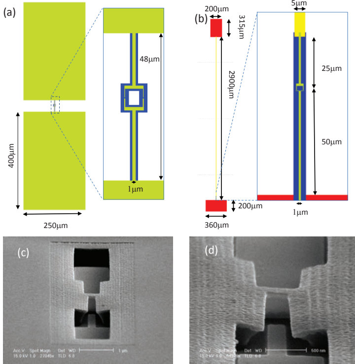
Figure 3.3. Electron beam lithography pattern of the transmons. a) and b) are snap shots of the GDSII exposure files controlling the shapes traced out by the electron beam. The color represents the dose in reference to a 250 \mu\text{C}/\text{cm}^2 nominal dose with \sim 10\% (blue), \sim 100\% (green) and \sim 190\% (red). a) The first transmon design used in a Cu cavity while the one in b) is used in the QZD experiment. c) Bilayer mask after exposure and development. We see the frame of the undercut box around the main pattern. d) Bridge in the PMMA: The bending of the structure is due to the stress induced by the imaging electron beam. c) and d) are test structure for tuning the doses of the undercut boxes and the main pattern.
