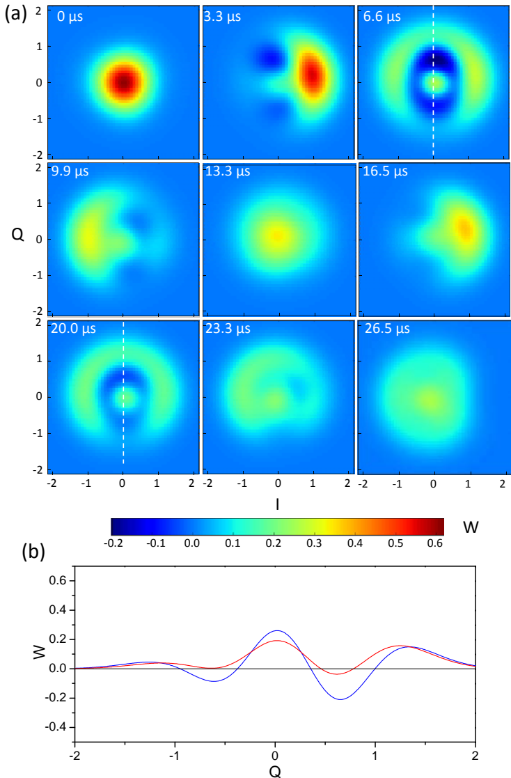
Figure 7.5. Measured QZD of the field initially in the vacuum state, confined in the exclusion circle of radius \sqrt{3} (blockade on n=3 ), and reconstructed with the maxlike method from section 4.2.4. Here p_{n,\beta} is measured for n \in \{0, 1, 2, 3\} and \beta \in \{0, 1, -1, i, -i\} , and the reconstructed density matrix is 4 \times 4 . a) Snap shots of the Wigner function taken every quarter-period, at times indicated in each frame. b) Cross section of the Wigner function after 0.5 (blue) and 1.5 (red) periods.
