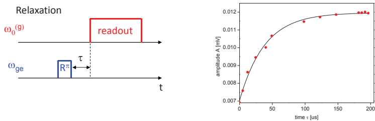
Figure 4.6. Relaxation time: protocol and example measurement. By exciting the transmon and varying the time before its state is read out, one can map the exponential decay. Here T_1 = 39 \mu\text{s} .
