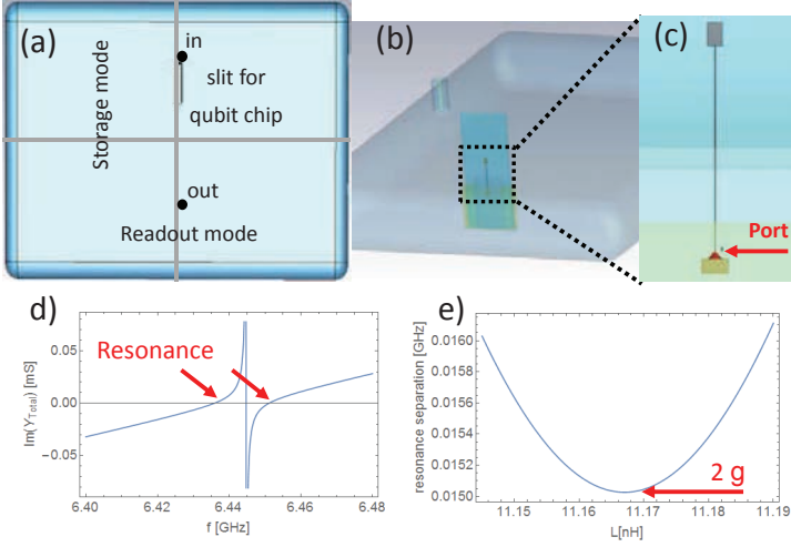
Figure 1.4. Design and simulation of the system. a) Schematic of the geometric distribution of the storage and readout mode within the cavity, the input port and are shown at the node/antinode of the storage/readout mode. b) A screen shot of the of the finite-element simulation cavity. c) A zoom-in on the simulated transmon with a port at the location of the SQUID. d) The simulated admittance \text{Im}[Y(\omega)] after adding the SQUID inductance. The roots \text{Im}[Y(\omega_{\text{res}})]=0 represent resonance frequencies. e) The anticrossing is simulated varying the SQUID inductance. The minimum separation is the coupling strength g_0 .
