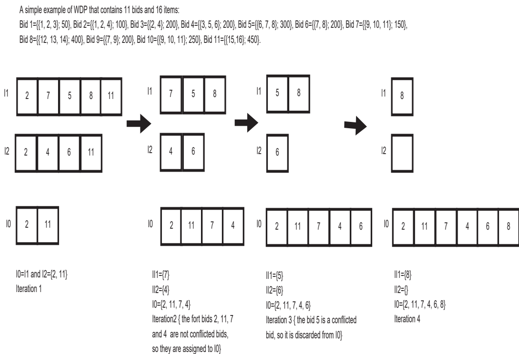
Figure 5.1 – An example of the recombination operator of MAOM-WDP algorithm
