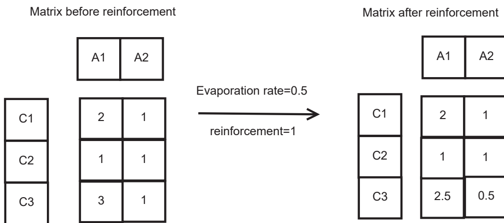
Figure 2.3 – An example of reinforcement learning with the decision matrix
