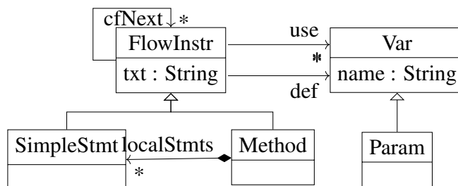
Figure 2.5 – Control-Flow metamodel excerpt
