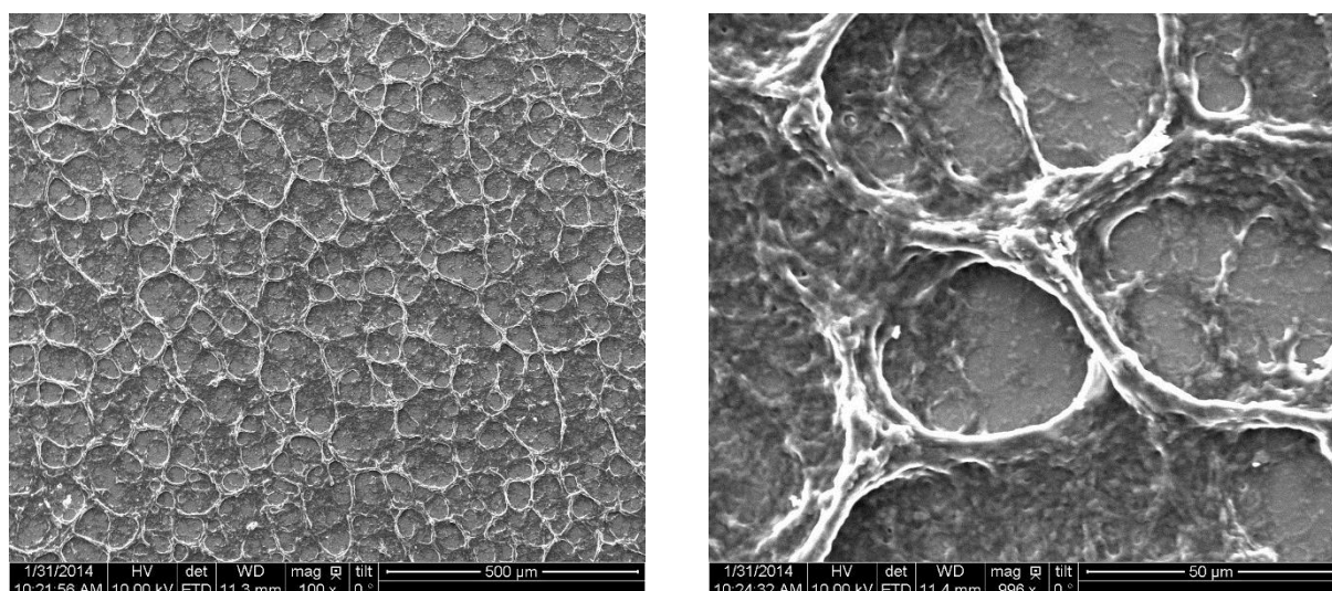
Figure III-27 : Image MEB d'un film multicouche (PDDA/PEDOT:PSS PH ) 50 , C PEDOT:PSS 1 g.L -1 , C PDDA 0,50 g.L -1 , pH 5,5.
