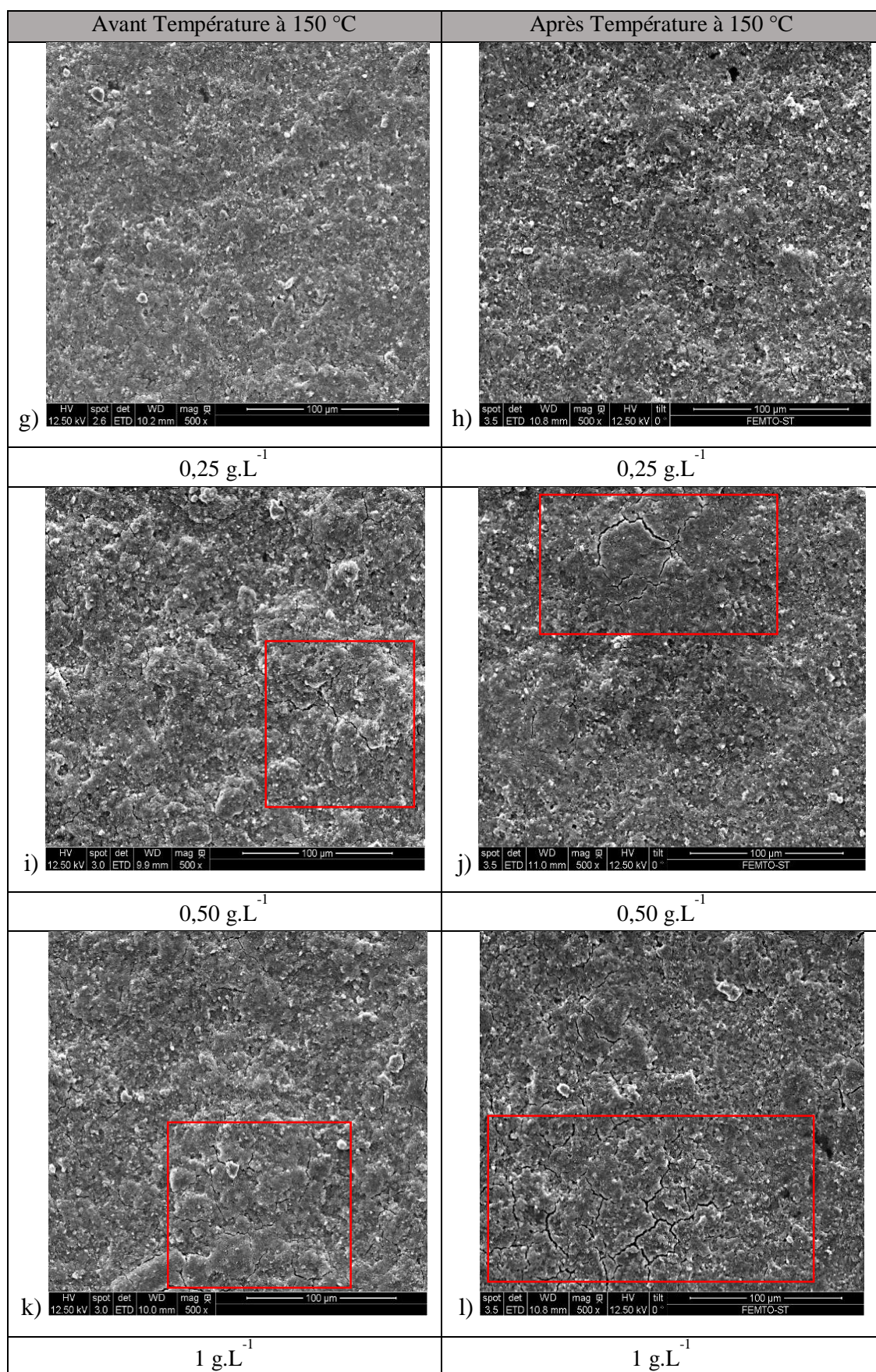
Figure IV-16 : Images MEB des films (PDDA/Al 2 O 3 -PEDOT:PSS) PH ) 10 Zoom X500, C PDDA 0,25-1 g.L -1 , C Particule 10 g.L -1 .
