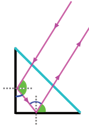
Figure 2.10 – Scheme of the optical path within corner-cube retro-reflectors. Congruent angles are indicated with the same colors; dashed grey lines indicate the perpendicular direction to the reflective surfaces at reflection points. The geometric structure ensures that the reflected beam is parallel to the incoming one. Corner cube reflectors are mounted on several SLR dedicated missions, such as LAGEOS, AJISAI and Starlette, and on navigation satellites, such as GPS, GLONASS and GALILEO. In the first case, retroreflectors are typically embedded in the satellite structure, while in the second they are usually displayed in planar arrays of different sizes and geometries according to the spacecraft block. The SLR geodetic mission BLITS, decommissioned in 2009 after collision with space-debris, proved the efficiency of the Luneburg lens concept as possible alternative to the corner-cube technology.
