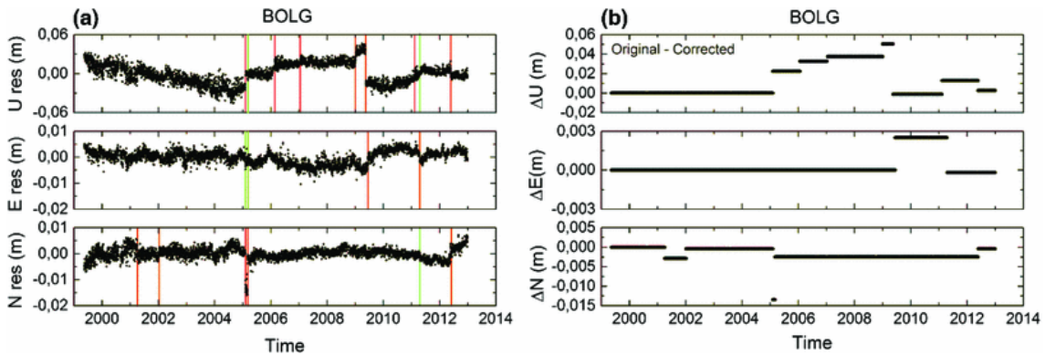
Figure C.8 – BOLG station: a Up, East and North residuals of the original GPS coordinate time series. Red lines indicate the detected discontinuities; green lines indicate cable replacement and reference system change. b Difference between the original and the corrected Up, East and North coordinate time series; the scales are different from those of panel a to clearly distinguish the magnitude of the discontinuities
