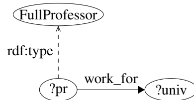
FIGURE 1.7 – Patron de graphe SPARQL
