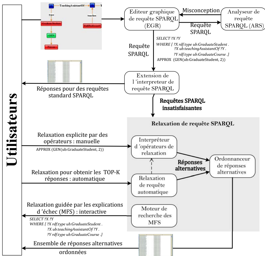
FIGURE 4.7 – Architecture de QaRS
