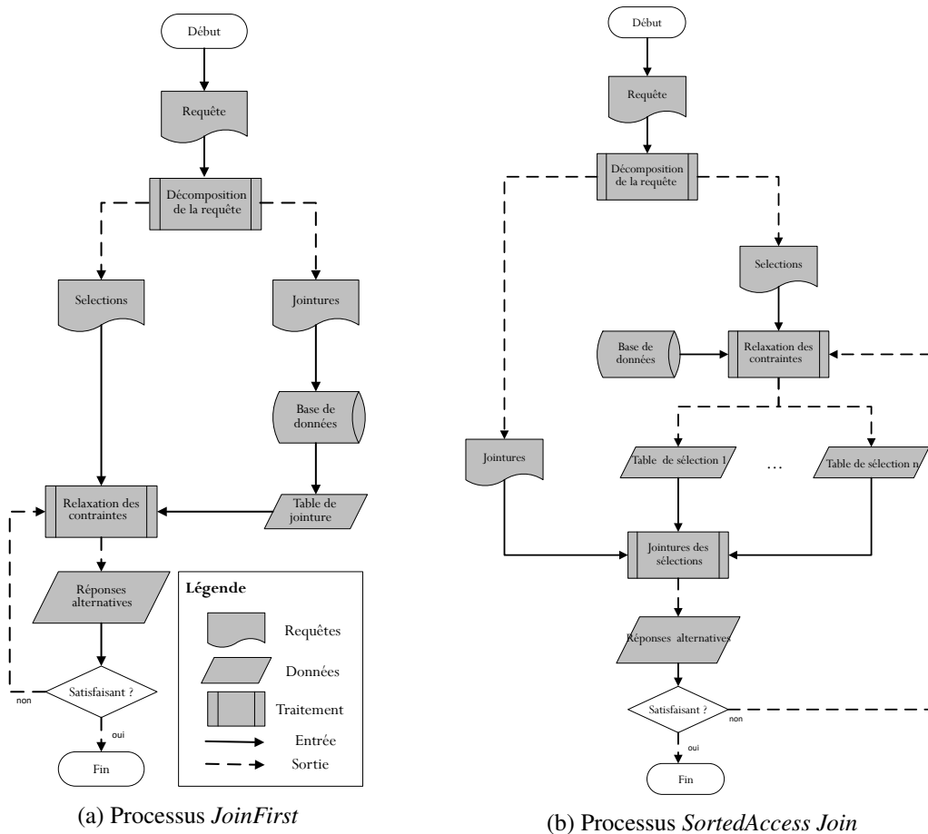
FIGURE 3.3 – Processus de relaxation des jointures
