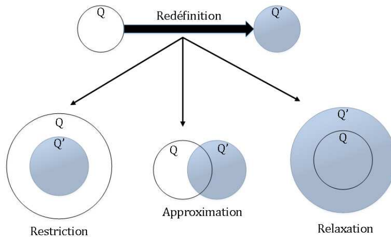
FIGURE 2.3 – Approche de modification de requête (source [163])
