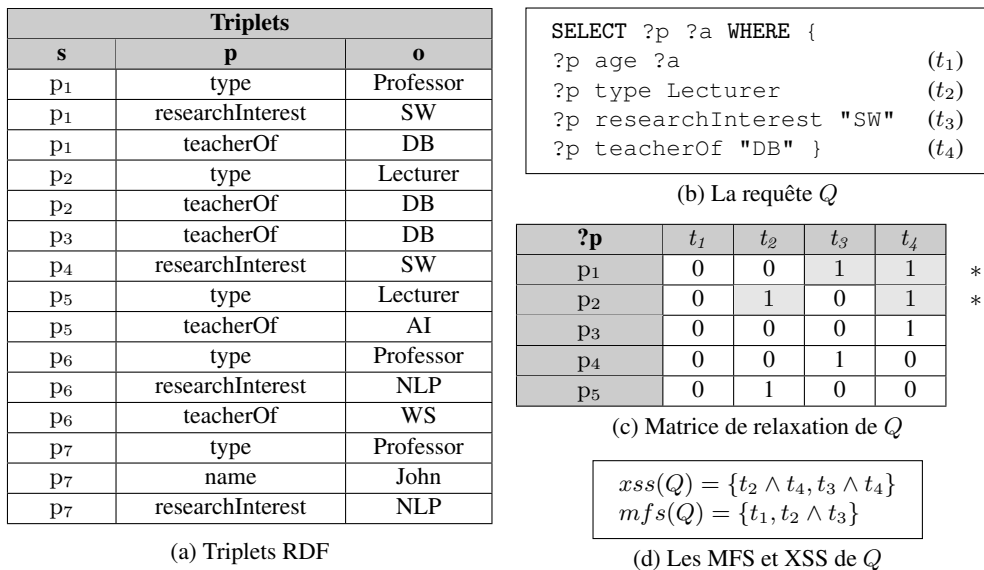
FIGURE 5.9 – Illustration de l'approche MBA
