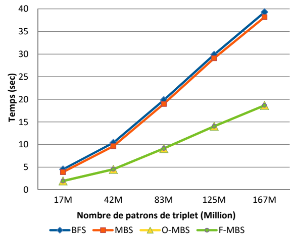
FIGURE 6.10 – Temps Vs Taille (log )
