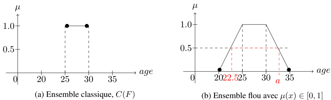
FIGURE 4.1 – Ensemble flou
