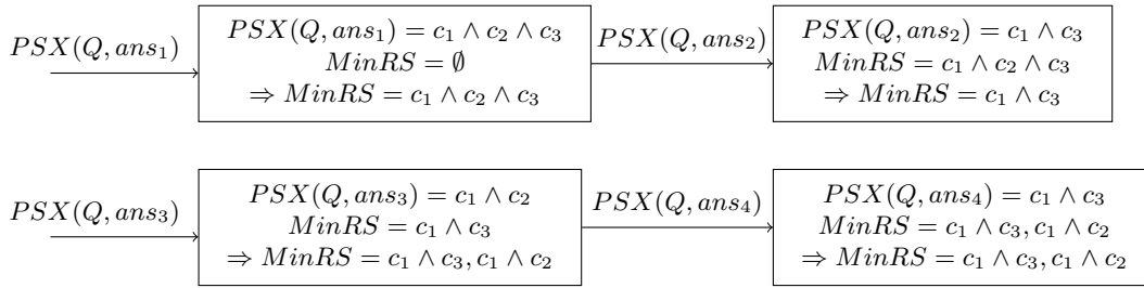
FIGURE 3.7 – Recherche des relaxations minimales
