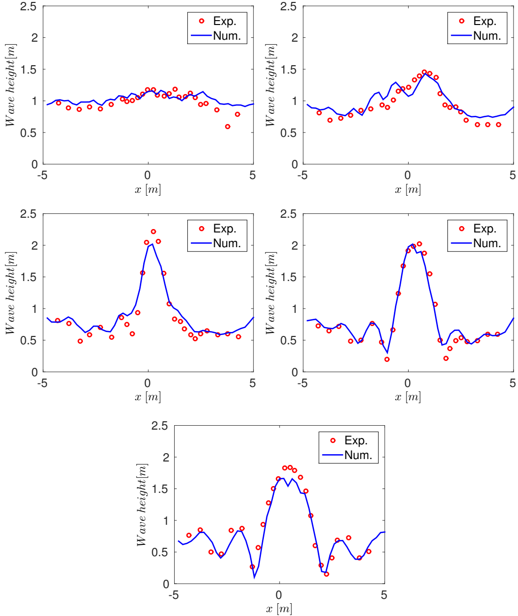
Figure 5.22: Wave diffraction over an elliptic shoal: comparison of the computed average wave height with the experimental data of Berkhoff et al. [1982] (sections 1 to 5).
