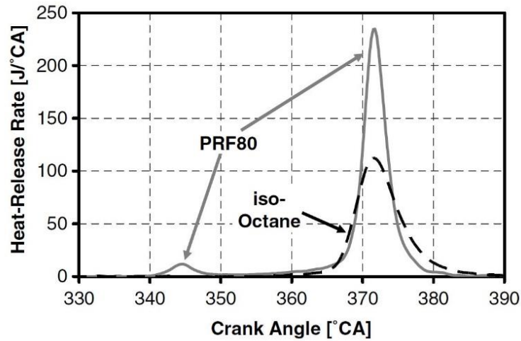
Figure 18. Heat release rate traces for isooctane and PRF80 (80% isooctane and 20% n-heptane) [27]. Isooctane combustion is in single stage while PRF80 is in two stages. The first stage between 340 and 350 °CA corresponds to the low temperature regime or cool flame. The area from 350 to 360 °CA is related to the negative temperature coefficient (NTC) regime and after 360, the peaks corresponds to the main combustion.
