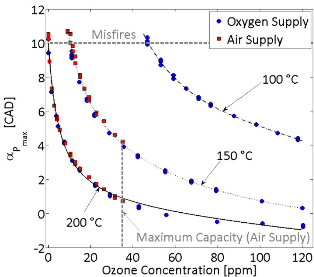
Figure 77. B. Phasing of the maximum pressure location as a function of the ozone concentration for an oxygen supply and an air supply.
