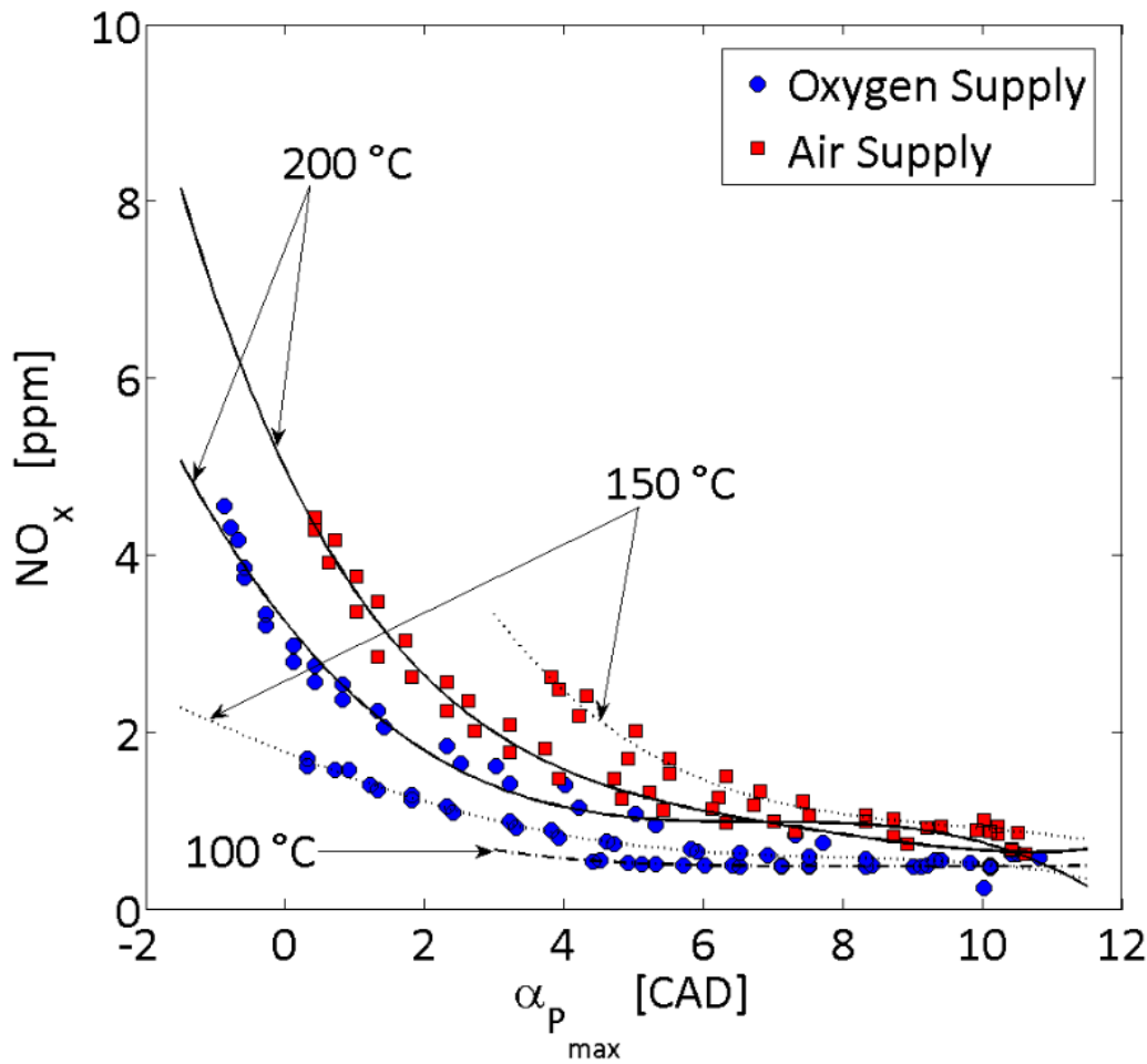
Figure 84. Nitrogen oxides trends as a function of the maximum pressure location.
