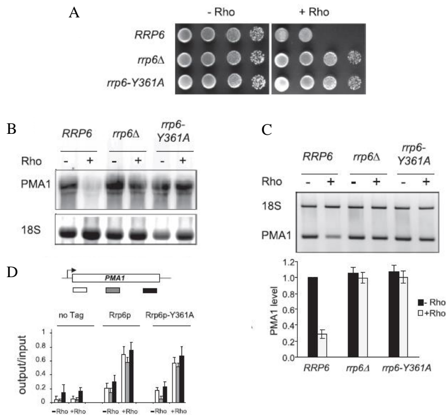
Figure 3.2: Exonuclease activity of Rrp6 is necessary for degradation of Rho-induced aberrant transcripts. (A) A 10-fold serial dilution test on BMA41 wt strain ( RRP6 ), rrp6Δ mutant and a strain harboring the catalytically inactive Rrp6 ( rrp6-Y361A ), all of which were transformed with the Rho expression plasmid pCM185-Rho-NLS. Strains were grown in selective liquid medium under non-inducing conditions (1 \mu g/mL Dox) and spotted onto Rho-repressing (+Dox) or Rho-inducing (-Dox) plates and left to grow for three days at 25°C. (B) Northern blot assay performed on the same strains as in (A). Total RNA was extracted from strains grown under Rho-repressing (1 \mu g/mL Dox) or Rho-inducing (without Dox) conditions. RNA samples (12 \mu g) were fractionated on an agarose gel and transferred to a membrane. Steady-state levels of PMA1 transcript were detected by a 5' end-labeled probe. The loading control 18S rRNA was visualized by ethidium bromide staining of the gel before membrane transfer. (C) Semiquantitative RT-PCR analysis performed on total RNA (1 \mu g) samples from strains as in (A), (B). Visualization was made using specific primers for PMA1 mRNA and 18S rRNA and ethidium bromide staining. Histogram shows PMA1 abundance relative to 18S rRNA as determined by quantitative RT-PCR. PMA1 signal for BMA41 wt strain in absence of Rho-expression is set to 1 as a reference value. The average of three independent experiments is shown, with error bars representing S.D. (D) Quantification by real-time PCR of ChIP samples obtained from yeast wt strain ( no Tag ) or strains harboring Myc-tagged Rrp6 variants, grown either in repressing (- Rho ) or inducing (+ Rho ) conditions. Immunoprecipitated ( output ) samples were normalized to input as in Fig. 3.1 for regions 5', middle and 3' as represented schematically. The average of three independent experiments is shown, with error bars representing S.D.
