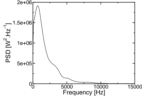
Figure 2.9: Power spectral density of the heat release rate using Welch's method, with 5 blocks, 50 % overlapping, zero-padding and a frequency resolution of \Delta f = 170 Hz.
