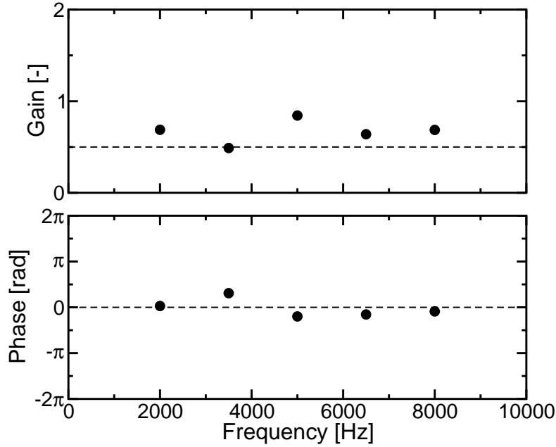
Figure 2.60: Flame transfer function of the pressure modulation cases. • FTF results from the large eddy simulations of pressure modulation without the influence of the induced velocity , -- modeled flame transfer function .
