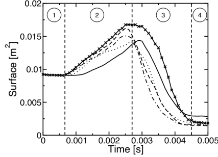
Figure 1.11: Evolution of the iso-density surface equal to 100 \text{ kg.m}^{-3} with time during the transient period for a constant modulation amplitude of 25 \text{ m.s}^{-1} (a) – VA_{25}^{0.1} , \dots VA_{25}^{0.3} , \cdot\cdot\cdot VA_{25}^{0.8} , -\cdot- VA_{25}^{1.6} , \times - \times VA_{25}^{3.2} .
