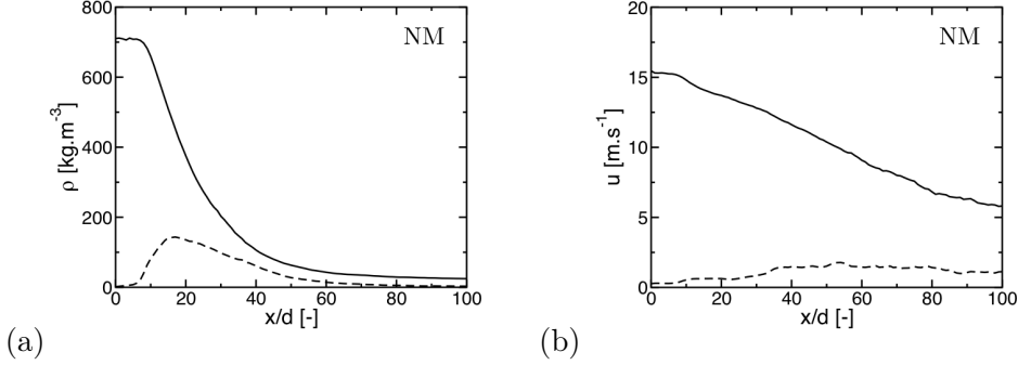
Figure 1.7: Evolution of (a) density and (b) axial velocity along the central axis for NM. — Mean value, - - rms value.
