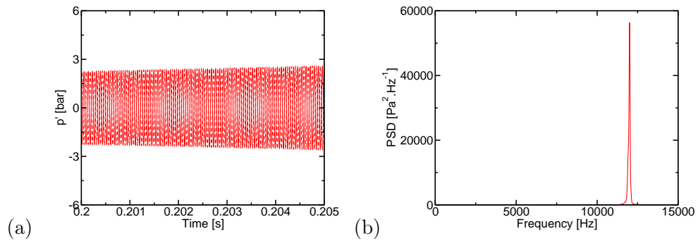
Figure 8.12: (a) Temporal evolution and (b) Power spectral density of the pressure fluctuation inside the BKD test rig for LP_4 using Welch's method, with 5 blocks, 50 % overlapping, zero-padding and a frequency resolution of \Delta f = 20 Hz.
