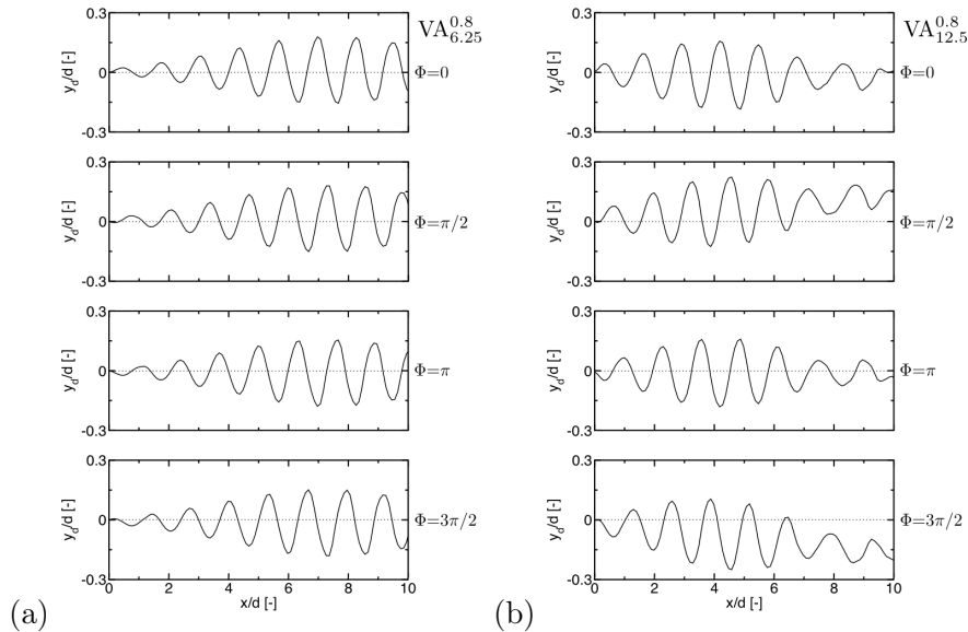
Figure 1.17: Evolution of the jet centerline for (a) VA_{6.25}^{0.8} and (b) VA_{12.5}^{0.8} . — Phase averaged centerline position, \cdots average centerline position.
