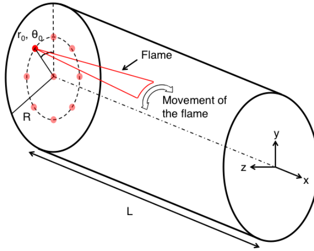
Figure 7.3: Schematic view of a moving flame in a cylindrical geometry. The length and radius of the domain are L and R respectively, the initial position of the flame is (r_0, \theta_0) .
