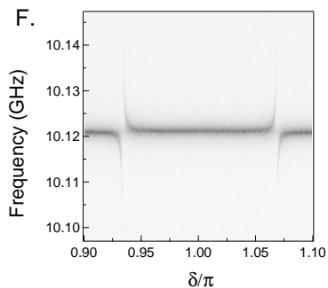
A single channel crossing \tau = 0.9983 \omega_A/2\pi = 3.66 GHz
