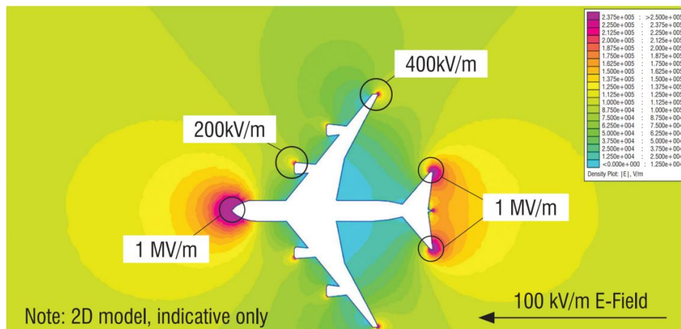
Figure I.5. Indicative 2D electrostatic model of an aircraft in a 100 \text{ kV m}^{-1} ambient field calculated by Morgan et al. (2012).
