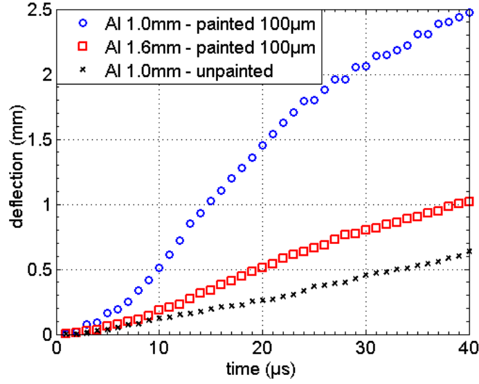
Figure VI.26. Measurements of the deflection at the panel center.
