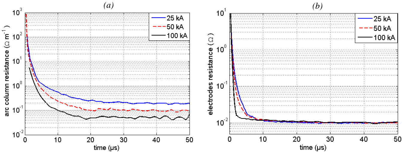
Figure IV.9. (a) Arc column resistance and (b) electrodes resistance obtained from linear regressions of each time step and using different arc lengths.
