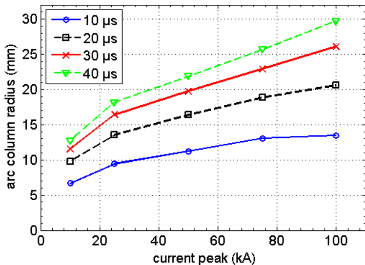
Figure III.7. Arc column radius versus the current peak for different times.
