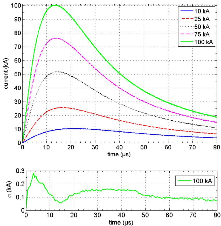
Figure II.3. Average of the measured current waveform produced with the experimental setup. On bottom part the standard deviation for the 100 kA peak level calculated using 20 shots.
