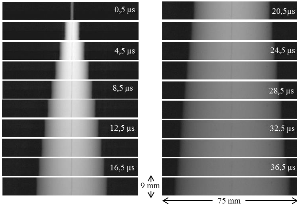
Figure III.5. Pictures of the column expansion during the first 38.5 \mu\text{s} . Experimental parameters – current peak: 100 kA; resolution: 256 \times 32 pixels; scale: 0.29 mm/pixel; exposure time: 300 ns.
