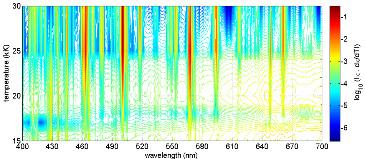
Figure V.1. Contour plot of \log_{10}(|\kappa \cdot d\kappa/dT|) calculated with a fixed pressure of 15 bar.
