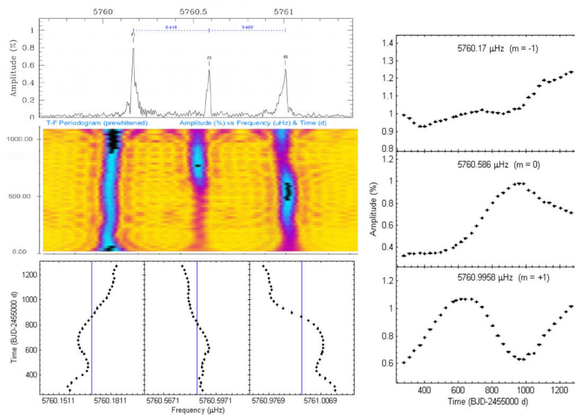
Fig. 1. Frequency and amplitude modulations of the dominant triplet near 5760 \mu\text{Hz} .
