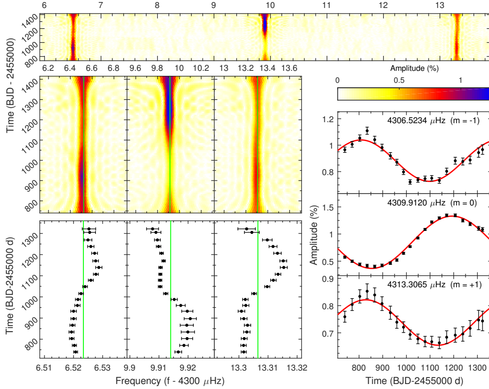
Figure 1. Amplitude and frequency modulations in the triplet near 4310 \mu\text{Hz} in the DB white dwarf star KIC 8626021. The color panels represent the sliding Lomb-Scargle periodogram. The vertical solid lines are the averaged values of the frequencies. Each data points in the bottom left and lower right panels are obtained from prewhitening subsets of the photometric data. The red solid curves denote the best sinusoidal fittings of amplitude variations. One can see more details in Ref. [11].
