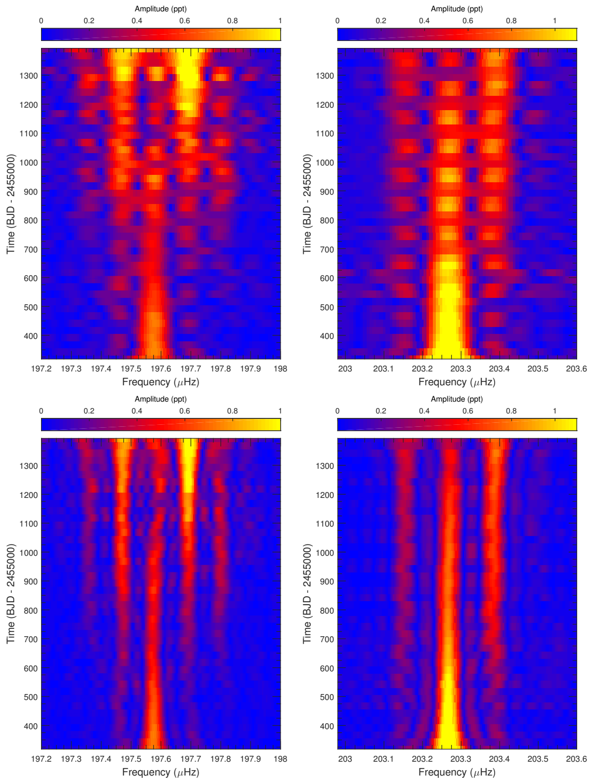
FIGURE 3.8 – Sliding LSPs of the 197.6 \mu\text{Hz} quintuplet and the 203.3 \mu\text{Hz} incomplete quintuplet with different filtering windows in KIC 10670103. The color scale represents the amplitude and the colorbar is shifted to the up side of each panels. As a comparison, the two top panels are built with window width of 150 d and the two bottom panels are built with a wider window, 300 d, which, obviously, gives a different frequency resolution.
