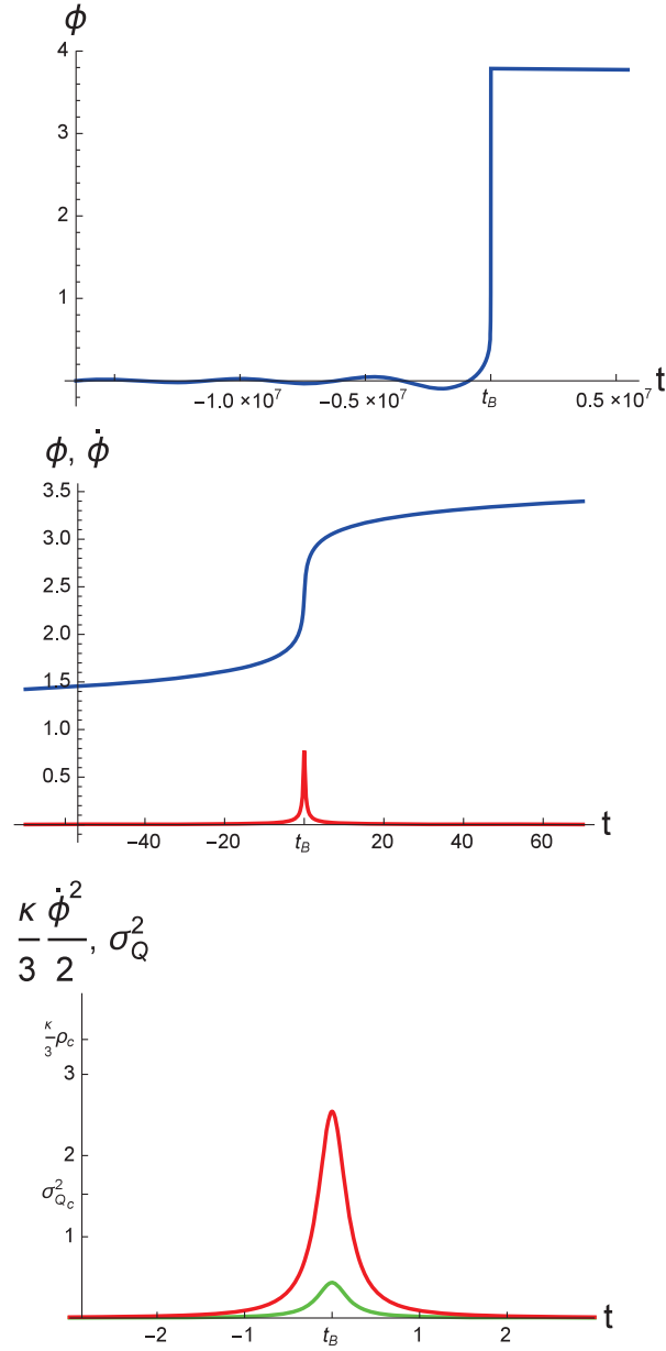
Figure 1. Typical evolution of \phi , \dot{\phi} , and \sigma_Q^2 as a function of time. t_B is the time of the bounce, when H = 0 . The blue line is \phi , the red is \dot{\phi} or \frac{\kappa}{3} \frac{\dot{\phi}^2}{2} , and the green is \sigma_Q^2 . All the above plots are from the same simulation. Note that the kinetic energy is always completely dominating over the potential energy at the bounce \frac{\dot{\phi}_B^2}{2} \gg \frac{m^2 \phi_B^2}{2} . The fraction of shear and potential energy at the bounce varies, depending on the initial conditions. The initial conditions are \sigma_Q^2(0) = 10^{-3} \frac{\kappa}{3} \rho_0 , S = 0 and \delta = 0 .
