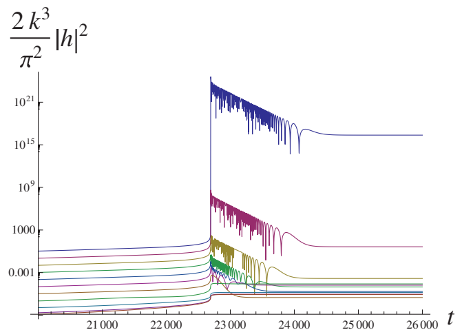
FIG. 3 (color online). Mode amplitudes as a function of time, corresponding (from top to bottom, at t = 20000 ) to k = 10^2, 10^{1.5}, 10^1, 10^{0.5}, 1, 10^{-0.5}, 10^{-1}, 10^{-1.5}, 10^{-2}, 10^{-2.5}, and 10^{-3} . The parameters are m = 10^{-3}M_{\text{Pl}} and x_B = -1.5 \times 10^{-3} . It should be noted that the initial conditions for each mode are specified long before the time interval of this plot.
