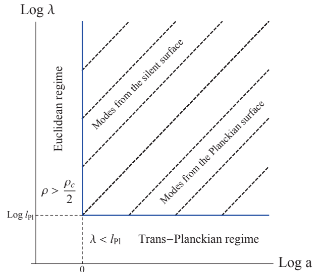
FIG. 6. The thick (blue) line represents the surface at which the initial conditions are imposed. For the modes with k < m_{\text{Pl}} at a = 1 this is the silent surface while for k > m_{\text{Pl}} it is the Planckian surface. The dashed lines represent the evolution of the different length scales \lambda = \frac{a}{k} . The wavelength \lambda = l_{\text{Pl}}a sets the limit between the different types of initial conditions.
