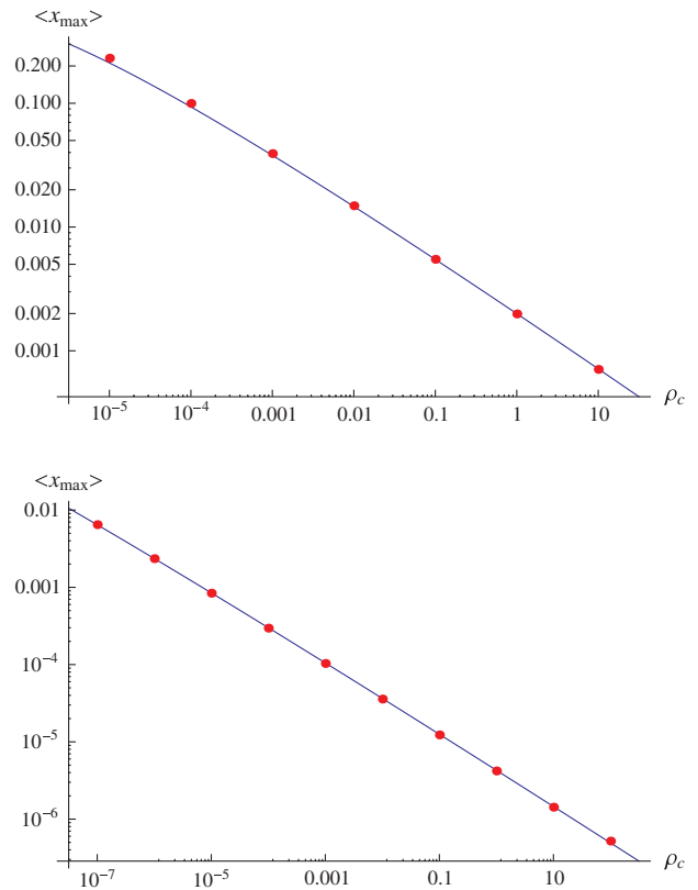
FIG. 4 (color online). Analytical approximation of x_{\max} as a function of \rho_c (blue line) and mean values of numerical simulations (red dots) for m = 10^{-3} (upper plot) and m = 1.21 \times 10^{-6} (lower plot).
