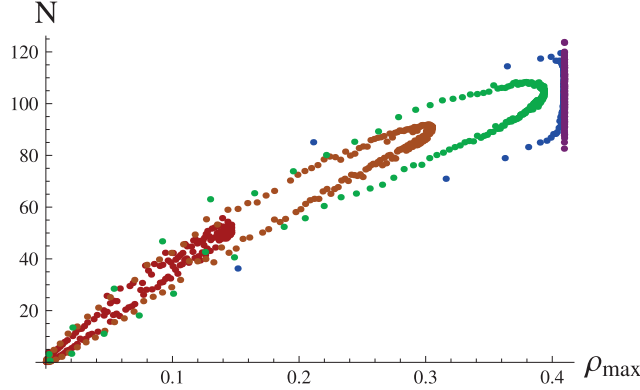
Figure 5. Number of e-folds as a function of \rho at the bounce. Red: \sigma_Q^2(0) = 10^{-\frac{2\kappa}{3}}\rho_0 . Orange: \sigma_Q^2(0) = 10^{-\frac{3\kappa}{3}}\rho_0 . Green: \sigma_Q^2(0) = 10^{-\frac{4\kappa}{3}}\rho_0 . Blue: \sigma_Q^2(0) = 10^{-\frac{6\kappa}{3}}\rho_0 . Purple: \sigma_Q^2(0) = 0 . Different points of the same color correspond to different values of delta.
