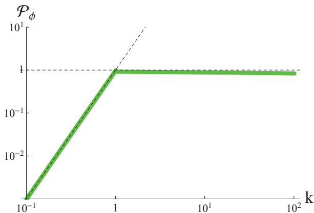
FIG. 7. Power spectrum at t = 10 t_{\text{Pl}} with w = -0.95 . The initial power spectrum was \mathcal{P}(k) = k^3 for k < 1 and \mathcal{P}(k) = 1 for the modes with k > 1 , imposed at the trans-Planckian surface, as depicted by the dashed lines. The slight red-tilt appears due to decrease of the Hubble factor in time.
