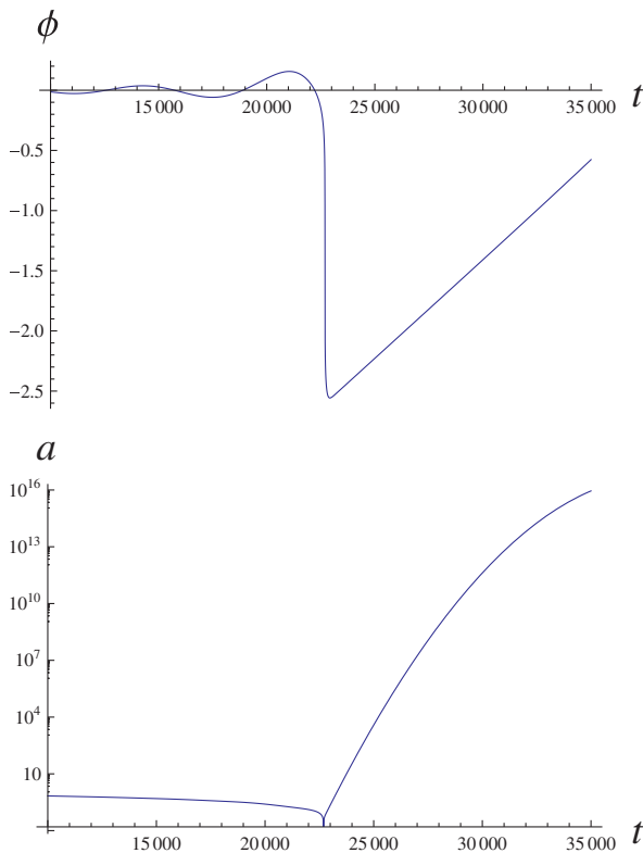
FIG. 2 (color online). Evolution of the scalar field (upper panel) and the scale factor (lower panel) as a function of cosmic time (the bounce corresponds to t = 22693 ). The parameters are m = 10^{-3}M_{\text{Pl}} and x_B = -1.5 \times 10^{-3} .
