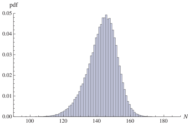
FIG. 3 (color online). Probability density of the number of e-folds of slow-roll inflation.
