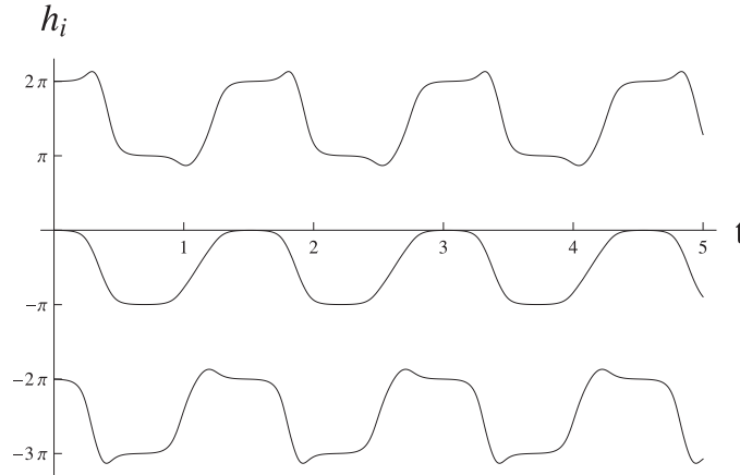
Figure 8. h_i as a function of time in a region without classical limit.
