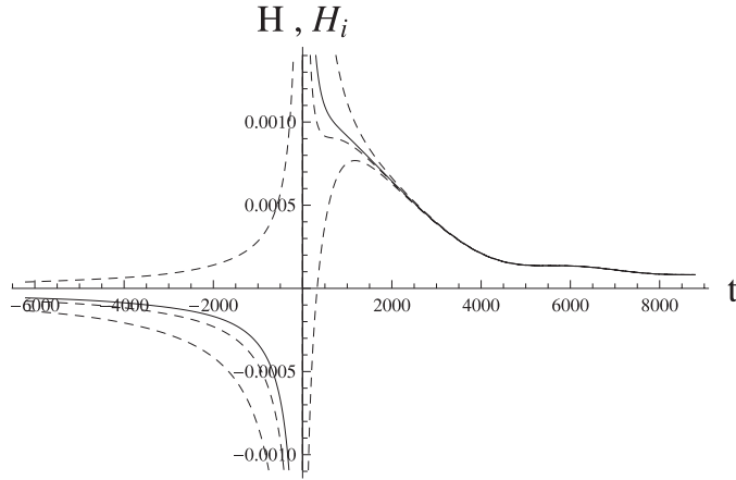
Figure 3. Zoom of figure 2 round the bounce. The full line is the total Hubble factor H and the tree dashed lines are the directional Hubble factors H_i , as a function of time.
