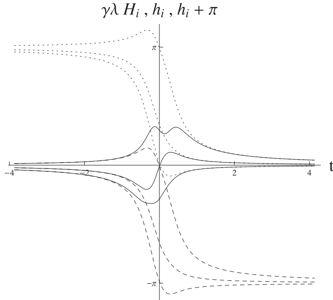
Figure 4. The full lines are \gamma\lambda H_i , the dashed lines are h_i and the dotted lines are h_i + \pi , as a function of time.
