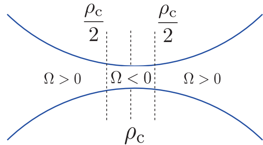
FIG. 1. Regions of the positive and negative values of the parameter \Omega in a typical symmetric cosmic bounce. The silent initial conditions investigated in this paper are imposed at \rho = \rho_c/2 .
