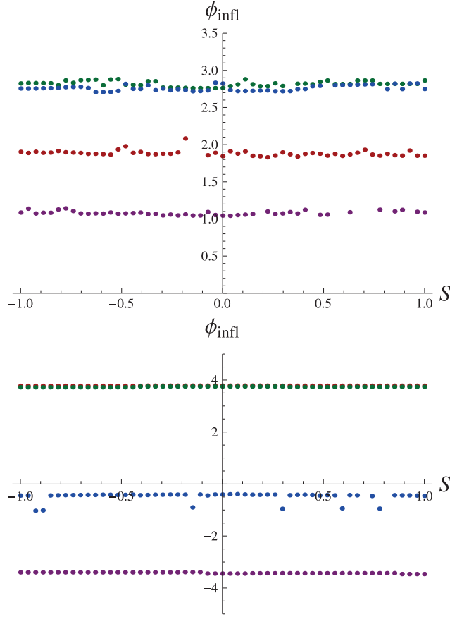
Figure 3. Scalar field at the beginning of inflation as a function of S . Upper: \sigma_Q^2(0) = 10^{-2\kappa/3}\rho_0 . Lower: \sigma_Q^2(0) = 10^{-3\kappa/3}\rho_0 . Red is \delta = 0 , green is \delta = \frac{\pi}{4} , blue is \delta = \frac{\pi}{2} and purple is \delta = \frac{3\pi}{4} . Note that in the lower plot, the green points are right on top of the red ones and are therefore hard to be seen.
