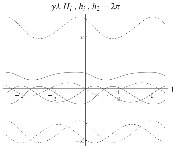
Figure 10. This solution is generated by taking the initial conditions at the bounce with the same values as the solution in figure 2–5 but adding 2\pi to h_2 . The full line are \gamma\lambda H_i , the dashed lines are h_i and the dotted line is h_2 - 2\pi .
