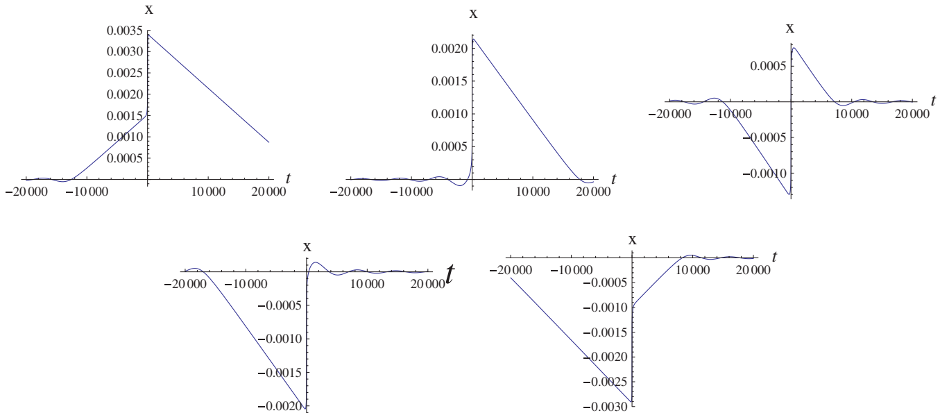
FIG. 1 (color online). Examples of evolutions of x as a function of time for different solutions. The linear increase (decrease) of |x| is the slow-roll deflation (inflation) phase, and the almost vertical increase or decrease of x is the superdeflation, bounce, and superinflation phase. A solution with no deflation at all like in the upper middle plot is by far the most probable. The mass of the scalar field used here is m = 10^{-3} , but the features remain true for any mass.
