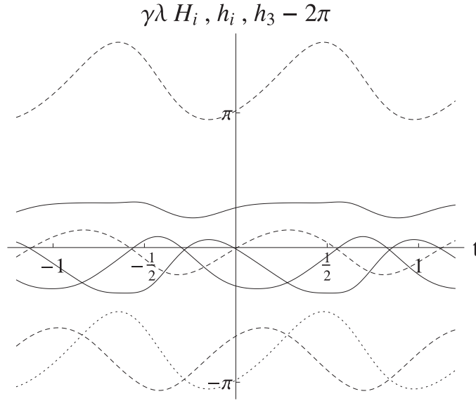
Figure 11. This solution is generated by taking the initial conditions at the bounce with the same values as the solution in figure 2–5 but adding 2\pi to h_3 . The full line are \gamma\lambda H_i , the dashed lines are h_i and the dotted line is h_3 - 2\pi .
