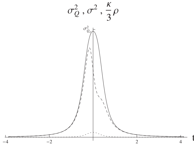
Figure 5. The full line is \sigma_Q^2 , the dashed line is \sigma^2 and the dotted line is \rho , as a function of time.
