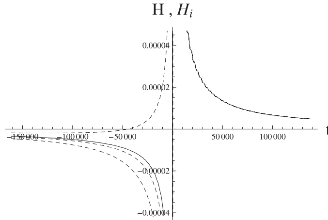
Figure 2. The full line is the total Hubble factor H and the three dashed lines are the directional Hubble factors H_i , as a function of time.
