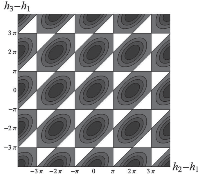
Figure 1. \sigma_Q^2 as a function of h_2 - h_1 ( x -axis) and h_3 - h_1 ( y -axis). The white areas correspond to \sigma_Q^2 > \sigma_{Qc}^2 , which is forbidden by the modified Friedman equation (24). The black lines are \sigma_Q^2 = \frac{1}{4}\sigma_{Qc}^2, \frac{1}{2}\sigma_{Qc}^2, \frac{3}{4}\sigma_{Qc}^2, \sigma_{Qc}^2 .
