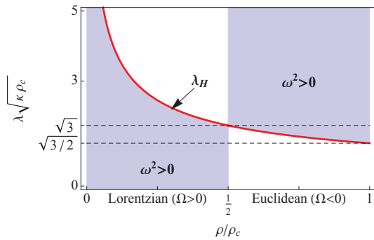
FIG. 4. The regions of \omega_k^2 > 0 for w = -1
