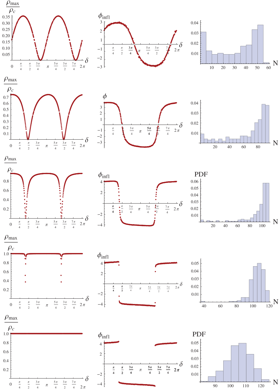
Figure 4. Results of the simulations, for each row, starting from the top \sigma_Q^2(0) = \{10^{-2\kappa/3}\rho_0, 10^{-3\kappa/3}\rho_0, 10^{-4\kappa/3}\rho_0, 10^{-6\kappa/3}\rho_0, 0\} . First column: the maximum value of \rho (which is the value of \rho at the bounce) normalized to \rho_c . Second column: \phi at the start of slow-roll inflation. Third column: numerically calculated probability distribution function of the number of e-folds of slow-roll inflation, given that all \delta have an equal probability.
