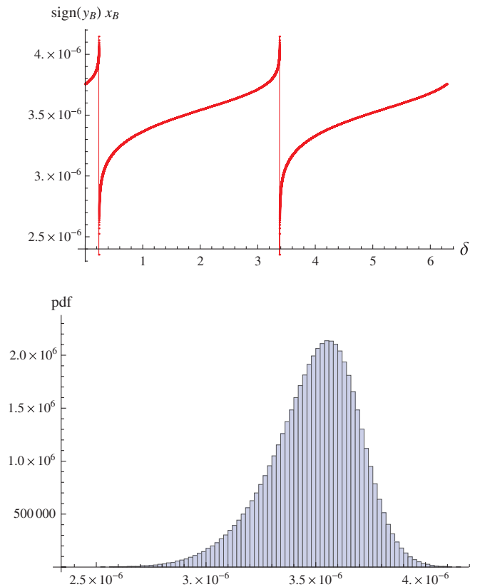
FIG. 2 (color online). \text{sign}(y_B)x_B as a function of \delta (upper plot) and its probability distribution (lower plot).
