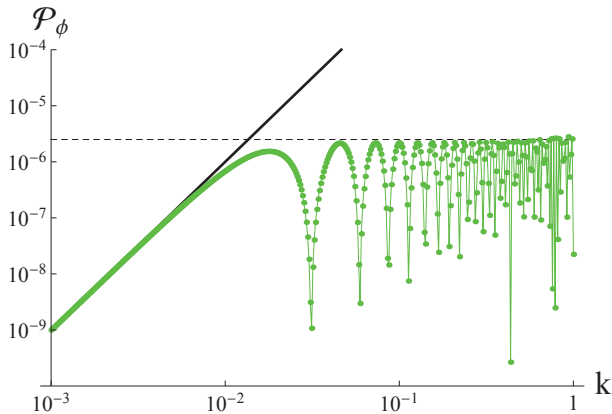
FIG. 8. Power spectrum converted to a rough scale invariance from the initial \mathcal{P}(k) = (k/m_{\text{Pl}})^3 . The spectrum was computed at t = 6000t_{\text{Pl}} with \frac{\Lambda}{8\pi G\rho_c} = 10^{-7} .
