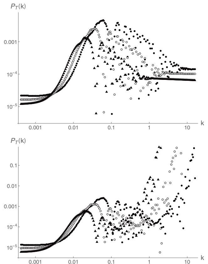
FIG. 2. Primordial power spectra for the tensor modes in the dressed metric approach (upper panel) and in the deformed algebra approach (lower panel) for different values of \rho_c . The mass of the scalar field is m = 10^{-3}m_{Pl} and \cos\theta_A \approx 1 . The critical energy density is \rho_c = 0.0041m_{Pl}^4 (triangles), \rho_c = 0.041m_{Pl}^4 (open disks) and \rho_c = 0.41m_{Pl}^4 (black disks).
