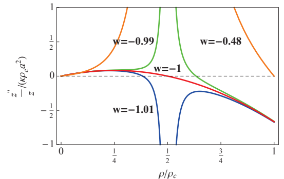
FIG. 3. The \frac{z''}{z} as a function of \rho/\rho_c for different values of w .
