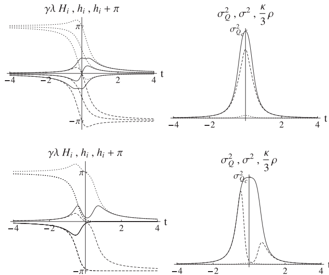
Figure 6. Upper: a solution with maximally symmetric anisotropy. Lower: a solution with maximally asymmetric anisotropy. Left: the full lines are \gamma\lambda H_i , the dashed lines are h_i and the dotted lines are h_i + \pi , as a function of time. Right: the full line is \sigma_Q^2 , the dashed line is \sigma^2 and the dotted line is \rho , as a function of time.
