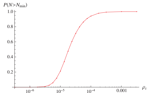
FIG. 5 (color online). Probability for having more than 65 e-folds of slow-roll inflation, P(N > 65) , as a function of \rho_c .
