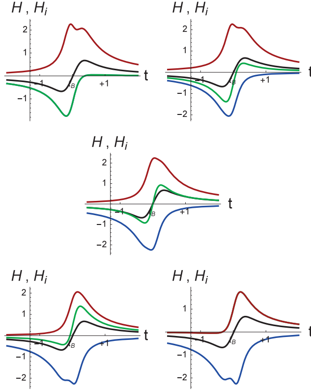
Figure 2. Details of the bounce shown for different values of the symmetry factor S . Upper left: S = -1 . Upper right: S = -0.5 . Center: S = 0 . Lower left: S = 0.5 . Lower right: S = 1 . Black is H , red is H_3 , green is H_2 and blue is H_1 . \sigma_Q^2(0) = 10^{-2\frac{k}{3}}\rho_0 and \delta = 0 for all the above plots. In the upper left plot, the blue line is hidden by the green one. In the lower right plot, the green line is hidden by the red one.
