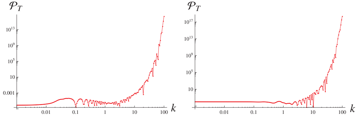
FIG. 4 (color online). Power spectrum of tensor perturbations after inflation for m = 10^{-3}M_{\text{Pl}} (left panel) and for m = 10^{-1}M_{\text{Pl}} (right panel).
