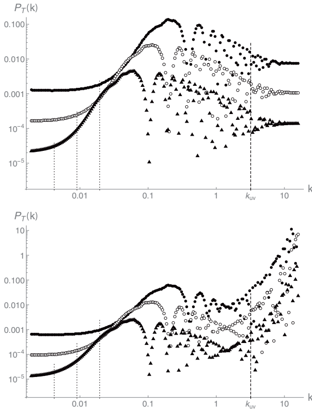
FIG. 1. Primordial power spectra for tensor modes in the dressed metric approach (upper panel) and in the deformed algebra approach (lower panel) for different values of the mass of the scalar field. The critical energy density is \rho_c = 0.41m_{\text{Pl}}^4 and \cos\theta_A \approx 1 . The mass of the scalar field takes three values: m = 10^{-3}m_{\text{Pl}} (triangles), m = 10^{-2.5}m_{\text{Pl}} (open disks), and m = 10^{-2}m_{\text{Pl}} (black disks). The dashed vertical line at large k , corresponds to k_{\text{UV}} (which does not depend on m ). The dotted vertical lines at smaller k correspond to k_{\text{IR}} (which scales as m^{2/3} ).
