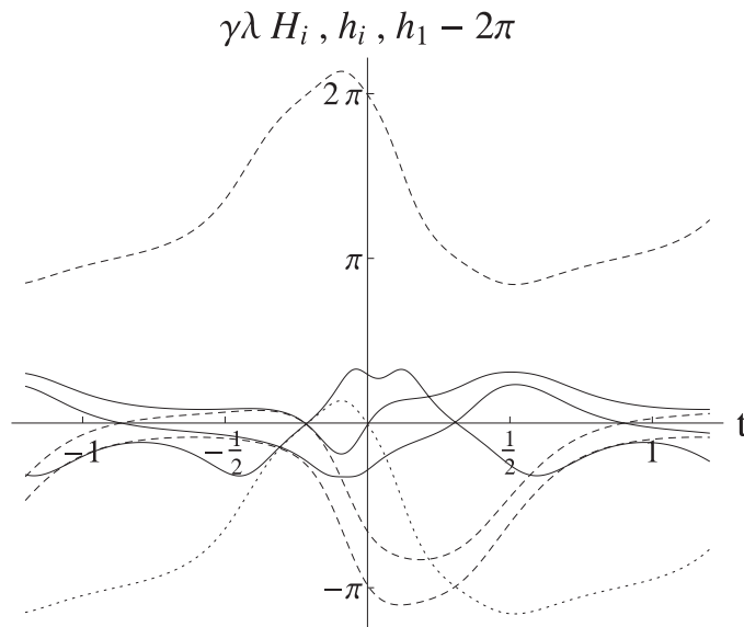
Figure 9. This solution is generated by taking the initial conditions at the bounce with the same values as the solution in figure 2–5 but adding 2\pi to h_1 . The full line are \gamma\lambda H_i , the dashed lines are h_i and the dotted line is h_1 - 2\pi .
