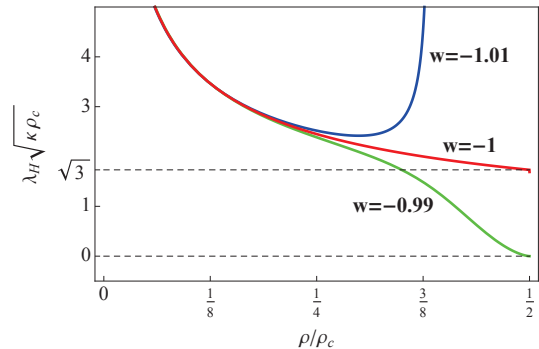
FIG. 2. Scale of the horizon \lambda_H as a function of \rho/\rho_c for different values of the barotropic index w . Only the Lorentzian domain ( \Omega > 0 ) is considered.
