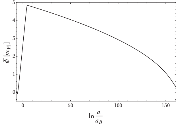
FIG. 1. Evolution of the scalar field as a function of the number of e -folds N := \pm \ln a/a_{\text{B}} , with m = 1.2 \times 10^{-6} m_{\text{Pl}} . The zero on the horizontal axis corresponds to the bounce when a_{\text{B}} = 1 . This solution is such that x_{\text{B}} = 3.55 \times 10^{-6} (obtained with \alpha = 17\pi/4 + 1 and \theta_0 = 5.11 ). The evolution is stopped at the end of inflation when \phi = 1/\sqrt{4\pi} m_{\text{Pl}} .
