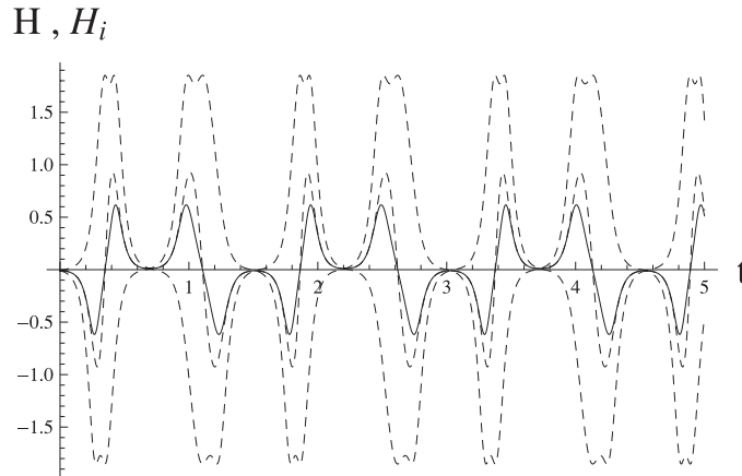
Figure 7. The full line is the total Hubble factor H and the three dashed lines are the directional Hubble factors H_i , as a function of time.
