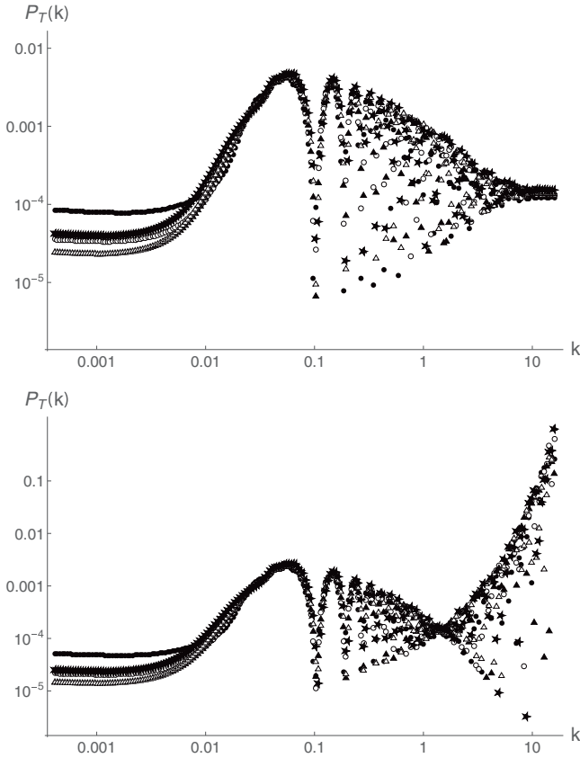
FIG. 3. Primordial power spectra for the tensor modes in the dressed metric approach (upper panel), and in the deformed algebra approach (lower panel). The parameter \theta_0 varies from (\pi/2 - 1) \simeq 0.18 \times \pi to (\pi/2 + 1) \simeq 0.81 \times \pi . The exact values are: plain disks for \theta_0 = (\pi/2 - 1) , open disks for \theta_0 = (\pi/2 - 1/2) , plain triangles for \theta_0 = \pi/2 , open triangles for \theta_0 = (\pi/2 + 1/2) , and plain stars for \theta_0 = (\pi/2 + 1) . The mass of the field is m = 10^{-3} m_{\text{Pl}} , and the critical energy density is \rho_c = 0.41 m_{\text{Pl}}^4 .
