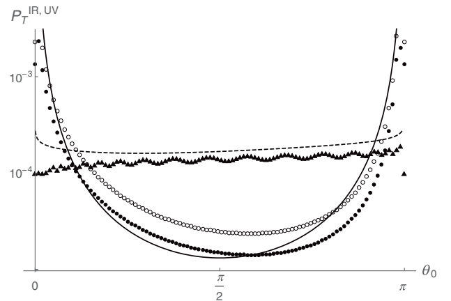
FIG. 4. The infrared limit (disks) and the ultraviolet limit (triangles) of the primordial power spectrum as a function of \theta_0 . The solid black curve corresponds to the analytical calculations for \mathcal{P}_T^{\text{IR}} , see (45). The IR limit from a numerical simulation is displayed with open disks for the dressed metric approach, and black disks in the deformed algebra approach. The dashed black curve stands for the analytical UV limit in the dressed metric approach, see (52a). The UV limit in the dressed metric approach, as derived from the numerics, corresponds to the black triangles. The mass of the scalar field is m = 10^{-3} m_{\text{Pl}} , and the critical energy density is \rho_c = 0.41 m_{\text{Pl}}^4 .
