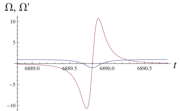
FIG. 1 (color online). Evolution of \Omega and its derivative with respect to conformal time. The density where \Omega vanishes is half the critical density, whereas \Omega' vanishes at the bounce.
