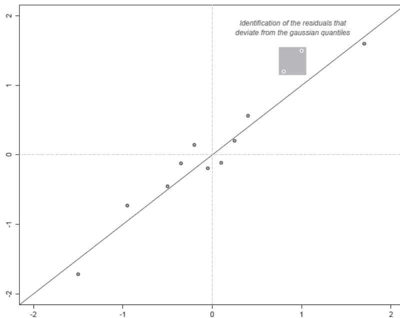
Figure 3.2 – Metamodel validation - QQ-plot true Gaussian quantiles vs. standardized residuals
