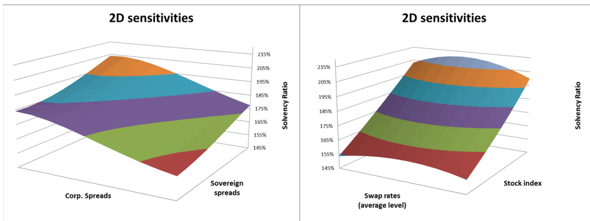
Figure 2.10 – 2D solvency ratio sensitivities.
