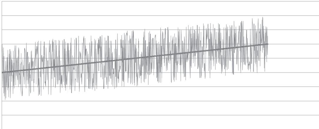
Figure 3.7 – Simplified scalar example - homoscedastic scheme (Own Funds in thick grey / NPV outcomes in thin grey)
