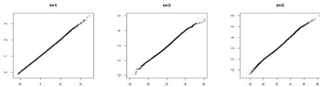
Figure 1.9 – QQ plots \widehat{SR}_t vs. ^{CF}SR_t
