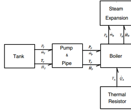
Fig. 2.10 Word Bond Graph of the system
