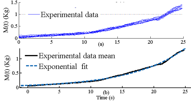
Fig. 3.22 Exponential variation of mass. (a) experimental data (b). Exponential fit over experimental data mean
