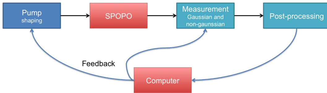
Figure 9.12: Squeezing of eigenmodes.
