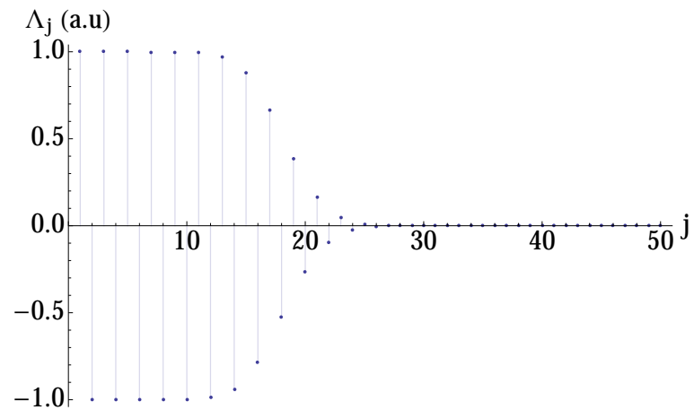
Figure 3.5: Eigenvalues of the joint spectral matrix with a 50nm bandwidth of mirror reflectivity .
