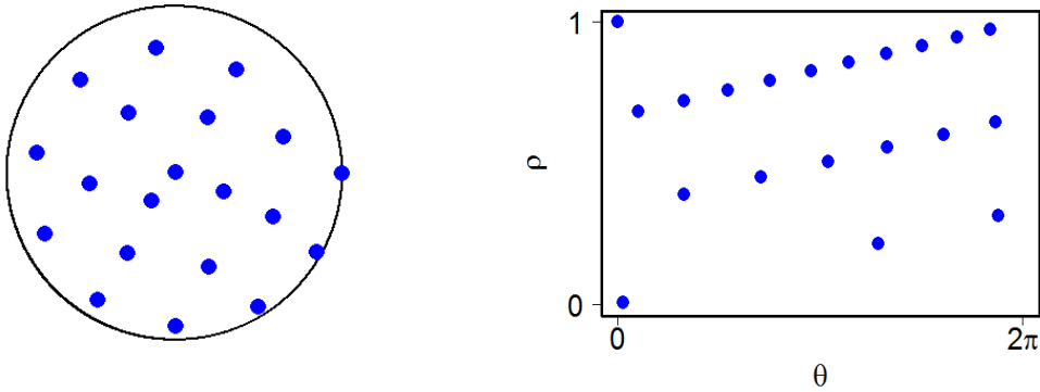
Figure 5.3 – Cartesian (left) and polar (right) representations of the Archimedean spiral DoE. This DoE is filling well the disk but not the cylinder of polar coordinates.
