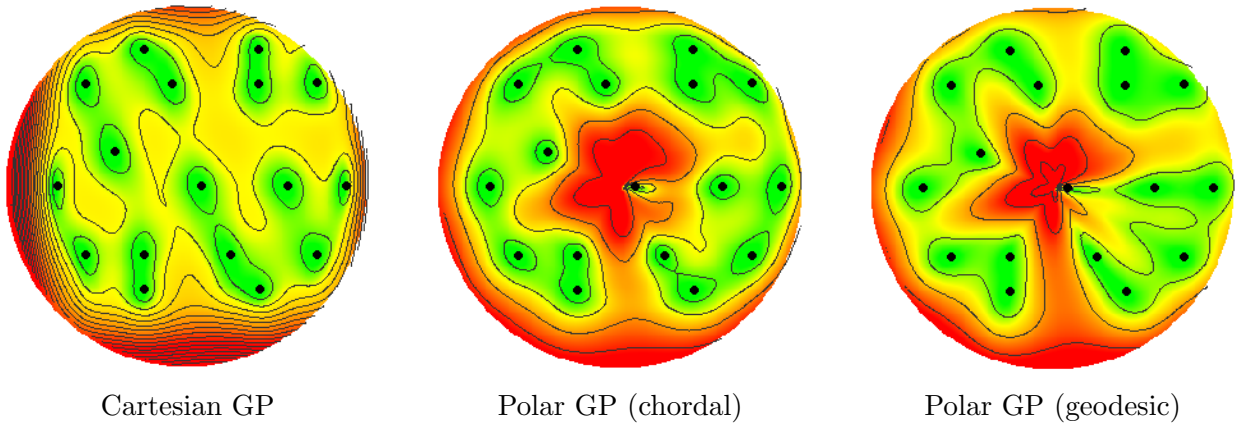
Figure 3.4 – Kriging standard deviations for Cartesian and polar GPs (kernels (a)-(c))
