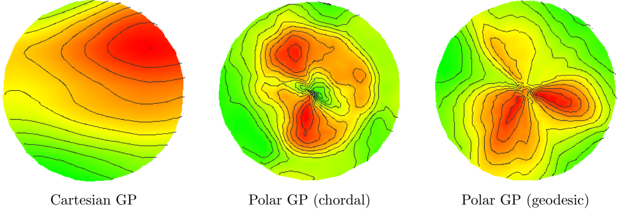
Figure 3.3 – Simulations of Cartesian and polar GPs with kernels (a)-(c).
