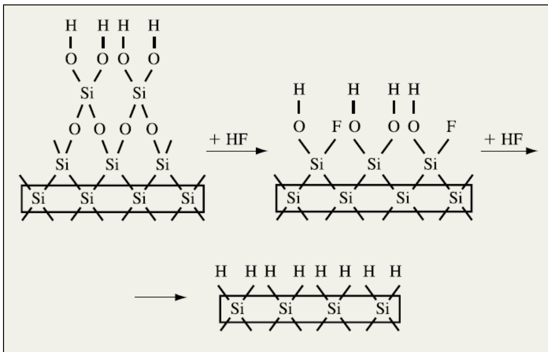
Figure 1-4: Schematic representation showing the changes of oxidized Si (100) wafer when immersed in HF solution [5], [6]
