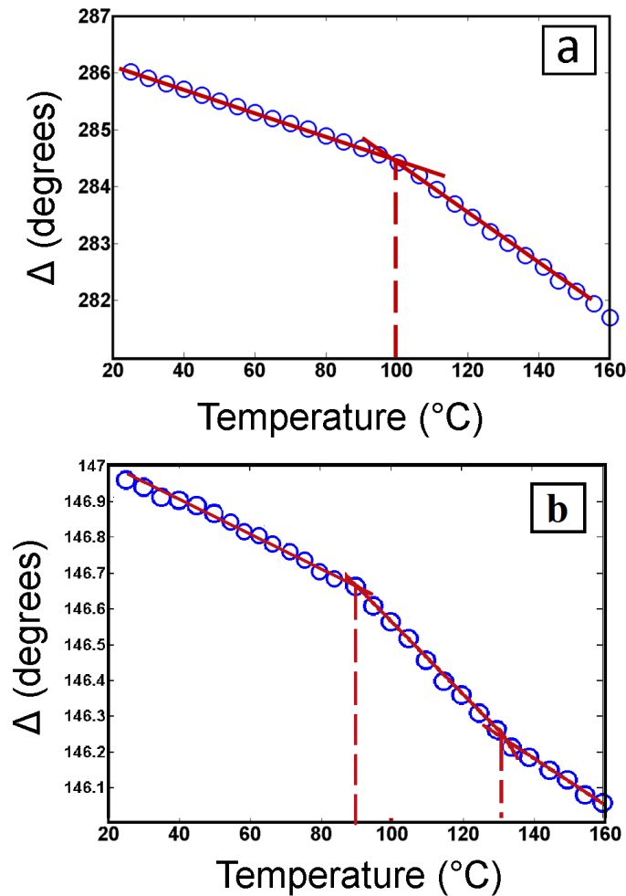
Figure 5-6. Raw ellipsometric curves showing \Delta as function of temperature for a) PS/H-Si (100 nm) measured at 2.75 eV b) PS/H-Si (~ 7.9 nm) after chloroform rinsing and post annealing.
