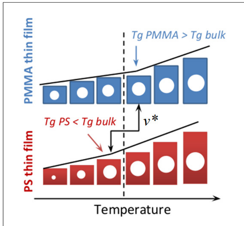
Figure 2-16: The schematic representation of the free volume that evolves with temperature, for PMMA and PS films. v^* stands for the critical volume.
