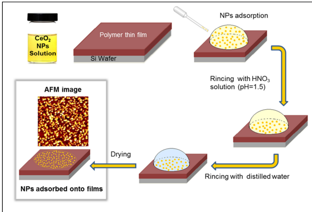
Figure 2-2. Schematic illustration of the ceria NPs adsorption process. The key parameters are the adsorption time, the refractive index of the polymer thin film and the NP dispersion, which allows tuning the surface coverage on samples of any shape and size.
