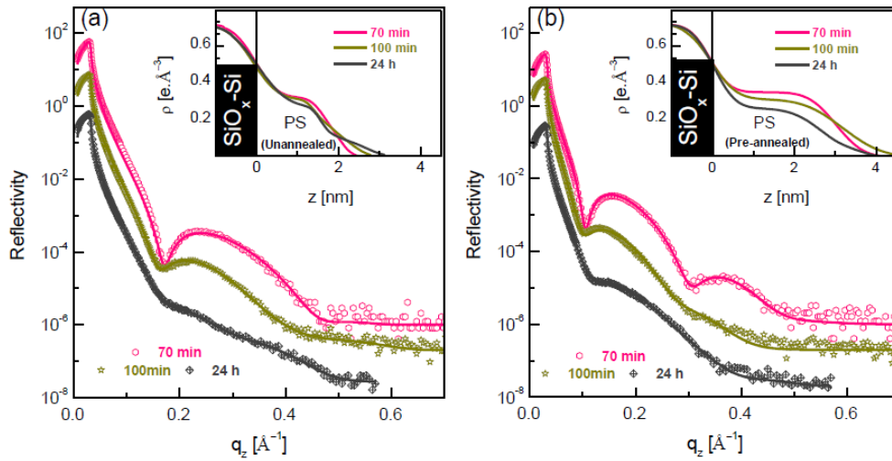
Figure 3-5: Solvent rinsing of a thick ( h_0 \approx 130 nm) PS film. XRR data (different symbols) and analyzed curves (solid line) of a thick PS film on a \text{SiO}_x\text{-Si} substrates before and after toluene rinsing during different durations as mentioned in the legend. Insets: corresponding EDPs showing different thicknesses of the PS films with different toluene rinsing times.
