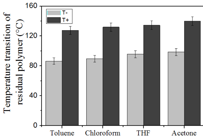
Figure 5-7. Temperature transition of PS/H-Si after rinsing with various solvents.
