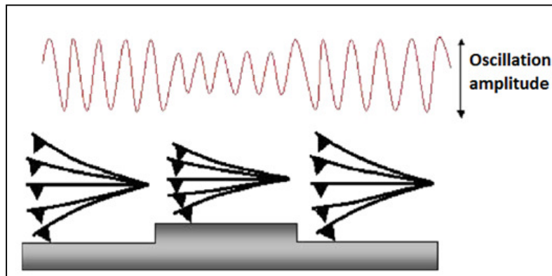
Figure 1-15: A schematic representation of AFM operating in tapping mode[20]
