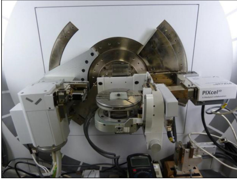
Figure 1-16: The photograph of Empyrean Panalytical reflectometer.
