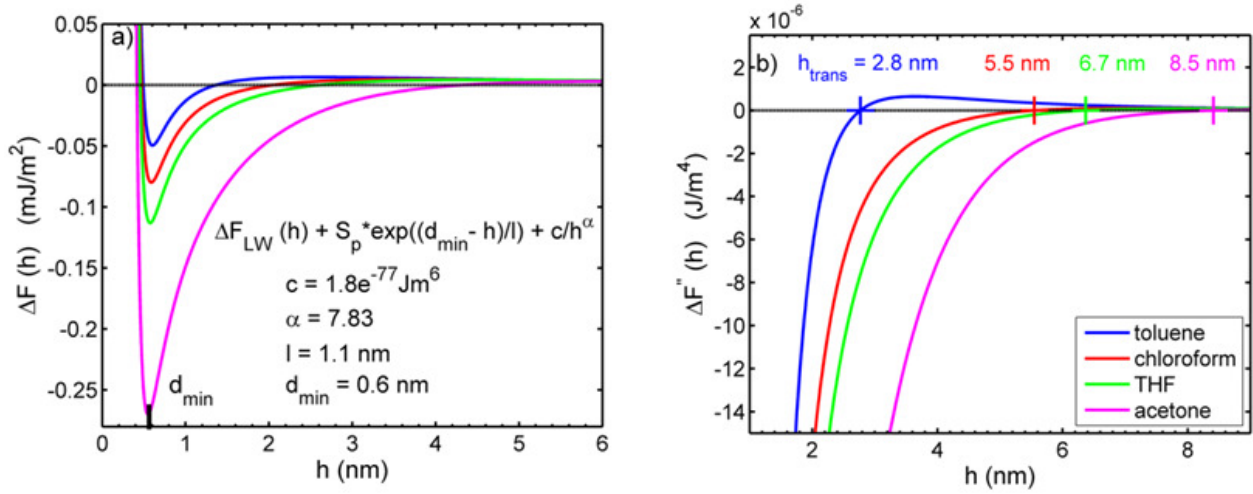
Figure 4-9: Simulation of (a) the effective free energy \Delta F and (b) its second derivative \Delta F'' as a function of PS film thickness h for a four layer Si/SiO x /PS/Solvent system. In these simulations, 4 solvents are considered: toluene, chloroform, THF and acetone. The effective free energy takes into account the effective contribution of the Lifshitz-van der Waals \Delta F_{LW} and of the polar \Delta F_P components as well as the steric repulsion energy c/h^\alpha .
