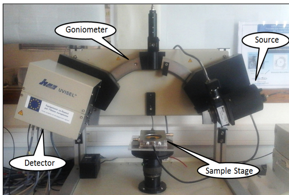
Figure 1-10: The photograph of Jobin-Yvon spectroscopic ellipsometer with labeled parts.
