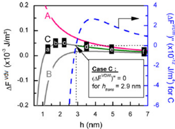
Figure 3-15: Simulated \Delta F^{VDW}(h) (solid lines) and [\Delta F^{VDW}(h)]'' (dashed line) curves using Eq.3-4 assuming 2 nm native oxides present on SiO_x -Si substrate. Curve 'A', drawn by choosing A_{Si/PS/Air} = -6.0 \times 10^{-20} J and A_{SiOx/PS/Air} = -0.2 \times 10^{-20} J , corresponds to a stable state. Curve 'B', deduced with A_{Si/PS/Air} = -4.4 \times 10^{-20} J and A_{SiOx/PS/Air} = 1.6 \times 10^{-20} J , depicts an unstable state. Curve 'C', plotted assuming A_{Si/PS/Air} = -5 \times 10^{-20} J and A_{SiOx/PS/Air} = 0.7 \times 10^{-20} J , corresponds to either a metastable state above h_{trans} \approx 2.9 nm and unstable films below h_{trans} . The letters a,b,c,d,e and f are corresponding to the AFM images presented in Figure 3-11. Color of state : stable in pink, unstable in grey, metastable in green.
