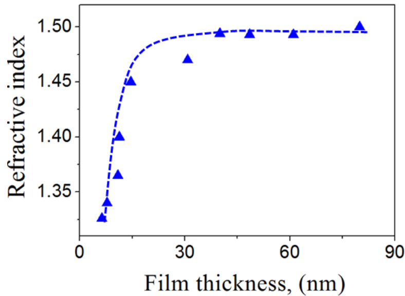
Figure 2-10: Refractive index of PMMA-SiO x -Si as a function of the PMMA film thickness.
