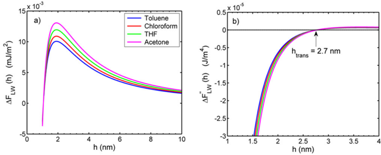
Figure 4-7: (a) Simulation of the Lifshitz-van der Waals component of the free energy \Delta F_{LW} and (b) its second derivative \Delta F''_{LW}(h) as a function of film thickness h for PS films for the four layer system Si/SiO_x/PS/Solvent under different solvent media. The effective Hamaker constants are the ones given in Table 4-3 and the thickness of the SiO_x layer was taken to be equal to 1.7 nm.
