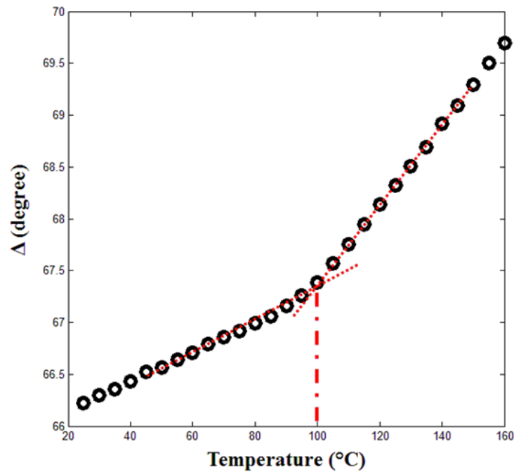
Figure 1-11: Raw ellipsometric curves showing \Delta as function of temperature for 100 nm PS film on Si wafer with native oxide.
