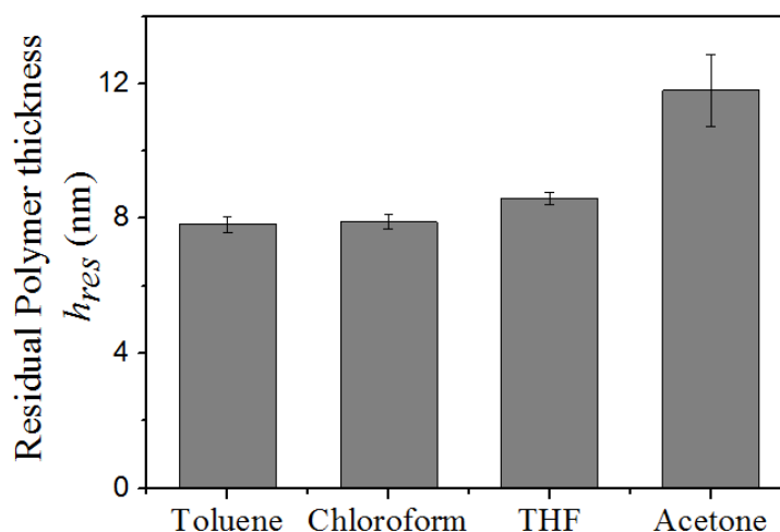
Figure 5-2. Residual thickness ( h_{res} ) of PS obtained by ellipsometry after rinsing with various solvents and post annealing (Acetone PS-HF is approximate value)
