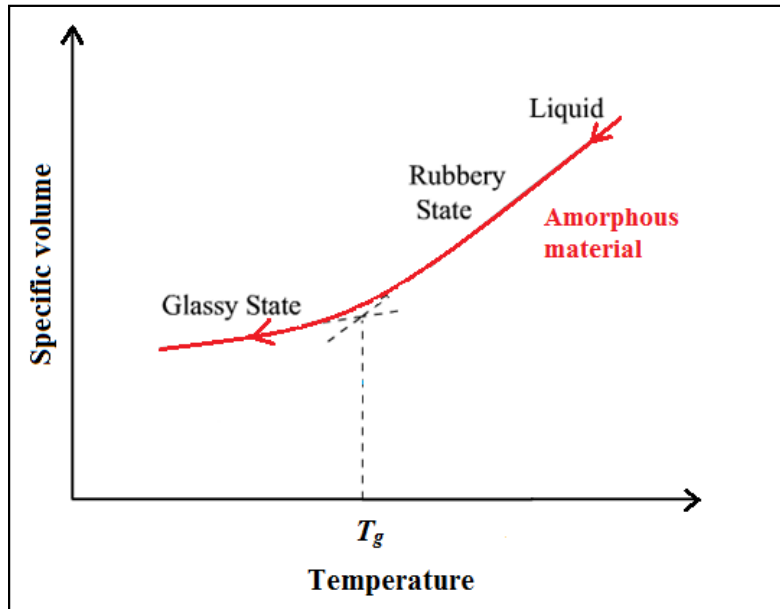
Figure 5-1: Schematic representation for the temperature transitions observed in an amorphous material
