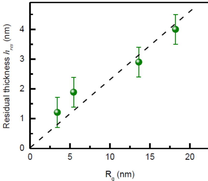
Figure 3-8: Residual layer thickness h_{res} as a function of R_g .
