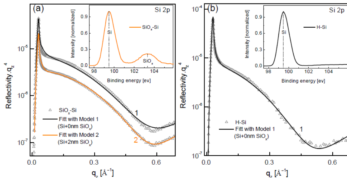
Figure 3-14: (a) Normalized XRR data (symbol) of RCA-cleaned Si and analyzed curves (solid lines). Inset: XPS spectrum of RCA-cleaned Si substrate demonstrating the existence of SiO x layer on top of Si. (b) Normalized XRR data (symbol) of HF-cleaned Si substrate and fitted curve (solid line) using model 1 without oxide layer. Inset: XPS spectrum confirming the absence of an oxide layer on H-Si substrate after HF-treatment.
