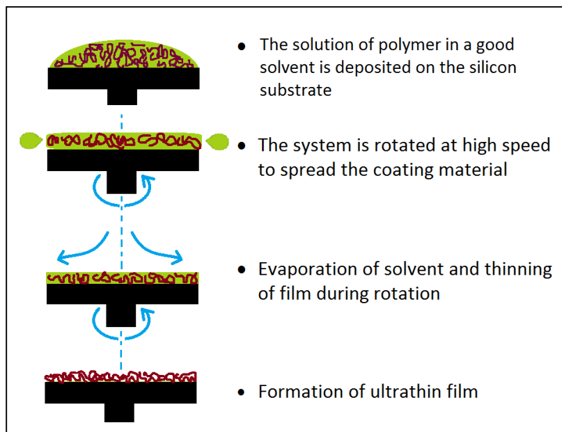
Figure 1-6: Schematic representation of the spin coating process. The substrate represented by black, solvent: green and the polymer: red respectively.
