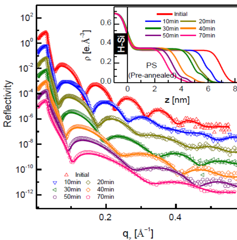
Figure 3-7: Solvent rinsing of a 7 nm preannealed PS film grown on a H-Si substrate. XRR data (different symbols) and analyzed curves (solid line) of a preannealed 7 nm PS film on a H-Si substrates before and after toluene rinsing during different durations as mentioned in the legend (curves are shifted vertically for clarity). Insets: corresponding EDPs showing different thicknesses of the PS films with different toluene rinsing times.
