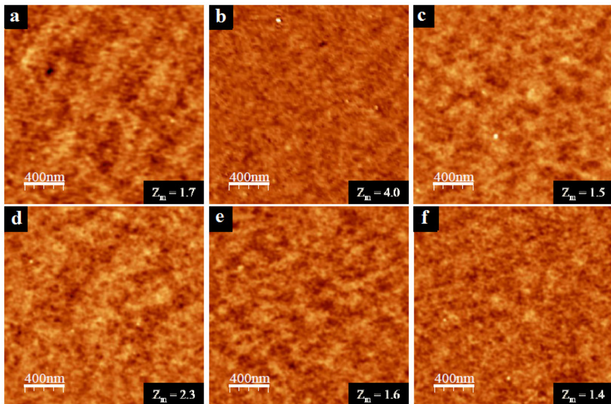
Figure 3-17: AFM topographic images (Scan size = 2 \times 2 \mu\text{m}^2 ) show the morphologies of residual films of thicknesses h_{\text{res}} (a) \approx 1.5 nm, (b) \approx 2.5 nm, (c) \approx 4.0 nm, (d) \approx 4.6 nm, (e) \approx 5.0 nm and (f) \approx 6.0 nm on H-Si substrates without post annealing. Z_m represents the maximum height in nm.
