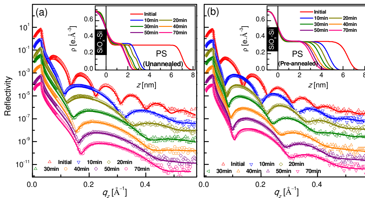
Figure 3-4: Structural evolution as a result of solvent rinsing. XRR data (different symbols) and analyzed curves (solid line) of unannealed (a) and pre-annealed (b) 7 nm PS films on SiO x -Si substrates before and after toluene rinsing during different durations (curves are shifted vertically for clarity). Insets: corresponding EDPs showing different thicknesses of the PS films with different toluene rinsing time.
