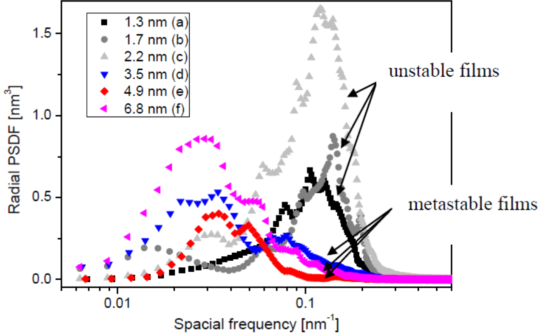
Figure 3-13: Power spectral density (PSD) curves of residual PS films grown on \text{SiO}_x -Si substrates having different thicknesses calculated from AFM images presented in Figure 3-11. B.
