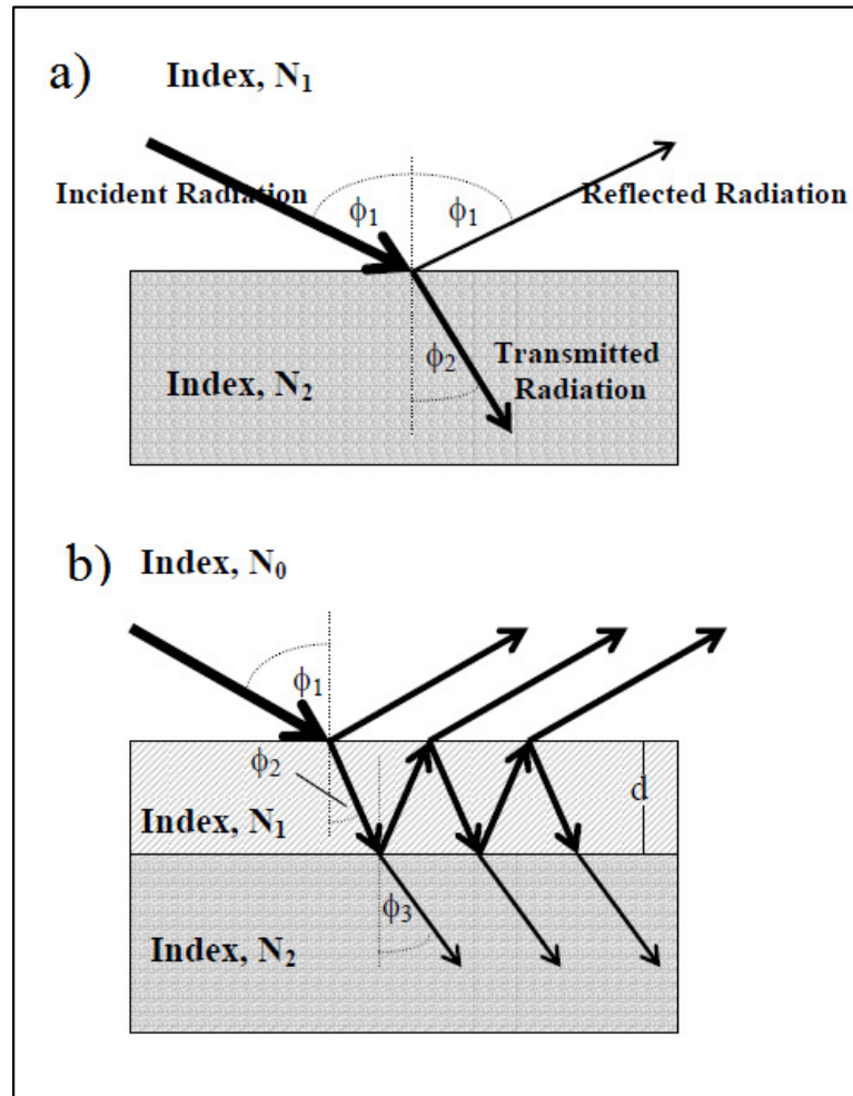
Figure 1-9: a.) Radiation interacting with a single plane parallel interface between Material 1, with refractive index N_1 , and Material 2, with refractive index N_2 . b.) Diagram of the beam path in a sample comprised of a film, with thickness d and refractive index N_1 , between Material 0, with refractive index N_0 , and Material 2, with refractive index N_2 . [17]
