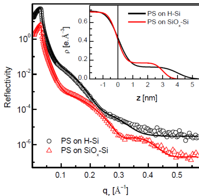
Figure 3-3: XRR and EDP profiles showing dewetting of directly spin-coated ultrathin films. XRR data (different symbols) and analyzed curves (solid line) of as-prepared PS films on H-Si and SiO x -Si substrates by direct spin-coating of 0.75 g/L solution (curves are shifted vertically for clarity). Insets: corresponding EDPs showing very low coverage of the PS films with respect to the bulk electron density \approx 0.344 e \cdot \text{\AA}^{-3} .
