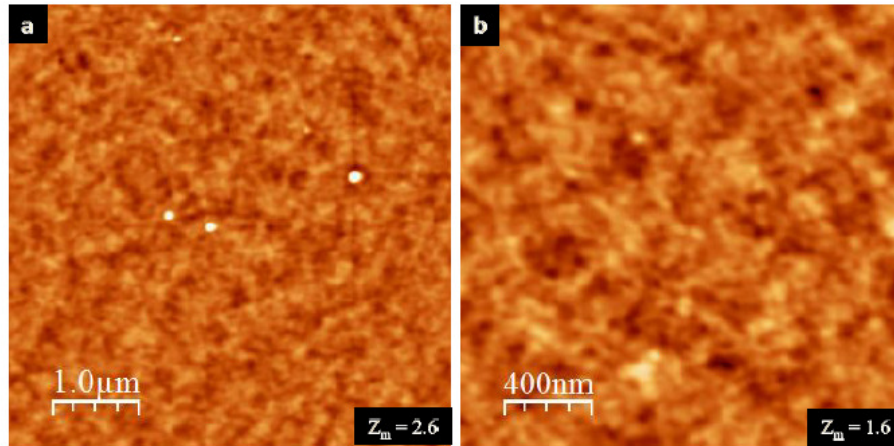
Figure 3-12: AFM topography images illustrate a 2.3 nm thick PS film (residual) on an oxide-free Si substrate. (a) Scan size = 5 \times 5 \mu\text{m}^2 (RMS roughness \approx 0.16 \text{ nm} ) and (b) Scan size = 2 \times 2 \mu\text{m}^2 (RMS roughness \approx 0.16 \text{ nm} ). The images were taken after post annealing at 170^\circ\text{C} during 24 h.
