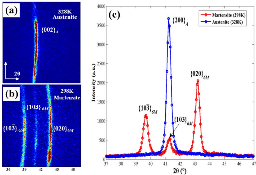
Fig. 6. 4 Neutron diffraction images of austenite (a) and martensite (b) at 2\theta from 35^\circ to 50^\circ . Their corresponding diffraction patterns against 2\theta ( 37^\circ to 47^\circ ) in intensity profiles are displayed in (c).
