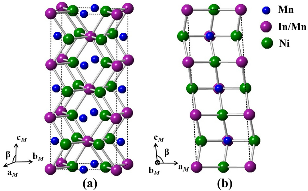
Fig. 3. 13 Schematic illustration of 3-dimensional superstructure with three consecutive unit cells.
