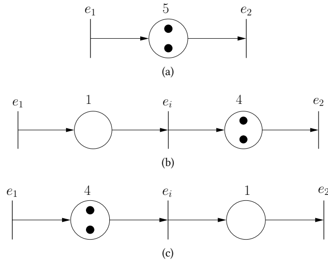
Figure B.1.: Equivalent synchronizations if no other synchronizations affect event e_i
