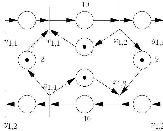
Figure 7.2.: Petri net representation of the train line
