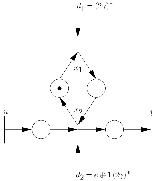
Figure 7.4.: Petri net representation of a (\max, +) -system subject to partial synchronization exhibiting impulse responses with different throughputs
