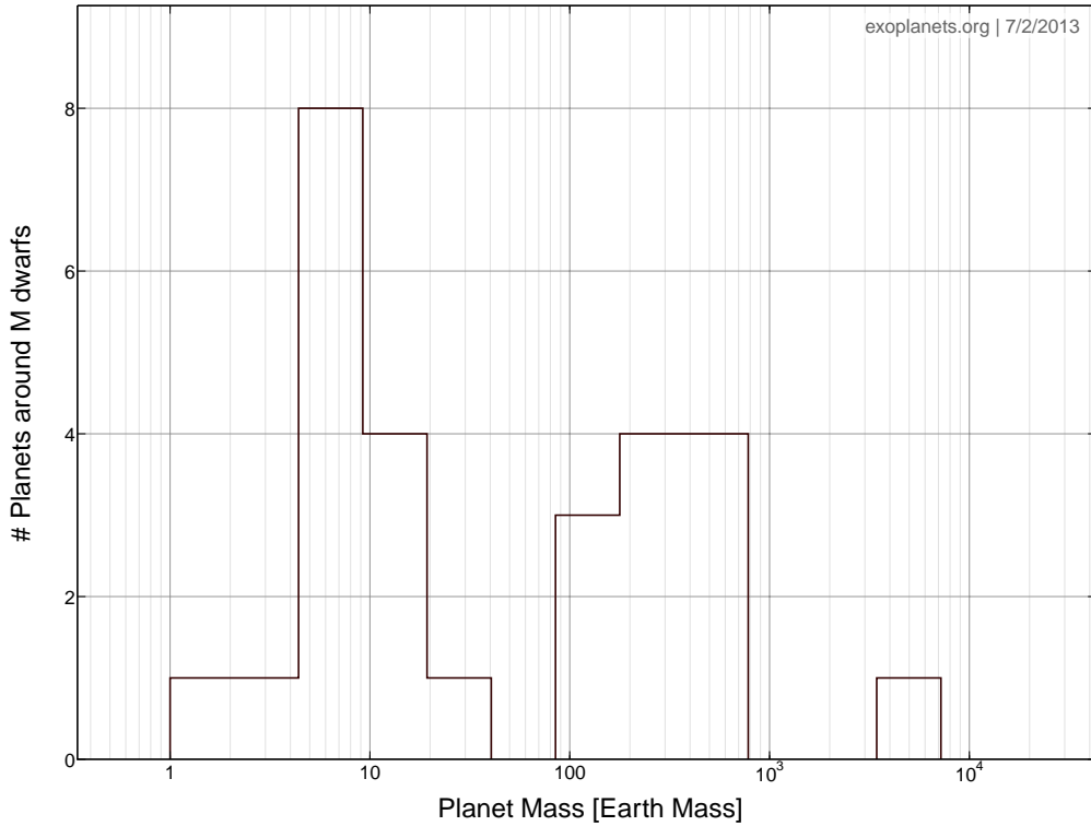
Figure B.4: Mass distribution of exoplanets detected by transit and RV surveys around M dwarfs. Plot made using exoplanets.org (Wright et al. 2012).
