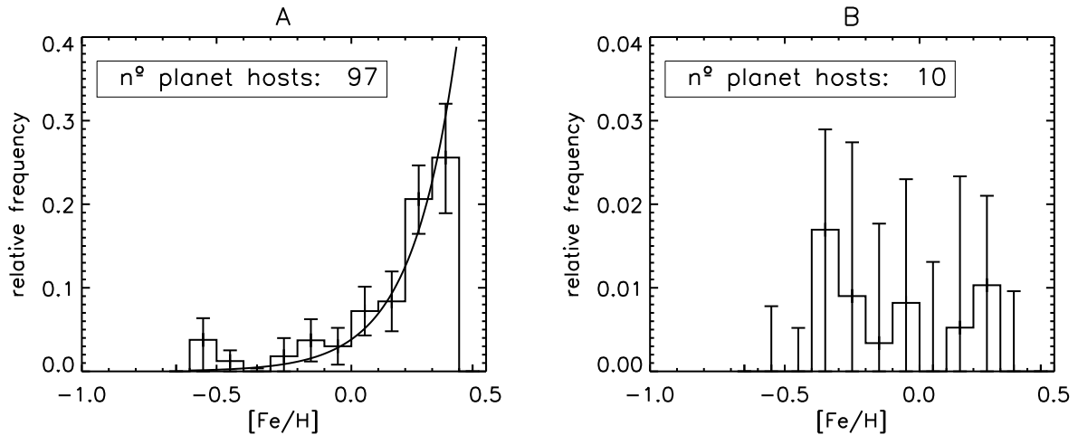
Figure 1.10: Frequency of planet-hosts as a function of [Fe/H] for the all planet hosts ( left panel ), and for planet-hosts with only Neptunian planets ( right panel ), of the volume-limited 582 FGK HARPS star sample (Sousa et al. 2011).
