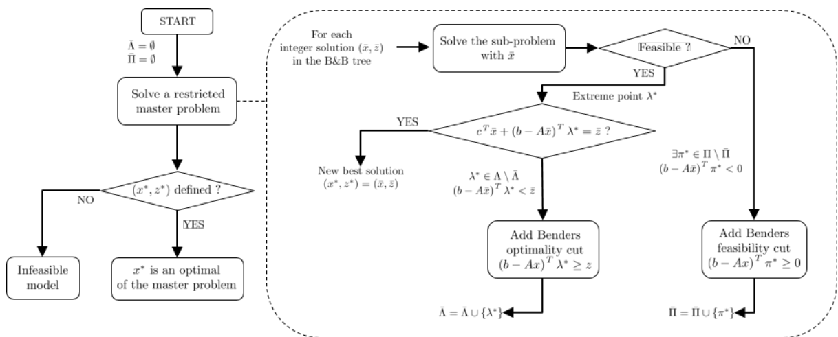
Figure 2.2 – Scheme of the alternative implementation of Benders decomposition
