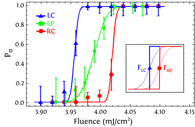
FIGURE 1.9: Switching probability P_{\sigma} as a function of the fluence at \lambda = 700 nm for three different polarizations. The measurements with RC and LC pulses were performed at a different time than the ones with LP pulses, and therefore the laser stability \epsilon was different. Shown in the inset are the switching probabilities in case of zero (solid) and nonzero (dashed) laser fluctuations. F_{LC} and F_{RC} denote the switching threshold of GdFeCo for LC and RC excitation pulses, respectively. Figure is adapted from [39].
