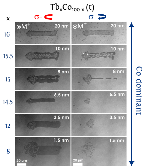
FIGURE 3.10: Optical response for \text{Tb}_x\text{Co}_{100-x} (t) alloy films for Tb concentration x ranging from 8 to 16 and alloy thickness varying from 1.5 nm to 20 nm. For each sample, right- and left-circularly polarized laser beam were swept over the sample from right to left. The initial magnetization saturation up is exemplarily shown. The dark contrast corresponds to a reversal to down. The laser power is ranging from 1.15 mW (for t < 8 nm) to 1.5 mW (for t > 8 nm).
