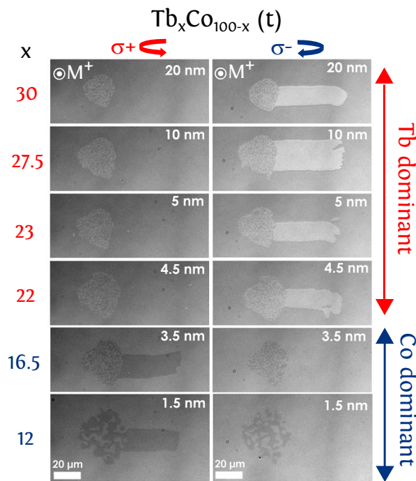
FIGURE 3.9: Optical response for Tb_xCo_{100-x} ( t ) alloy films for Tb concentration x ranging from 12 to 30 and alloy thickness varying from 1.5 nm to 20 nm. For each sample, right- and left-circularly polarized laser beam were swept over the sample from right to left. The initial magnetization saturation up is exemplarily shown. The white contrast for an alloy thickness varying from 20 nm to 4.5 nm, and the dark contrast for an alloy thickness 3.5 nm and 1.5 nm correspond to a reversal to down.
