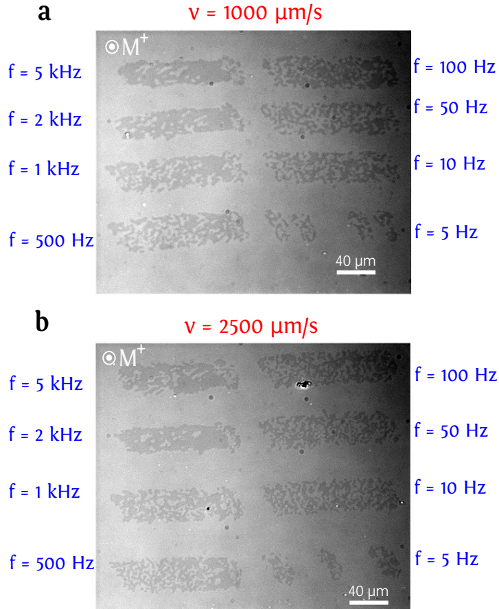
FIGURE 4.9: (a) and (b) Magneto-optical response of Pt(3.7 nm)/Co(0.6 nm)/Pt(3.7 nm) continuous film to right-circularly polarized laser beam swept from left to right at sweeping speeds of 1000 \mu\text{m/s} and 2500 \mu\text{m/s} , respectively. The used laser power is 0.7 \text{ mW} and the repetition rate is varied from 5 \text{ kHz} to 5 \text{ Hz} . The initial up magnetization saturation is exemplarily shown and the dark contrast corresponds to a reversal to down.
