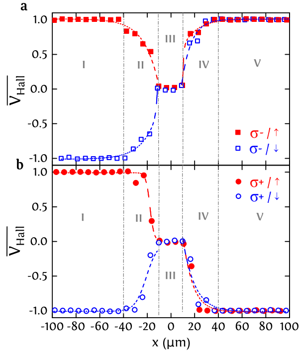
FIGURE 4.5: Normalized Hall voltage \overline{V}_{Hall} as a function of the position of the beam x swept where (a) corresponds to left-handed circular polarization ( \sigma^- ) and (b) to right-handed circular polarization ( \sigma^+ ). The values 1 and -1 of the \overline{V}_{Hall} correspond to both saturated magnetic states. The laser beam is swept over the whole x axis of Hall cross from position -100 \mu\text{m} to 100 \mu\text{m} , with a sweeping speed of 40 \mu\text{m/s} and a power of 0.95 mW. The experiment is repeated for both positive and negative saturation of the magnetization. The dashed lines are guides to the eyes.
