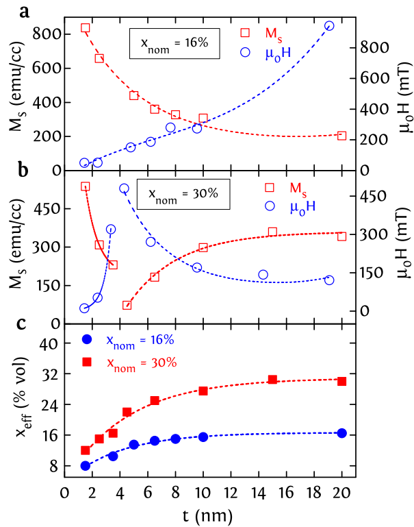
FIGURE 3.8: (a) (resp. (b)) Saturation magnetization and coercive field of TbCo alloy films for nominal Tb concentration x_{nom} of 16 at.% (resp. 30 at.%). (c) Effective concentration of Tb x_{eff} as a function of the thickness of TbCo alloy films with nominal Tb concentrations x_{nom} of 16 and 30. The dashed lines are guide to the eyes.
