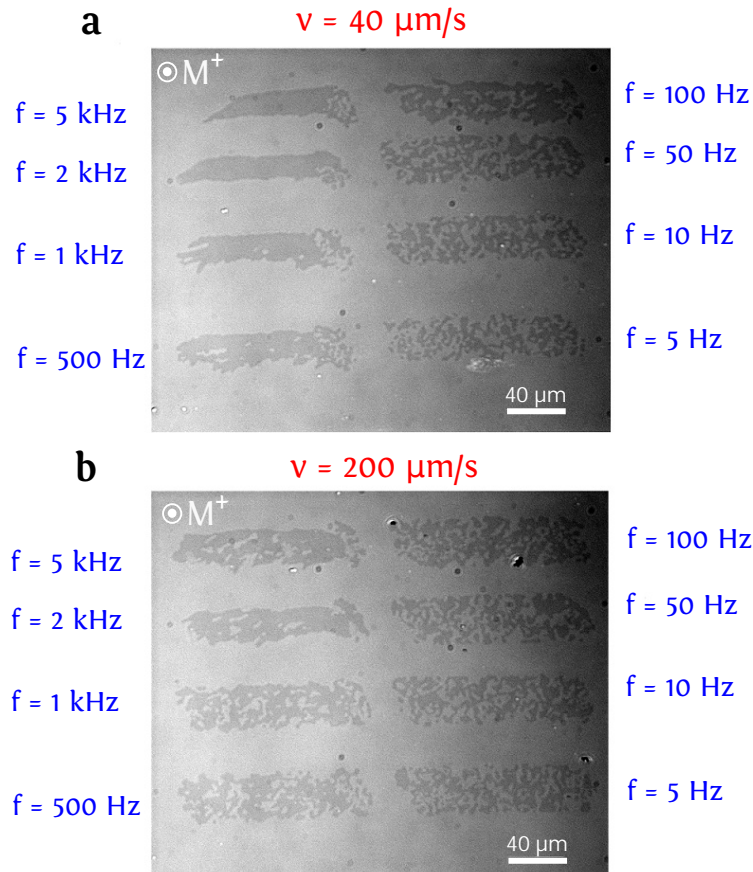
FIGURE 4.8: (a) and (b) Magneto-optical response of Pt(3.7 nm)/Co(0.6 nm)/Pt(3.7 nm) continuous film to right-circularly polarized laser beam swept from left to right a sweeping speeds of 40 \mu\text{m/s} and 200 \mu\text{m/s} , respectively. The laser power is 0.7 \text{ mW} and the repetition rate is varied from 5 \text{ kHz} to 5 \text{ Hz} . The initial up magnetization saturation is exemplarily shown and the dark contrast corresponds to a reversal to down.
