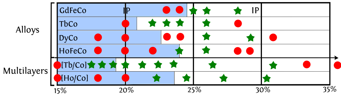
FIGURE 1.12: Response to optical excitation for RE-TM alloys ( \text{Gd}_x\text{FeCo}_{1-x} , \text{Tb}_x\text{Co}_{1-x} , \text{Dy}_x\text{Co}_{1-x} , \text{Ho}_x\text{FeCo}_{1-x} ) and two types of RE-TM multilayer ( [\text{Tb}/\text{Co}] and [\text{Ho}/\text{Co}] ) as a function of the RE concentration ( x ). Red dots indicate thermal demagnetization and green stars AO-HDS. All of these alloys show perpendicular anisotropy except the two \text{GdFeCo} alloys marked IP (for in-plane anisotropy). The regions shaded correspond to alloy compositions for which T_{\text{Mcomp}} is below RT. For the multilayers the RE layer thicknesses varied from 0.3 to 0.5 nm and the TM layers varied from 0.25 to 1.0 nm. Figure adapted from [43].
