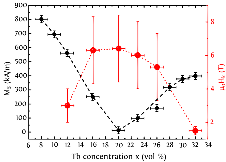
FIGURE 2.4: Magnetic properties of the Tb_xCo_{100-x} samples. Saturation magnetization M_s (black circles) and anisotropy field H_k (red circles) for the different Tb_xCo_{100-x} samples. The dashed and dotted lines are interpolations between the measured points. Large error bars are due to the uncertainty of magnetometry measurements for thin film samples with small magnetization. Figure adapted from [11].
