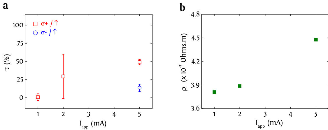
FIGURE 4.16: (a) Switching ratio as a function of the applied current intensity for sweeping beam measurements performed in a 7 \mu\text{m} -wide Pt/Co/Pt Hall cross with a speed of 40 \mu\text{m/s} and a laser power 0.4 mW. The initial up magnetization saturation is exemplarily shown. (b) Resistivity of Ta/Pt/Co/Pt as a function of the applied current intensity. No laser beam is applied during the resistivity measurement.
