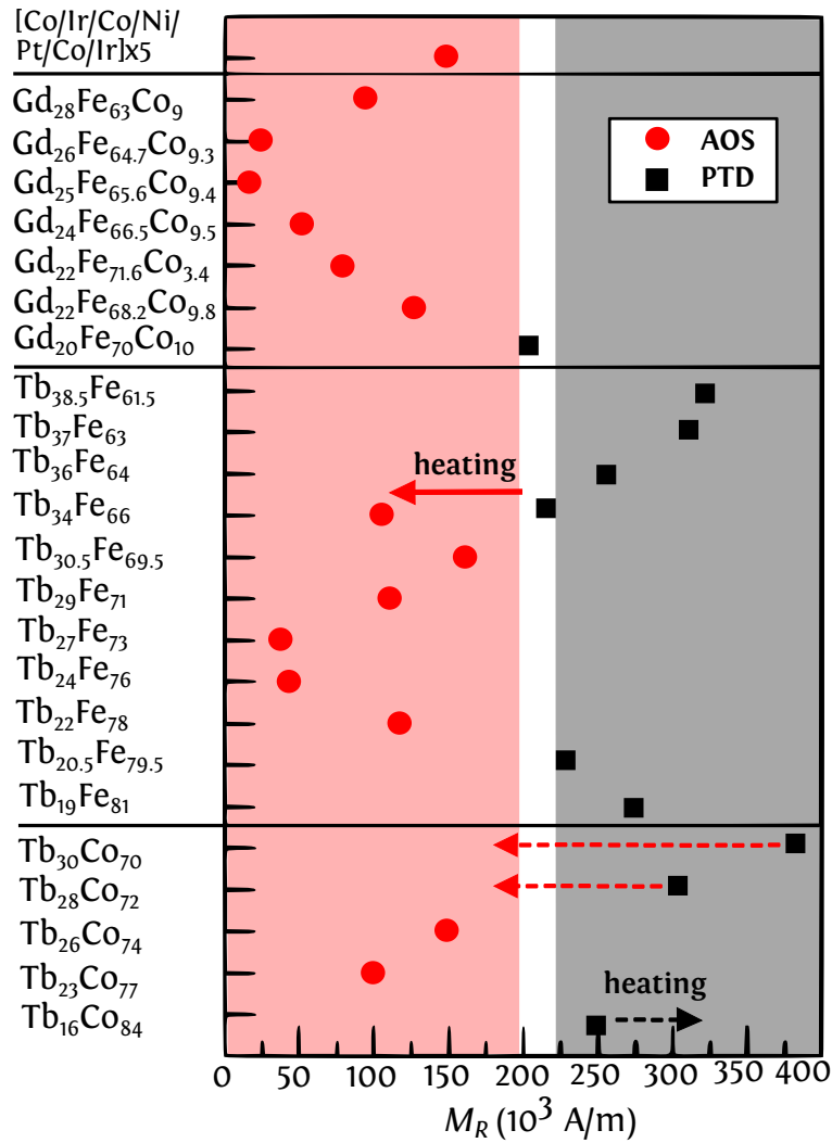
FIGURE 1.23: Overview of all-optical switching (AOS) in \text{Gd}_x\text{Fe}_{100-x-y}\text{Co}_y , \text{Tb}_x\text{Fe}_{100-x} , \text{Tb}_x\text{Co}_{100-x} , and [\text{Co/Ir/Co/Ni/Pt/Co/Ir}]_5 . Red dots and light-red area indicate AOS. Black squares and light-gray area denote pure thermal demagnetization (PTD). Red (black) arrows represent the decrease (increase) of sample magnetization due to heating; the solid red arrow shows our result obtained in \text{Tb}_{34}\text{Fe}_{66} . The dashed red and black arrows visualize the trend in \text{Tb}_x\text{Co}_{100-x} . Figure adapted from [44].
