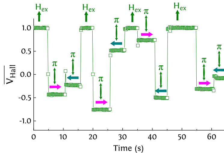
FIGURE 4.10: Time evolution of the normalized Hall voltage \overline{V_{\text{Hall}}} for the sweeping beam measurement repeated four times, with linear polarization sweeping and initial saturation up. The laser spot is swept back (dark cyan arrow) and forth (magenta arrow) over the whole x axis of the Hall cross, with a sweeping speed of 1000 \mu\text{m/s} and a power of 0.95 \text{ mW} , leading on average to a random switching ratio.
