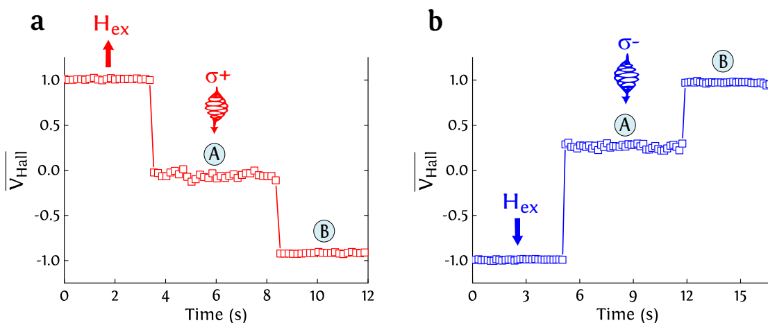
FIGURE 4.26: (a) (resp. (b)) Time evolution of the normalized Hall voltage while performing static beam measurement on the studied CoFeB/MgO based Hall cross with an initial saturation up (resp. down) and \sigma^+ (resp. \sigma^- ) polarization. The laser beam is well centered and turned on in “A”, whereas it is turned off in “B”.
