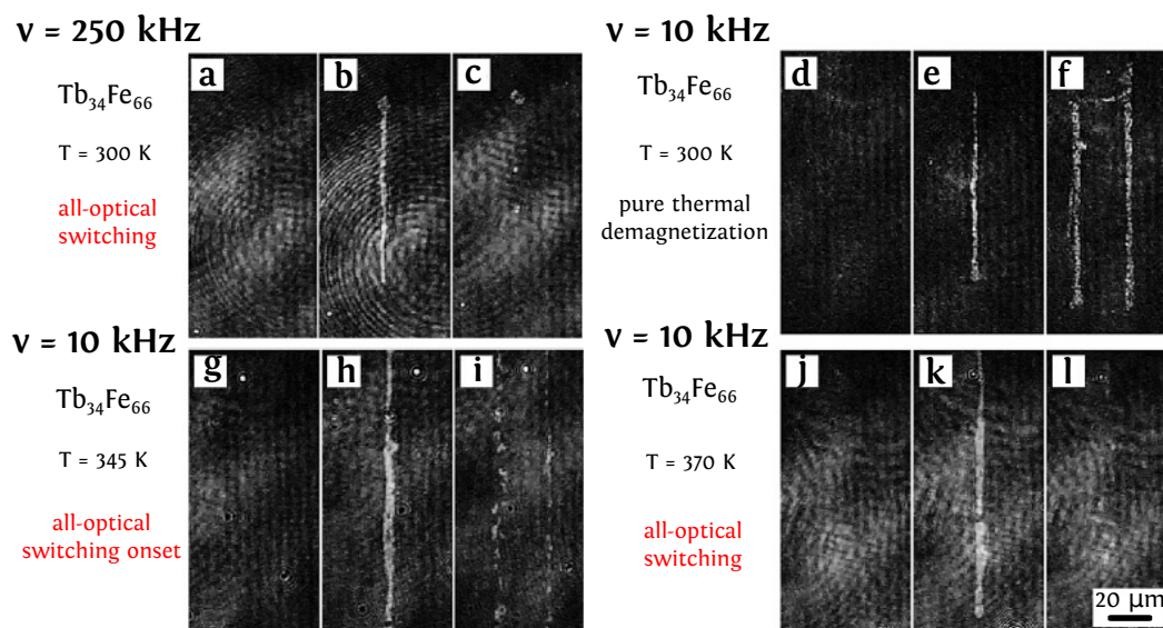
FIGURE 1.17: AO-HDS in Tb_{34}Fe_{66} at a pulse repetition rate of 250 kHz or 10 kHz. The left column shows the initial homogeneously magnetized state, the middle column after exposure with right-handed circularly polarized ( \sigma^+ ) laser pulses, and the right column images the state after exposure with left-handed circularly polarized ( \sigma^- ) laser pulses at the same fluence as used in the corresponding previous image. (a-c) 250 kHz pulse repetition rate and substrate temperature of T = 300 K. The threshold fluence for all-optical switching (AOS) is F = 1.0 \pm 0.3 mJ/cm 2 . (d-l) 10 kHz repetition rate and different substrate temperatures. (d-f) Pure thermal demagnetization (PTD) at a substrate temperature of T = 300 K and F = 1.46 \pm 0.2 mJ/cm 2 . (g-i) AOS onset at a substrate temperature of T = 345 K and F = 0.9 \pm 0.1 mJ/cm 2 . (j-l) AOS at a substrate temperature of T = 370 K and F = 0.5 \pm 0.1 mJ/cm 2 . Figure adapted from [44].
