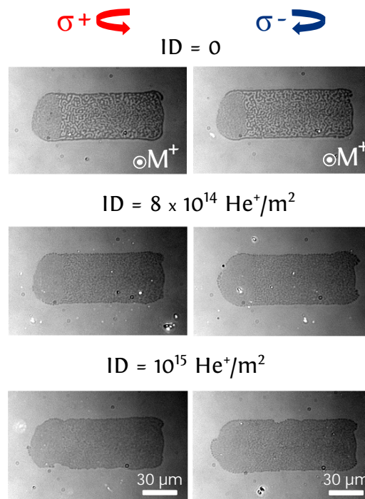
FIGURE 3.22: Optical response for [\text{Co}(0.6 \text{ nm})/\text{Pt}(0.7 \text{ nm})]_4 multilayers as a function of the irradiation dose ID. A pure TD is obtained and the domain size in the laser excited decreases by increasing ID up to 10^{15} \text{ He}^+/\text{m}^2 . The measurements were performed using a constant laser power of 2.5 mW.
