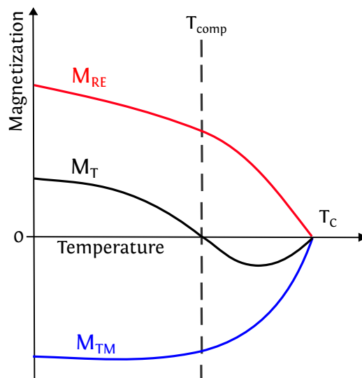
FIGURE 2.5: Temperature dependence of the net magnetization M_T and the sublattice magnetizations M_{RE} and M_{TM} . T_{comp} is the compensation temperature at which the two different sublattices compensate.
