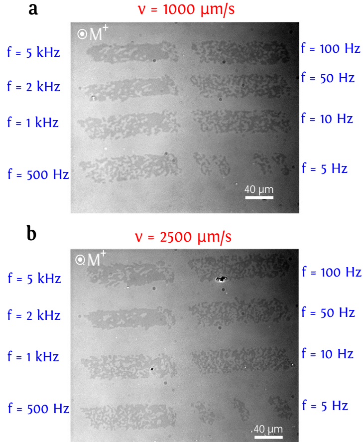
FIGURE 4.9: (a) and (b) Magneto-optical response of Pt(3.7 nm)/Co(0.6 nm)/Pt(3.7 nm) continuous film to right-circularly polarized laser beam swept from left to right at sweeping speeds of 1000\ \mu\text{m/s} and 2500\ \mu\text{m/s} , respectively. The used laser power is 0.7 mW and the repetition rate is varied from 5 kHz to 5 Hz. The initial up magnetization saturation is exemplarily shown and the dark contrast corresponds to a reversal to down.
