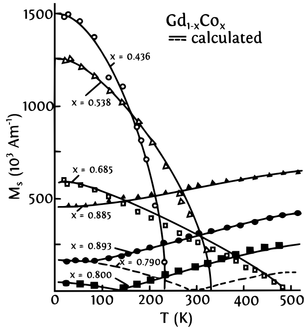
FIGURE 2.6: Temperature dependence of the saturation magnetization for GdCo alloys. The solid and dashed lines were calculated from the mean-field theory. Figure adapted from [6].
