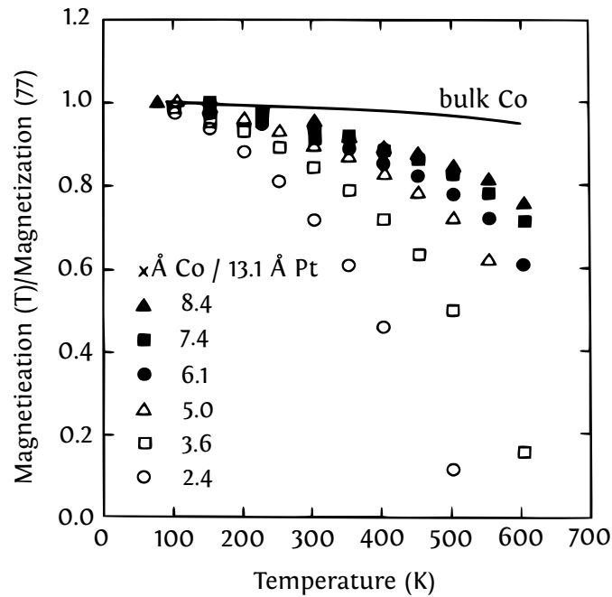
FIGURE 2.7: Temperature dependence of the magnetization of Co/Pt multilayers (60 bilayers) with varying Co thicknesses. The magnetizations are normalized to those at 77 K. Figure adapted from [14].
