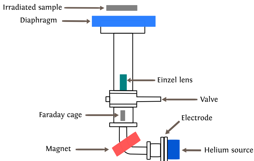
FIGURE 2.2: Schematic representation of He + -irradiation setup.
