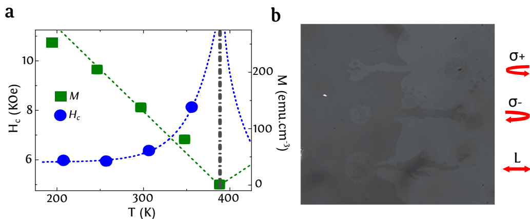
FIGURE 1.13: Magnetic measurements of a \text{Ta}(4 \text{ nm})/\text{Pd}(3 \text{ nm})/[\text{Co}(1 \text{ nm})/\text{Ir}/\text{Co}(0.4 \text{ nm})/\text{Ni}(0.6 \text{ nm})/\text{Pt}(0.3 \text{ nm})/\text{Co}(0.4 \text{ nm})]_5/\text{Pd}(3 \text{ nm}) SFI structure. (a) Remanent magnetization M and coercive field H_c as a function of temperature allow us to define a compensation temperature at T_{\text{Mcomp}} = 380 \text{ K} . (b) Images after scanning the laser with three types of polarized beam that were swept over the sample: from top to bottom, right circularly polarized light ( \sigma^+ ), left circularly polarized light ( \sigma^- ) and linear polarized light (L). Figure adapted from [43].
