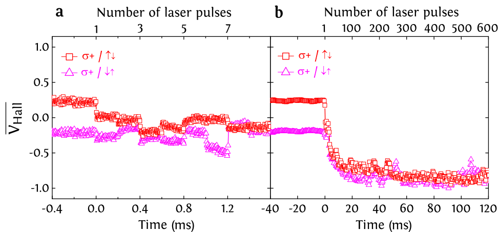
FIGURE 4.45: (a) and (b) Time evolution of the anomalous Hall voltage of a 5- \mu\text{m} -wide Pt(4.5 nm)/Co(0.6 nm)/Pt(4.5 nm) Hall cross which is initially partially demagnetized ( \overline{V_{Hall}} = \pm 0.25 ), under the action of right-circularly polarized beam with a 5 kHz repetition rate and a laser fluence of 10 \text{mJ}/\text{cm}^2 .
