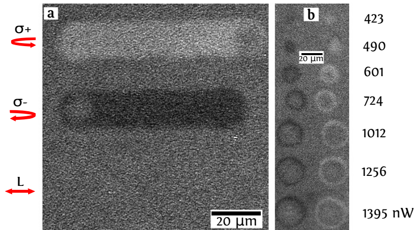
FIGURE 1.16: Magneto-optical response in zero applied magnetic field of a 15-nm FePtAgC granular film sample starting with an initially demagnetized sample. (a) Line scans for \sigma+ , \sigma- and linear polarized light (L). The laser beam was swept over the sample and the magnetization pattern was subsequently imaged. (b) Images of magnetic domains written by keeping the laser spot at a fixed position on the sample. The laser was either \sigma+ polarized (left column) or \sigma- polarized (right column). The laser power is given next to the image. Figure adapted from [53].
