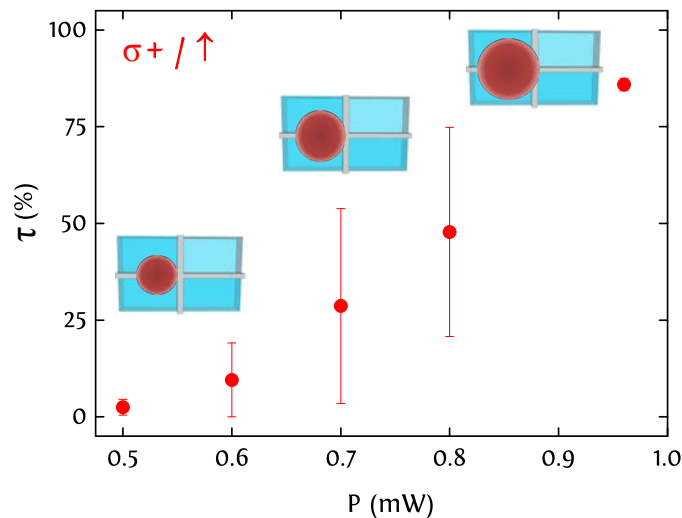
FIGURE 4.18: Switching ratio \tau as a function of the laser power P for the static beam measurement. The center of the beam spot is kept fixed at a position approximately 40 \mu\text{m} from the Hall cross center. Shown in the inset is the schematic evolution of the diameter of the AOS rim.
