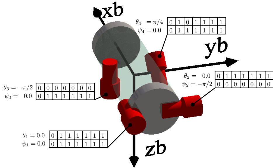
Figure 6.7: Thruster orientation encoding.
