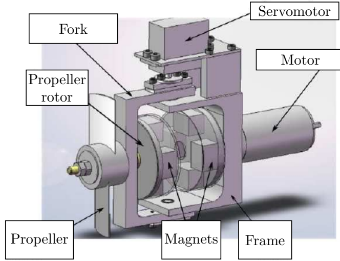
Figure 4.8: RMCT prototype.
