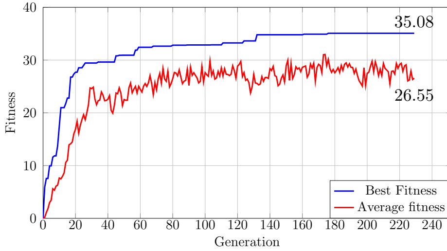
Figure 6.21: Fitness evolution for the global optimization of the RSM robot.
