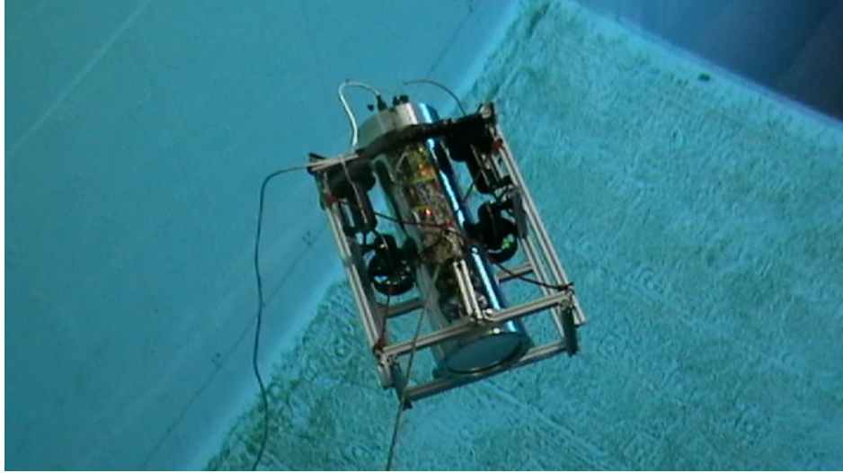
Figure 6.5: Structure of RSM robot (IRDL-ENIB, Brest Ifrement bassin).
