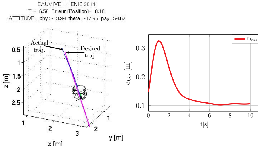
Figure 6.43: EAUUVIVE simulation and kinematic error evolution for diving phase (Dyn. conf.).
