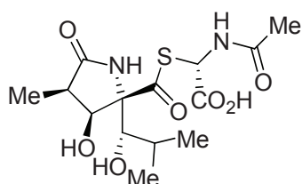
Lactacystine
