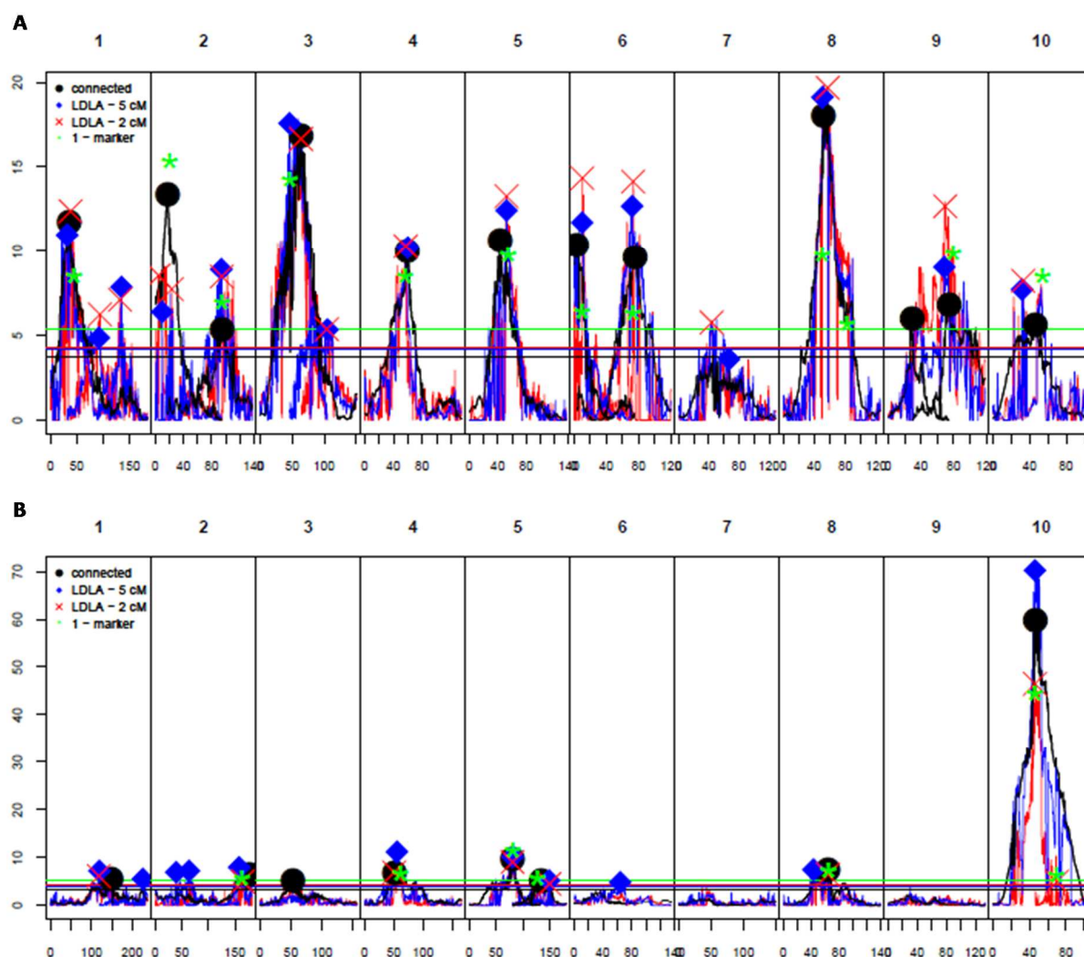
Figure S1 Results of the QTL detection with each model for DMC for (A) the dent design and (B) the flint design. The -\log_{10}(\text{p-values}) of the connected model are represented by black lines, the QTL positions of the connected models by black dots. The -\log_{10}(\text{p-values}) of the LDLA – 5 cM model are represented by blue lines and the QTL positions by blue diamonds. The -\log_{10}(\text{p-values}) of the LDLA – 2 cM model are represented by red lines and the QTL positions by red crosses. The -\log_{10}(\text{p-values}) of the QTL detected by the LDLA – 1-marker model are represented by green stars. Horizontal lines correspond to the threshold values of the different models.
