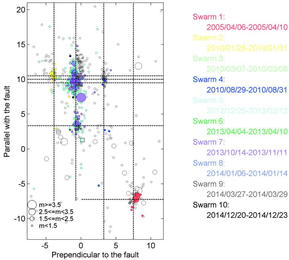
Figure 5.17. Epicenter distribution in map view rotated along orientation of fault ( N146^\circ = \text{vertical} ) of relocated events of Emeelt fault zone (2005 to 2014). Colour indicates swarms and grey colour empty circles indicate events that occurred between swarms.
