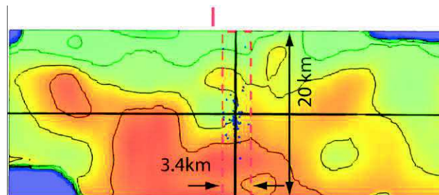
Figure 4.37. Vertical section of V_p model across fault. Vertical black line corresponds to cross-section along fault and horizontal black line corresponds to 10 km depth used in map view. Red line - trench site, red dashed line is border of blue square shown in Figure 4.35. Velocity scale is same as Figure 4.35.
