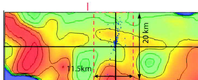
Figure 4.39. Vertical section of Vp model along fault. Vertical black line corresponds to cross-section across fault and horizontal black line corresponds to 10km depth used in map view. Red line - trench site, red dashed line is border of blue square shown in Figure 4.38. Velocity scale is same as Figure 4.38.
