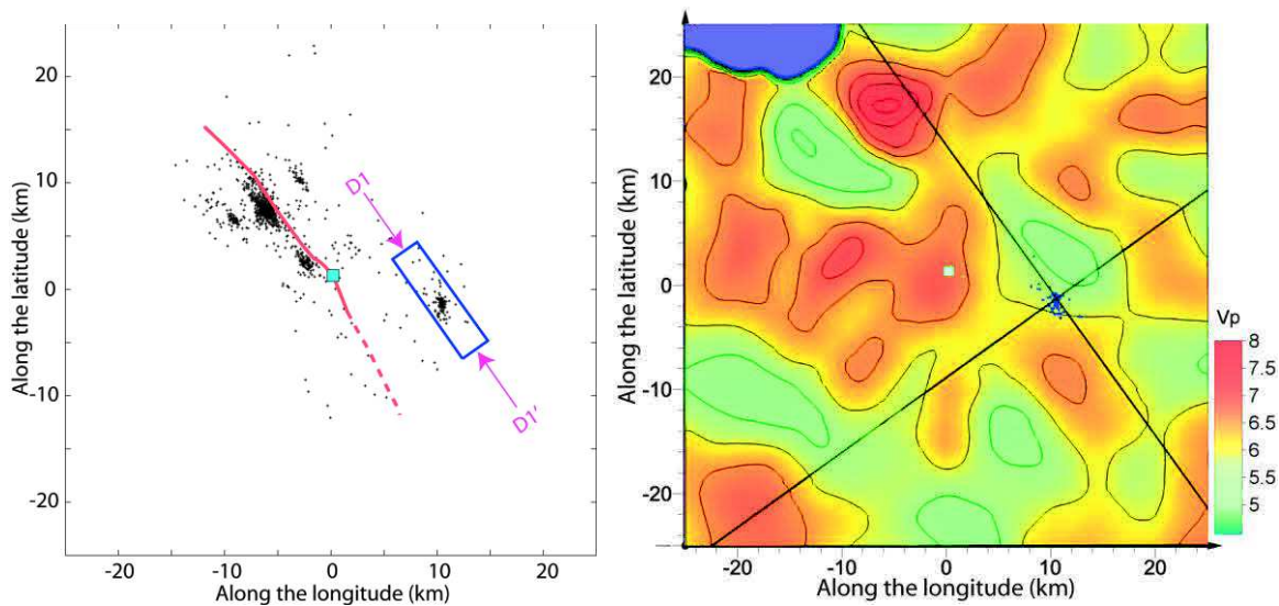
Figure 4.38. Left = Epicentral map and position of polygon D. Red line = Emeelt fault, Aqua square = trench site. Right = Cross section of Vp velocity model at 10 km depth. Blue dot = epicenter in polygon illustrated at left. Black lines are positions of NW-SE and SW-NE vertical cross-sections, respectively, in Figure 4.39 and Figure 4.40.
