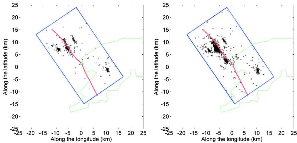
Figure 4.25. Epicentral view of relocated events in TEFZ. Left = 450 events (1995 to 2013-01). Right = 1300 events (1995 – 2014). (Green line = urban area of Ulaanbaatar city, dashed red line = possible Emeelt fault, solid red line = observed surface rupture of Emeelt fault; Aqua square = trench site).
