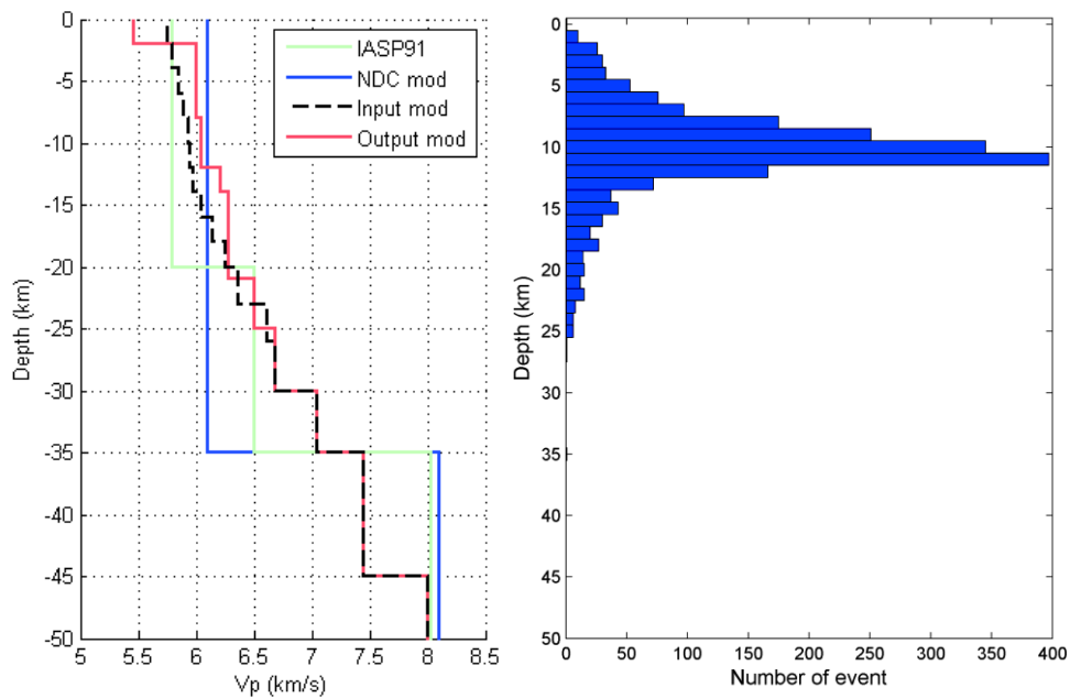
Figure 5.13. Left figure is 1D velocity model and right figure shows depths histogram of seismicity after tomoDD relocation.
