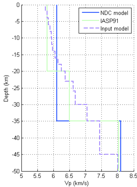
Figure 3.16. Initial 1D velocity model (NDC model after Baljinnyam et al., 1975)
