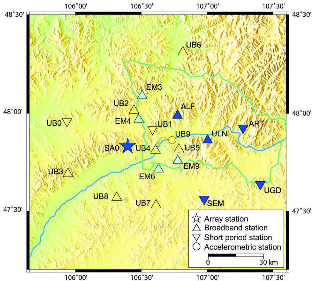
Figure 2.3. Seismic network around Ulaanbaatar area (in January 2013) used in this PhD work. Blue line is Tuul river and green line is asministrative border of Ulaanbaatar city. Blue: “UB-array”, yellow triangles: “UB-mobile”, and aqua: additional mobile stations active during 2 weeks in 2013.
