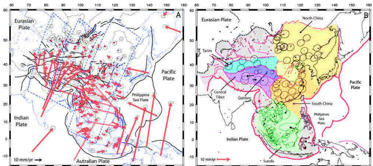
Figure 1.4. (A) Horizontal GPS velocities shown with respect to Eurasia. Large velocities at sites on adjacent plates are shown transparent for a sake of readability. (B) Residual velocities after subtracting rigid block rotations. Dots show locations of all GPS sites. Major blocks are shown with colour backgrounds. White areas are not included in analysis. Error ellipses are 95% confidence interval on both figures (after Calais et al., 2006).
