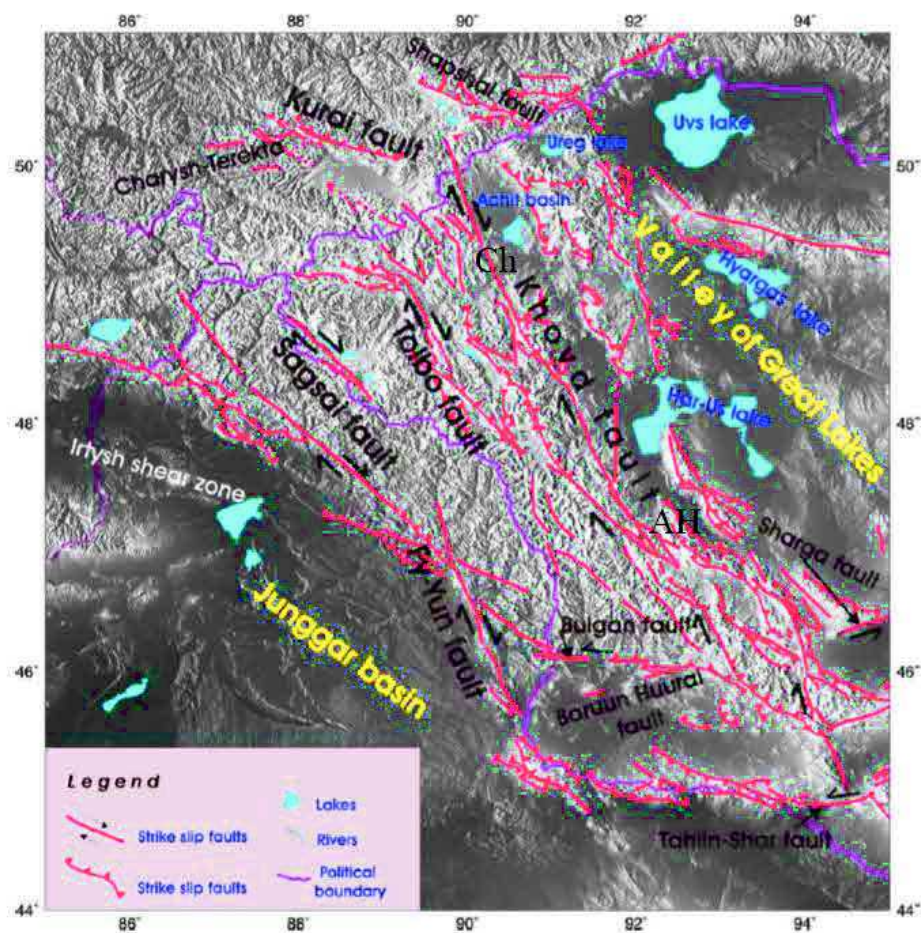
Figure 1.8. Main active structures of Mongolian Altai interpreted using SPOT and Landsat satellite images overlapped on GTOPO30 topography (Ch = Chihte and AH = Ar Hotol) (modified from Munkhuu, 2006).
