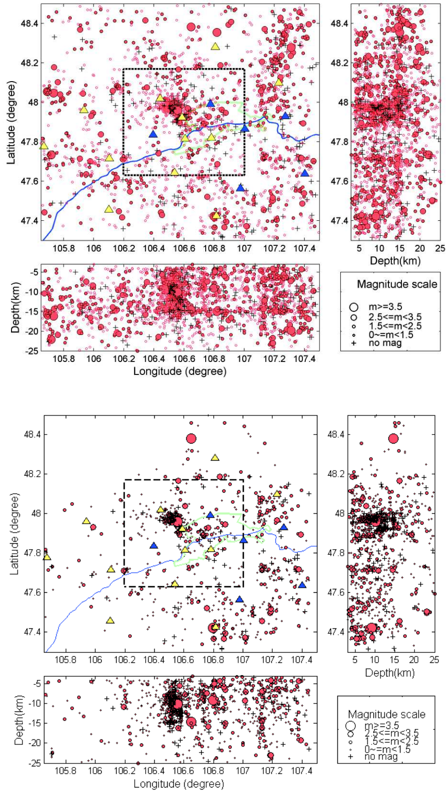
Figure 4.14. Top = Figure 4.14a : Hypoinverse hypocenter locations for the period 1995-2014 (Output B1 and Output B2). Bottom = Figure 4.14b: selected events (Selection D) for the TomoDD relocation = part of the event shown on the figure 4.14a. (Blue line is Tuul river and green line is urban area of Ulaanbaatar city and triangle is seismic station).
