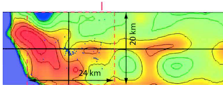
Figure 4.36. Vertical section of V_p model along fault. Vertical black line corresponds to cross-section across fault and horizontal black line corresponds to 10 km depth used in map view. Red line - trench site, red dashed line is border of blue square shown in Figure 4.35. Velocity scale is same as Figure 4.35.
