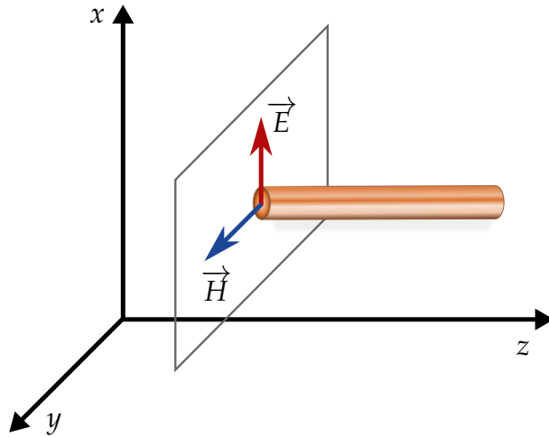
Figure 1.14: Structure of ElectroMagnetic (EM) fields in the TEM mode.
