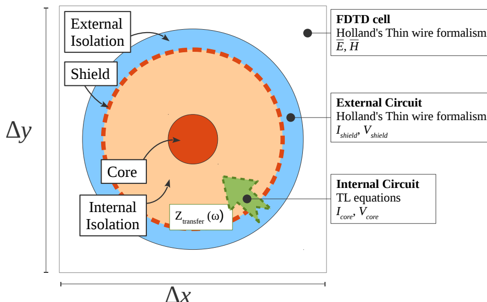
Figure 2.8: Solution methods for each component in a cable
