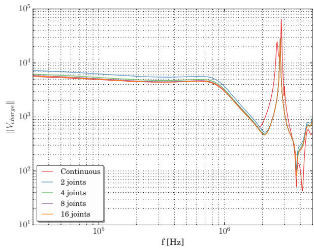
Figure 3.64: Effect of the presence of expansion joints in the frequency response of the voltage at the 50\ \Omega load. Building side. For a negative subsequent stroke.
