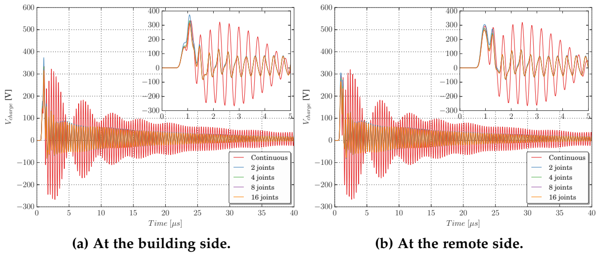
Figure 3.63: Effect of the presence of expansion joints in the voltage at the 50\ \Omega load, for a negative subsequent stroke.
