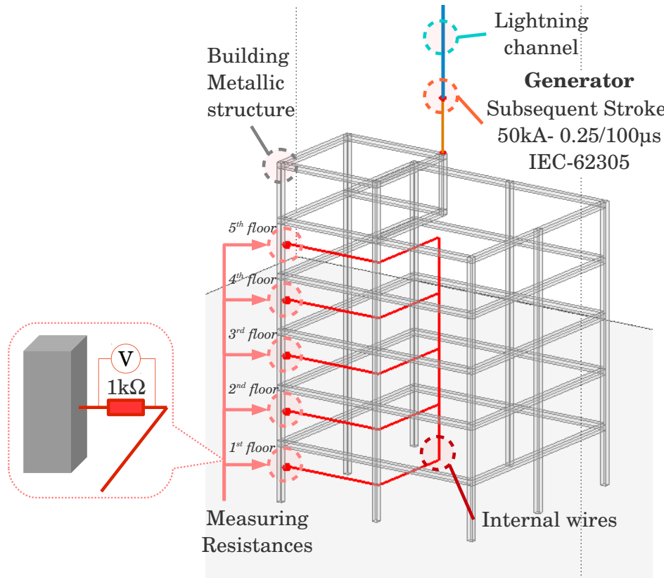
Figure 2.21: Schematic of a building as proposed in [24]
