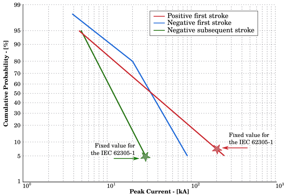
Figure 1.4: Cumulative frequency of the current peak. Adapted from the standard IEC-62305-1 [6]
