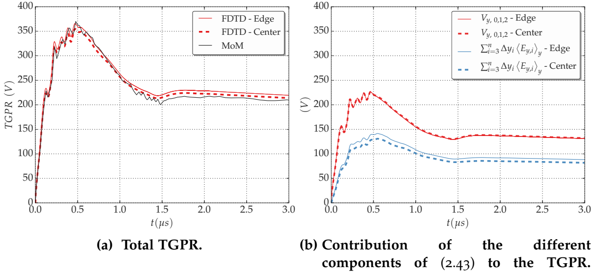
Figure 2.32: Transient potential rise of a vertical conductor.
