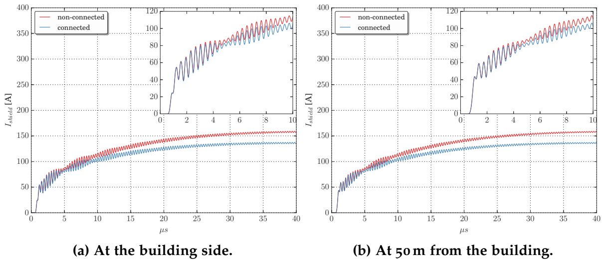
Figure 3.36: Effect of connecting two grounding systems in the shield current for a negative subsequent stroke.
