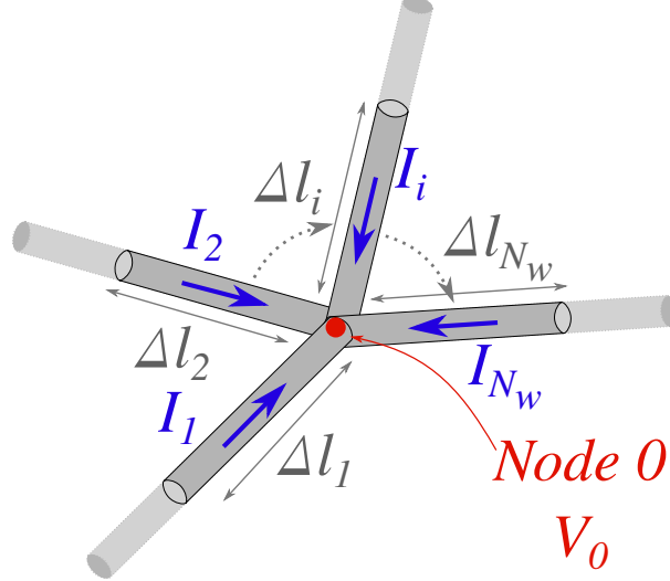
Figure 2.20: Junction of multiple wires.
