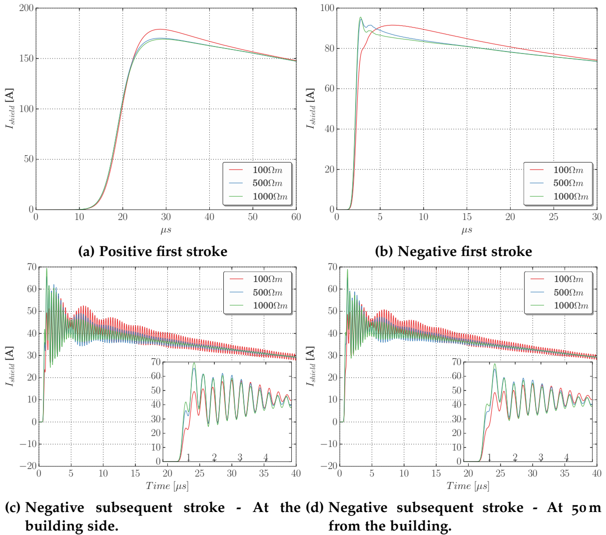
Figure 3.9: Influence of the soil resistivity in the current flowing through the cable shield. For the case depicted in figure 3.1
