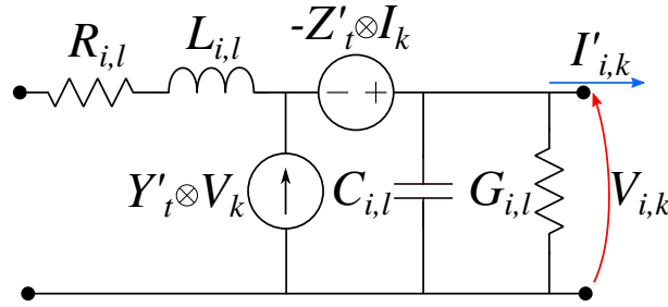
Figure 3.25: Equivalent TL model for a coaxial cable considering the transfer impedance.
