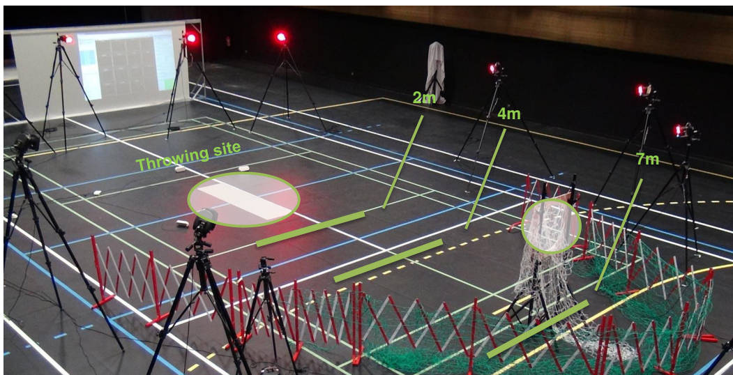
Figure 3.2 – Experimental setup. Throwing site and the different target positions.
