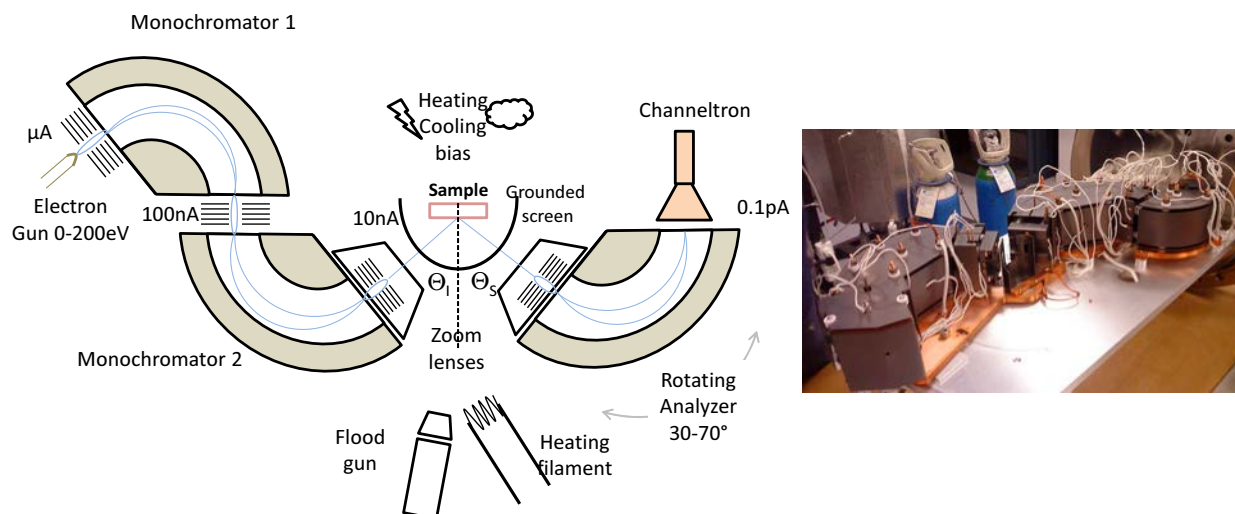
Figure 2.7: The HREELS spectrometer. Electrons emitted by a \text{LaB}_6 filament are monochromated by two 127^\circ cylindrical electrostatic sectors. Focussed particles are reflected by the sample prior to being analysed. The signal is finally amplified by a channeltron. The incident angle \Theta_I is fixed at 60^\circ (with respect to the direction normal to the surface) and the analyser can be rotated to change the scattering angle \Theta_S from 20^\circ to 70^\circ . The sample is mounted on 5-axis manipulator copper head of which can be heated and cooled down. The set-up also involves the above mentioned (Sect 2.2.3) tungsten filament placed in front on the sample to radiatively anneal the surface and the additional electron gun that can be used to irradiate the sample with electrons.
