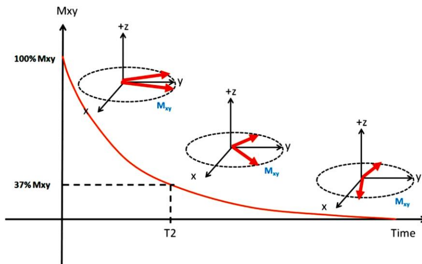
Figure 7. T2 relaxation: the time it takes for M_{xy} to decrease to 37% of initial M_{xy} . Ref. (66)
