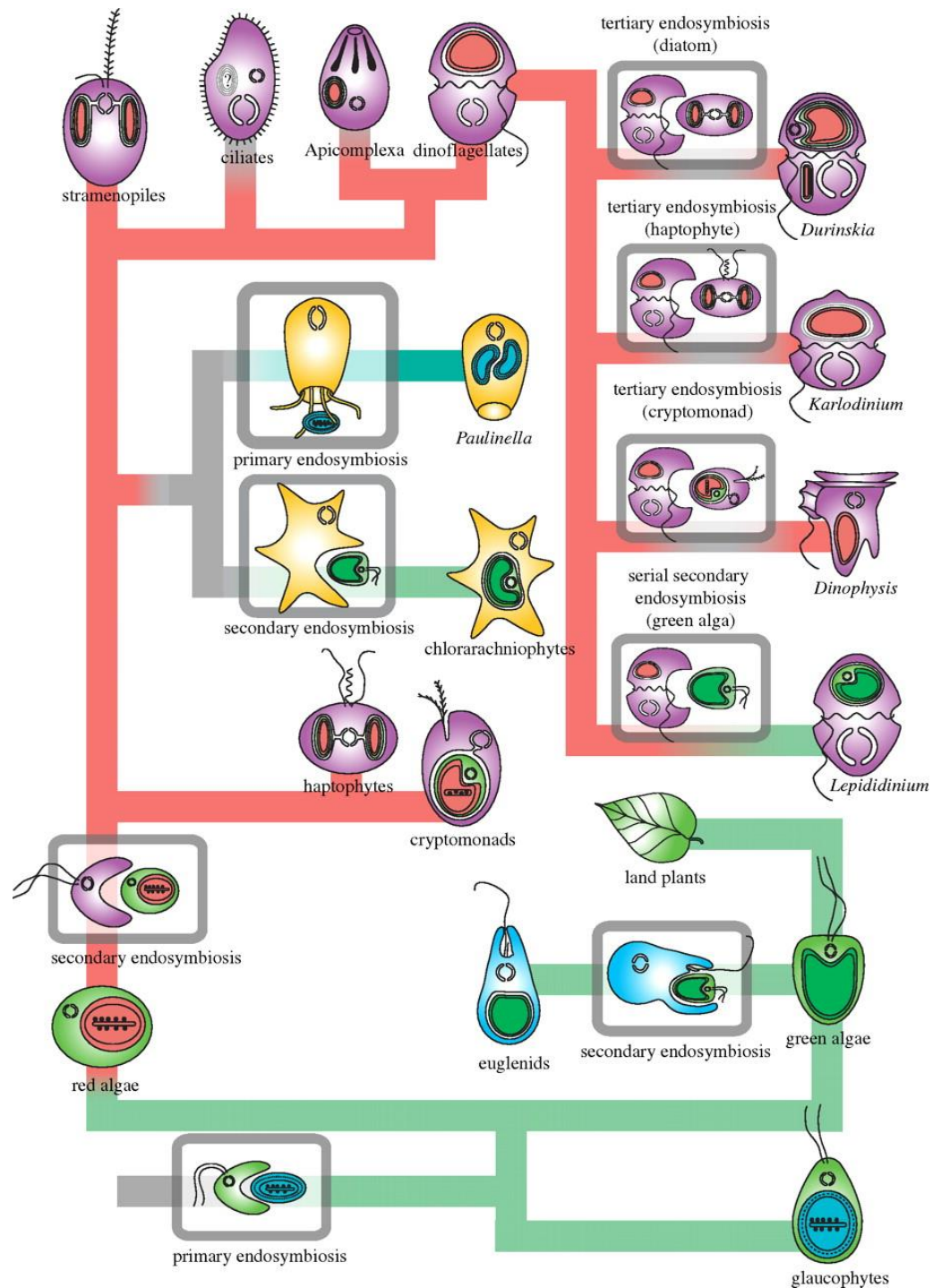
Figure 3 Hypothetical evolution pathway of plastid inheritance in eukaryotic phytoplankton. The primary endosymbiont generated the green algae, red algae, and glaucophytes (here followed by a green line), while all other groups of algae result from secondary endosymbiosis of a primary eukaryotic alga (followed by a red line), among which we find the Stramenopiles. Two serial secondary endosymbiotic events, with a green and then a red alga engulfed by the heterotrophic eukaryotes generated diatoms. Figure from (Keeling 2010)
