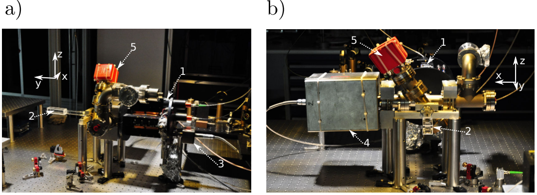
Figure 4.2: Pictures of the vacuum system: (a) side view; (b) front view. The main axis of the experimental set-up are indicated for each pictures. The following elements can be seen on the set-up: 1) 2D MOT , 2) science glass cell, 3) Agilent Technologies 2L/s ion pump, 4) Agilent technologies VacIon 20 L/s, 5) SAES NEX Torr D200-5 ion getter pump.
