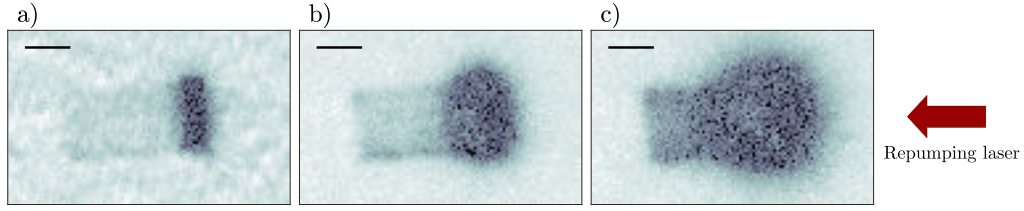
Figure 5.1: Cloud of 15\,\mu\text{m} \times 30\,\mu\text{m} at different repumping times: (a) 10\,\mu\text{s} , (b) 25\,\mu\text{s} , (c) 50\,\mu\text{s} . The atoms acquire a velocity after being repumped from one hyperfine state to the other which is much larger than the recoil velocity. It can be explained by large light-mediated repulsion when one atom of a pair is in the excited F' = 2 state. Scale bars correspond to 10\,\mu\text{m} .
