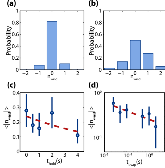
Figure 3.11: Study of the winding number. (a) and (b) Histograms showing the statistical appearance of winding number n_{\text{wind}} for t_{\text{hold}} = 0.5 \text{ s} . (a) We show the result of 39 realizations for t_{\text{evap}} = 2 \text{ s} . We get \langle n_{\text{wind}} \rangle = 0.03(8) . (b) We show the result of 36 realizations for t_{\text{evap}} = 0.025 \text{ s} . We get \langle n_{\text{wind}} \rangle = 0.19(14) . (c) Mean absolute winding number \langle |n_{\text{wind}}| \rangle as a function of hold time ( t_{\text{evap}} = 2 \text{ s} ). The data is fitted with an exponential with a time constant of 7 s. (d) Mean absolute winding number \langle |n_{\text{wind}}| \rangle as a function of evaporation time ( t_{\text{hold}} = 0.5 \text{ s} ) in log-log scale. The line is a power-law fit to the data, \langle |n_{\text{wind}}| \rangle \propto t_{\text{evap}}^{-\alpha} , gives \alpha = 0.19(6) . The uncertainty on \langle n_{\text{wind}} \rangle and the bars on figure (c) and (d) represent the statistical error determined with a bootstrapping approach.
