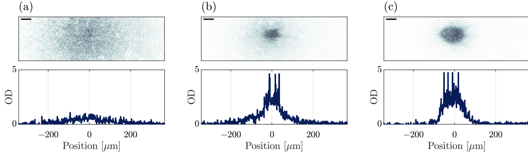
Figure 4.7: Condensation in an all-optical 2D box potential using the vertical imaging axis. The gas is initially trapped in a disk of radius 20\text{ }\mu\text{m} , and released for 8 ms of ToF. In (a), the box potential beam is kept at full power. The power of the box potential beam has been divided (in 0.1 s) by 2.4 in (b) and by 24 in (c). Starting from a thermal distribution, the cloud exhibits first a bimodal distribution then a strong occupation of low-momentum states. Scale bar 50\text{ }\mu\text{m} .
