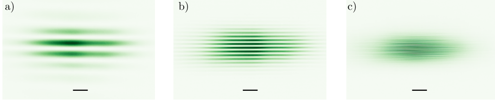
Figure 4.13: Examples of vertical lattices created using the optical accordion set-up proposed in [74]. Light intensities of lattices with spacing (a) 11\ \mu\text{m} , (b) 3.6\ \mu\text{m} and (c) 1.2\ \mu\text{m} . Scale bars indicate a distance of 20\ \mu\text{m} on the atoms.
