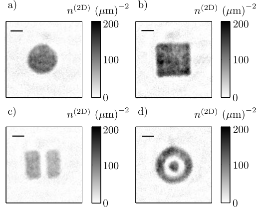
Figure 3.3: (a-d) Examples of in-situ density distributions of uniform gases for different intensity masks. (a) is a disk of radius 12\ \mu\text{m} , (b) a square of length 30\ \mu\text{m} , (c) two rectangular boxes of size 24\ \mu\text{m} \times 12\ \mu\text{m} separated by 4.5\ \mu\text{m} , (d) the so-called “target” potential consisting in a disk of radius 4.5\ \mu\text{m} surrounded by a ring of inner radius 9\ \mu\text{m} and of external radius of 15\ \mu\text{m} . The scale bars indicate a length of 10\ \mu\text{m} .
