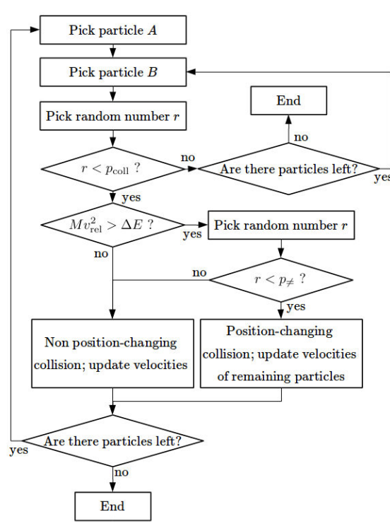
Figure 6.4: Process used to decide for collision events.
