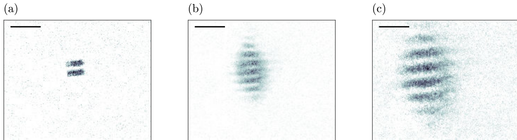
Figure 4.8: Matter-wave interferences in a 2D box potential in the xy plane observed using the vertical imaging axis. The gas is initially trapped in two rectangular boxes of size 15\text{ }\mu\text{m} \times 5\text{ }\mu\text{m} , spaced by 3\text{ }\mu\text{m} (a). After being released for 10 ms (b) and 20 ms (c) ToF, interference fringes are clearly visible. Scale bar 50\text{ }\mu\text{m} .
