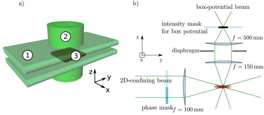
Figure 3.2: Schematic view of the two blue-detuned traps providing the 2D box potential for the atoms. In (a) (1) is the Hermite-Gauss beam providing the 2D, vertical confinement; (2) is the box potential whose production is explained in 3.1.3; the atoms are located in (3). The optical system used to produce the 2D confinement and the box potential is shown in (b).
