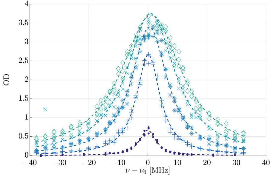
Figure 5.10: Resonance curve for in situ clouds. The various symbols correspond to varying densities: dots 4.0(6) at/ \mu\text{m}^2 , plus signs 25(4) at/ \mu\text{m}^2 , stars 50(7) at/ \mu\text{m}^2 , crosses 75(11) at/ \mu\text{m}^2 , diamonds 100(15) at/ \mu\text{m}^2 . Dashed lines correspond to the lorentzian fit of the curve with the corresponding colour.
