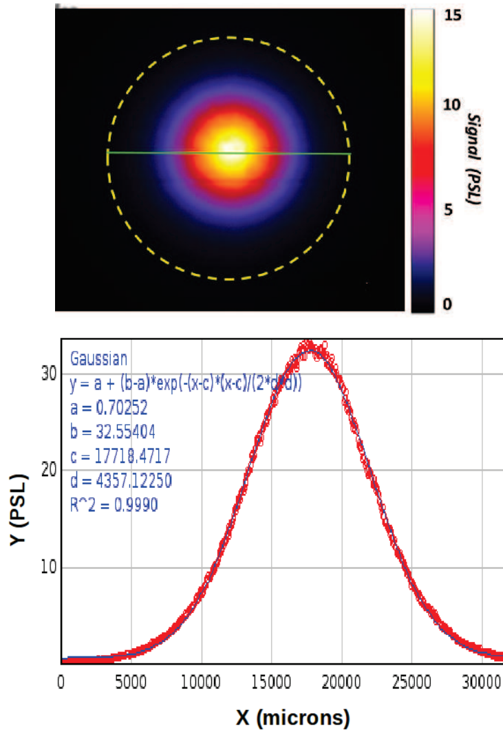
Figure 2.2: The signal detected on an IP
