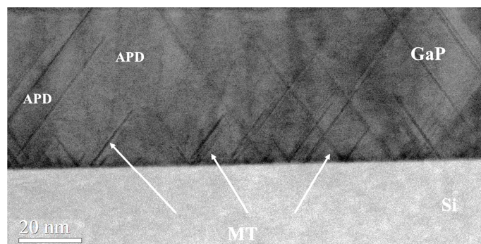
Figure 3.10 Cross-sectional STEM image evidencing the presence of intercrossing MTs in a sample with high MT density. (LPN)
