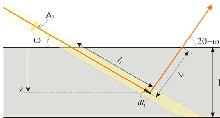
Figure 3.9 Sketch of effective scattering volume in a thin layer, with I_0 and A_0 the intensity and cross section of the incident X-ray beam, \omega and 2\theta - \omega the incident and emergent angle and T the layer thickness.
