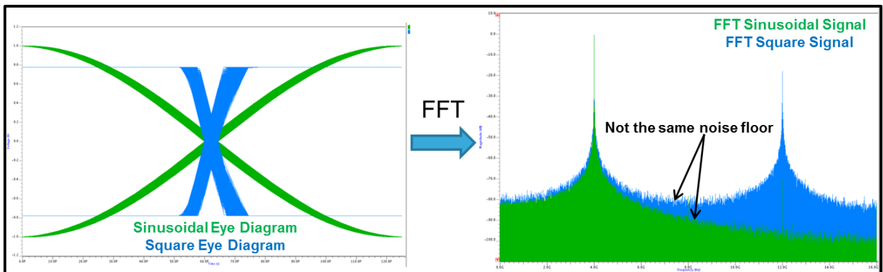
Figure 8-28: Sin/Square Signals Eye Diagrams & FFT
