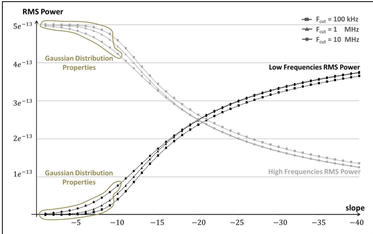
Figure 4-19: RMS power of low and high frequencies
