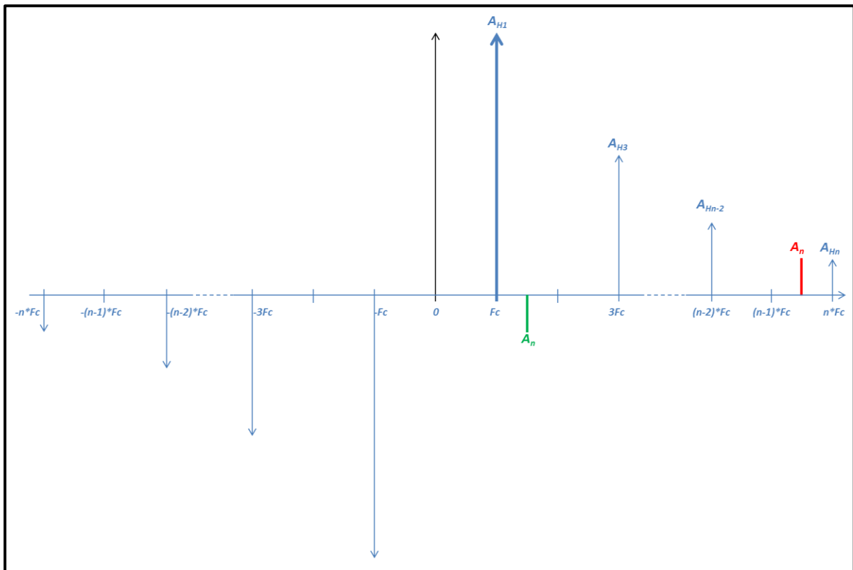
Figure 8-17: Frequency representation – Noise spurs aliased from 0 to 2*Fc.
