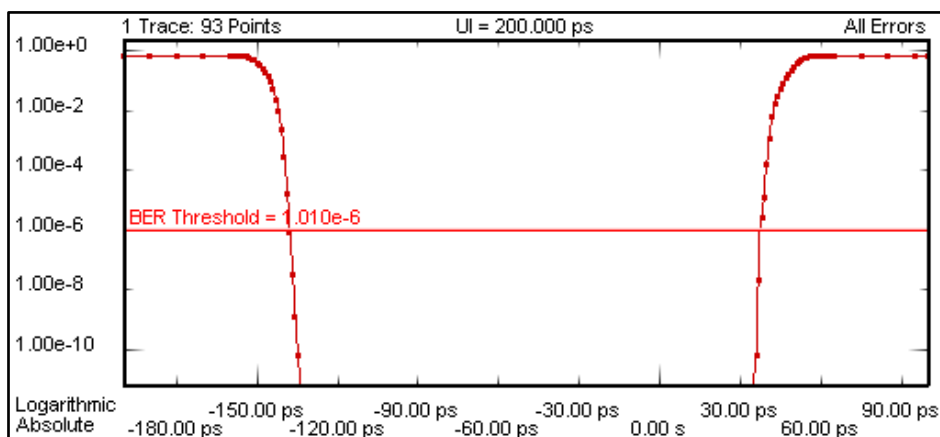
Figure 4-2: J-BERT Measurement
