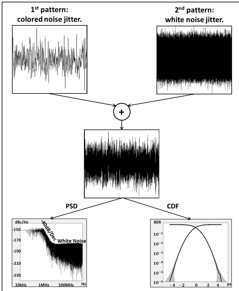
Figure 4-21: Step 2 - Generating colored noise profiles with Gaussian distribution.
