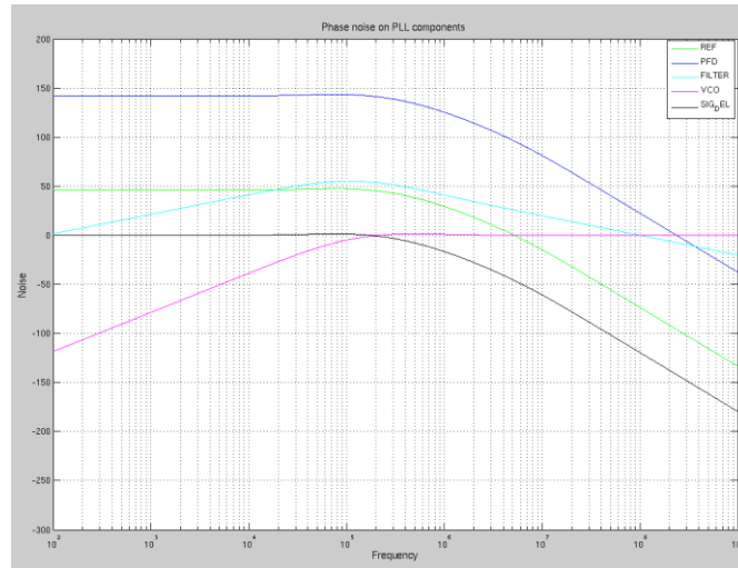
Figure 3-10: Noise Transfer Function for each sub-block of the PLL
