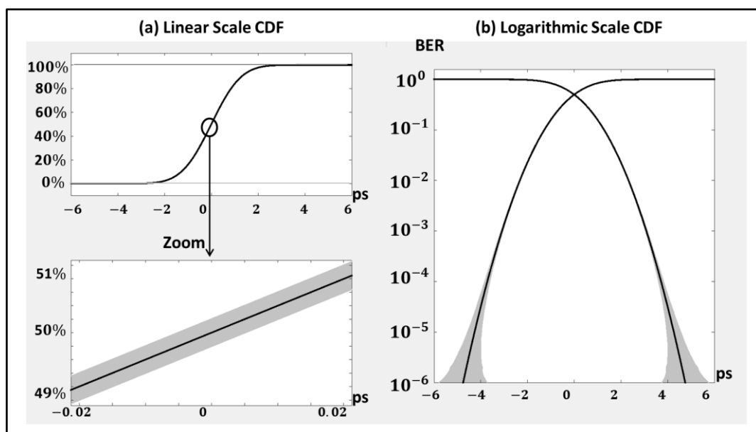
Figure 4-7: CDF Templates to ensure Gaussian distribution for the generated pattern
