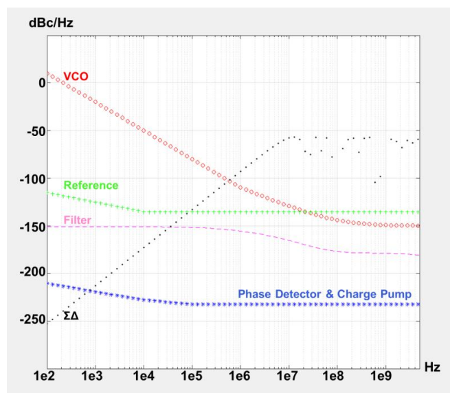
Figure 3-11: Open-loop phase noise profiles
