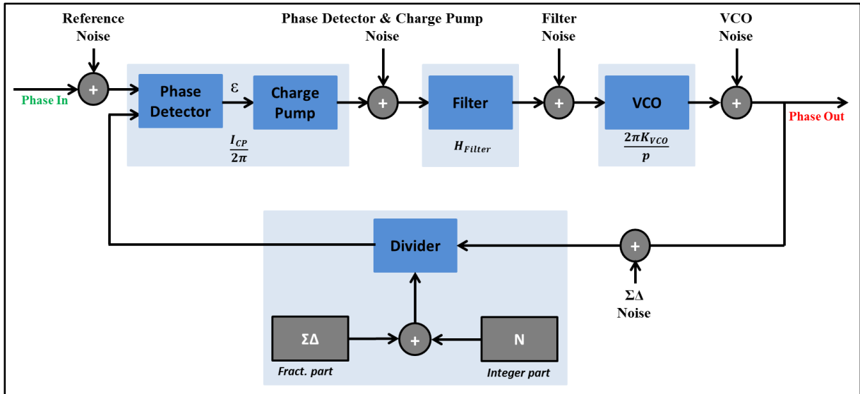
Figure 3-9: PLL Schematic with Phase Noise Injection
