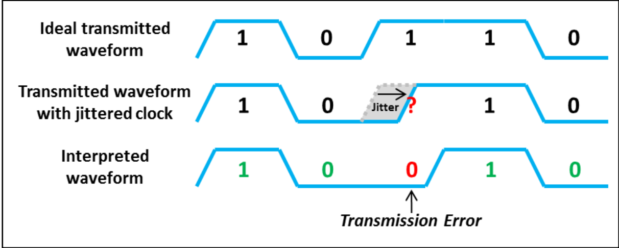
Figure 1-6: Transmission Error due to Jitter
