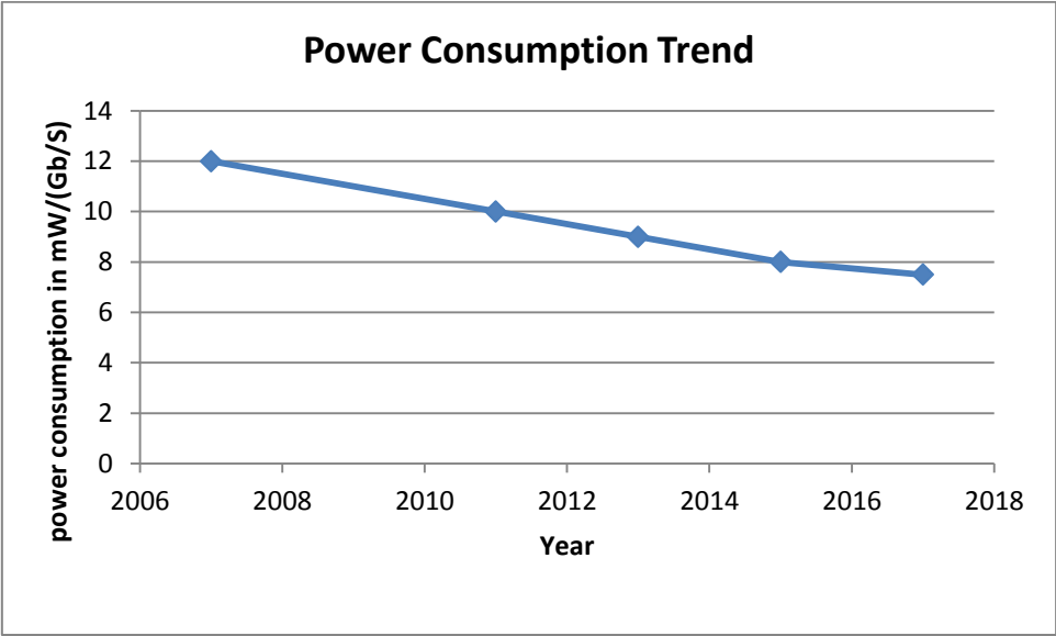
Figure 1-4: Power consumption evolution of STM HSSL circuits.
