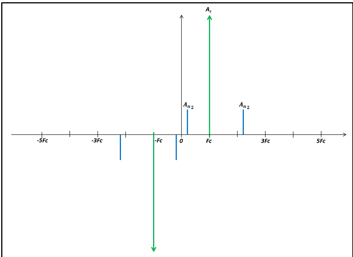
Figure 8-21: Phase Noise Modulation for Sinusoidal Signal
