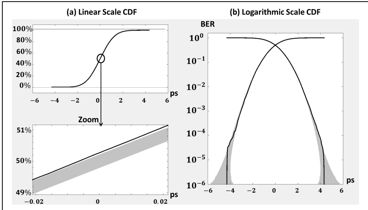
Figure 4-13: CDF & CCDF of Colored Noise generated by Filtering
