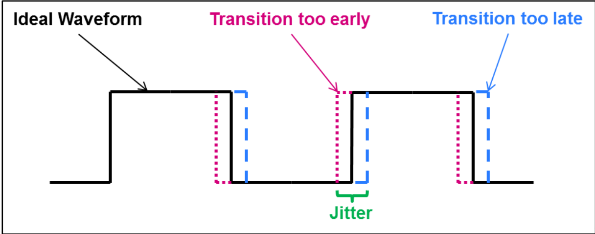
Figure 1-5: Jitter Definition
