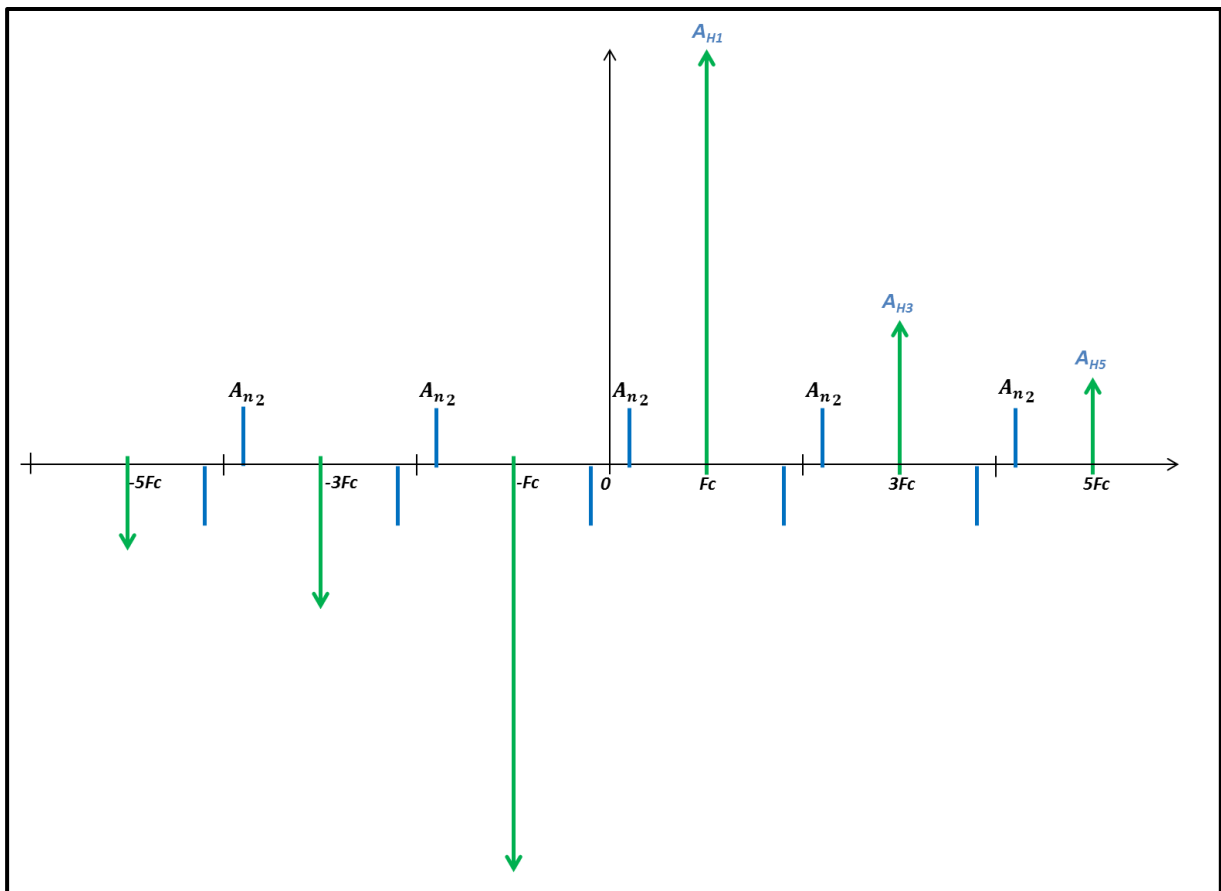
Figure 8-22: Phase Noise Modulation for Square Signal
