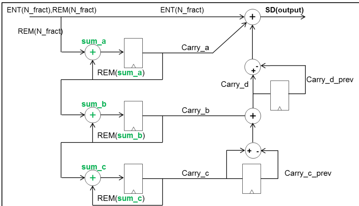
Figure 3-8: Sigma Delta Modulator
