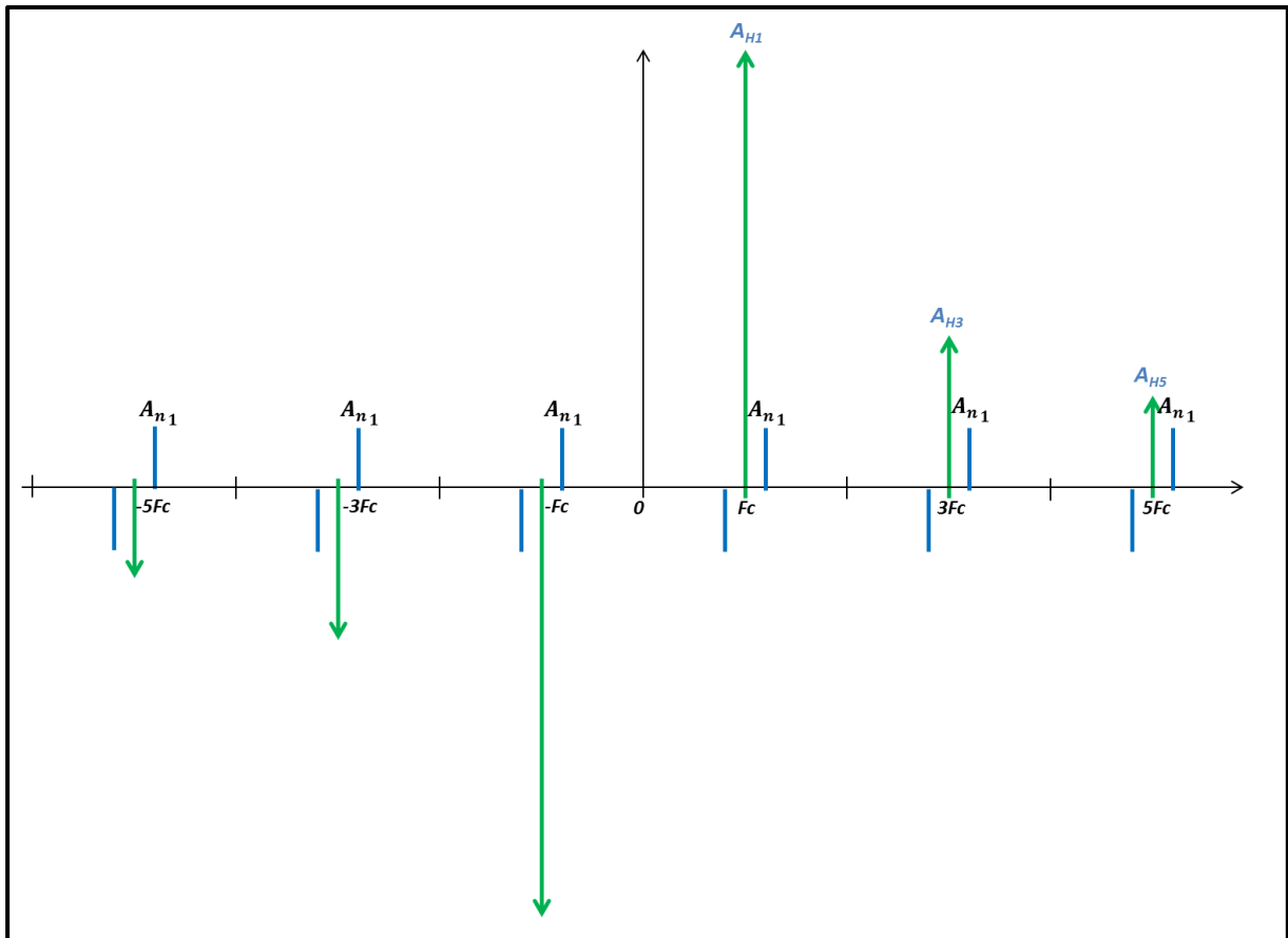
Figure 8-14: Frequency representation of the square modulated signal
