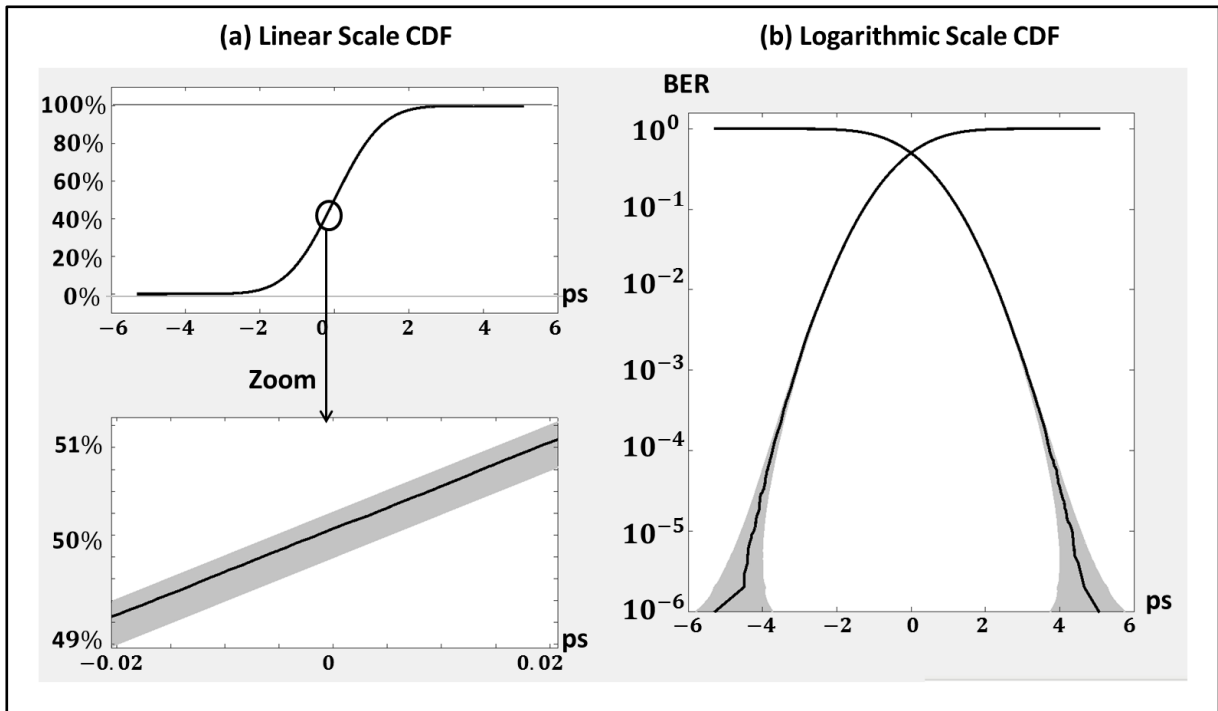
Figure 4-10: CDF & CCDF curves of the generated white noise pattern.
