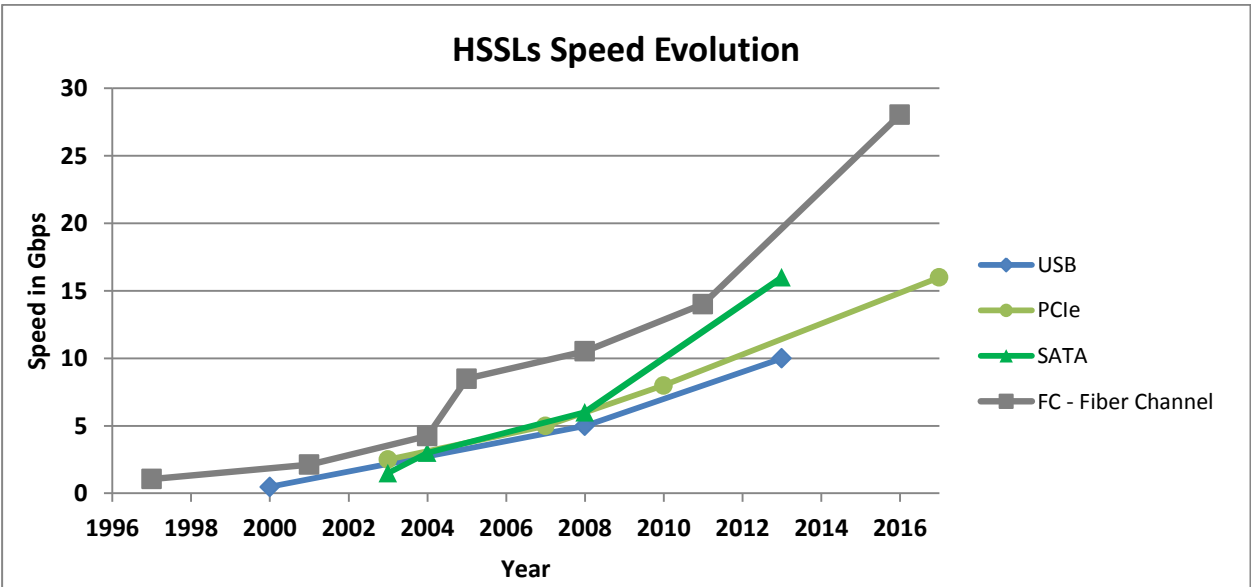
Figure 1-3: HSSLs Speed Evolution over years
