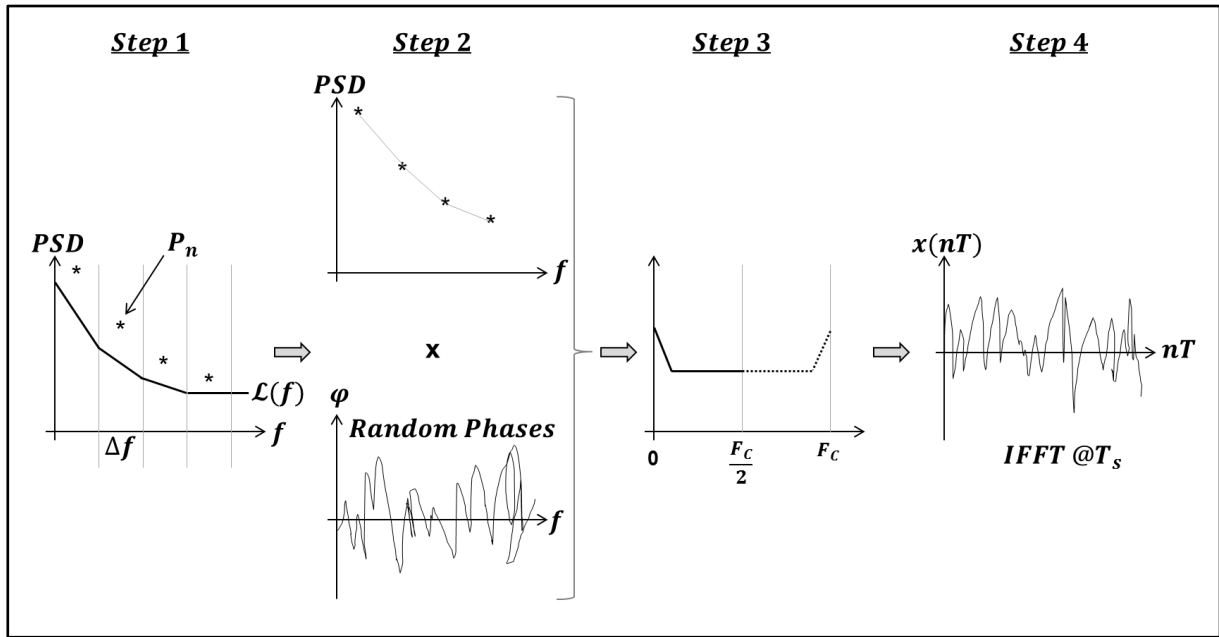
Figure 3-13: Time Jitter Generation Technique
