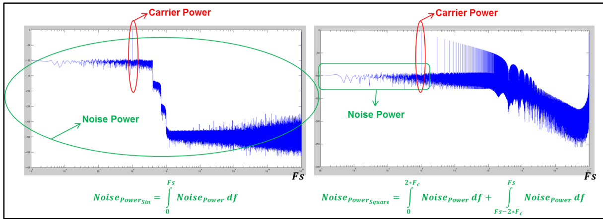
Figure 8-35: FFT of Sinusoidal & Square Noisy Signal - Matlab
