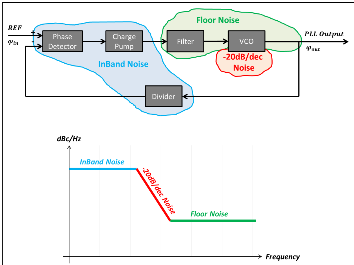
Figure 6-1: PLL Specification Schematic
