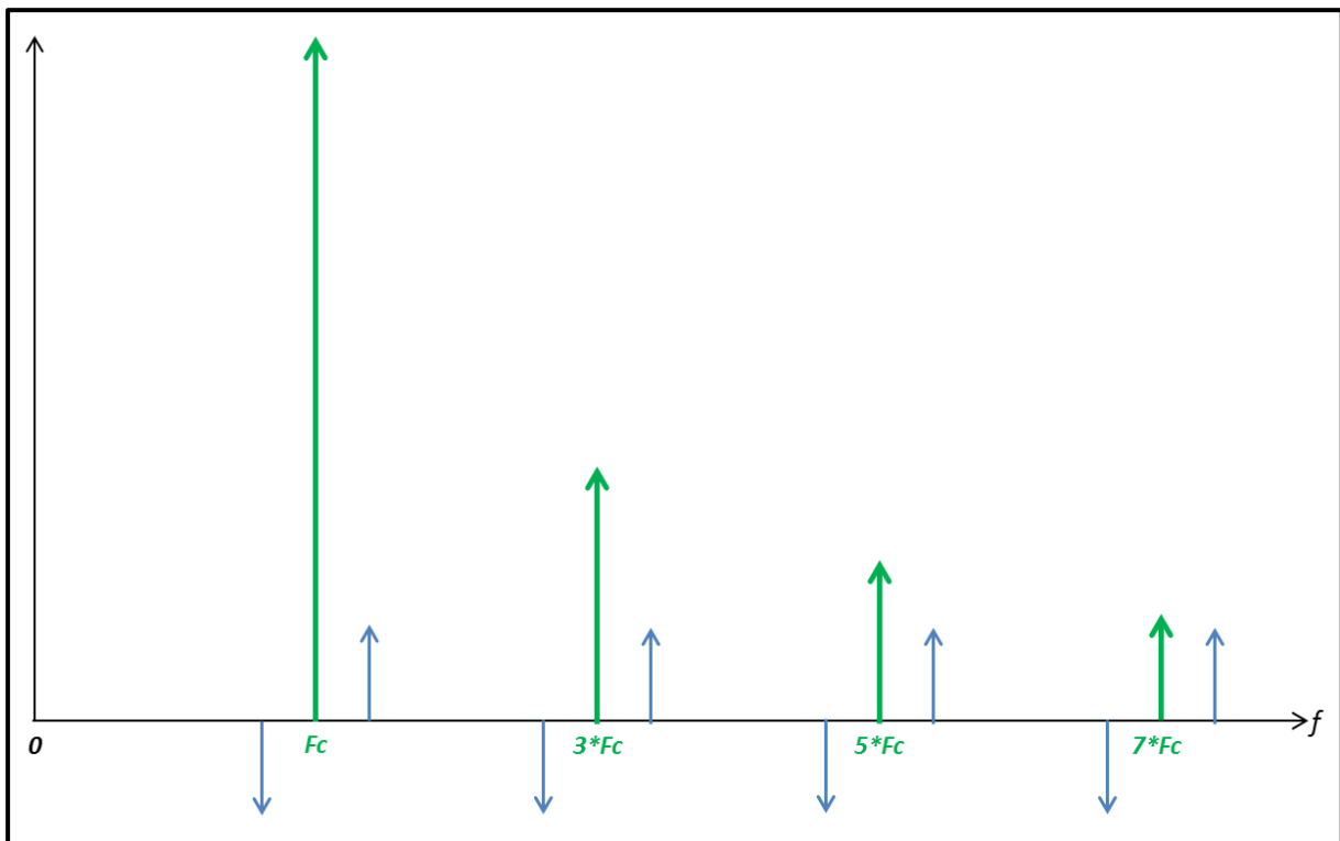
Figure 8-4: Phase Noise Modulation for Square Signal (Frequency Domain)
