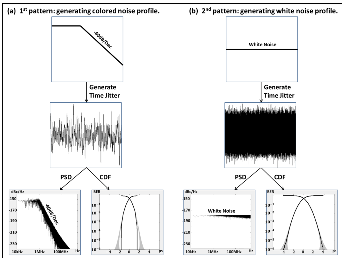
Figure 4-20: Step 1 - Generating white and colored noise profiles.
