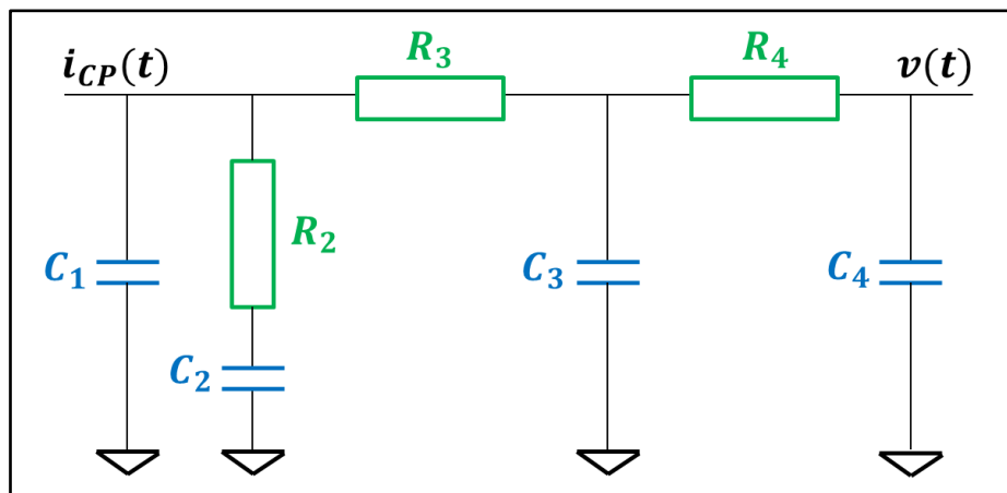
Figure 3-4: Loop Filter Schematic
