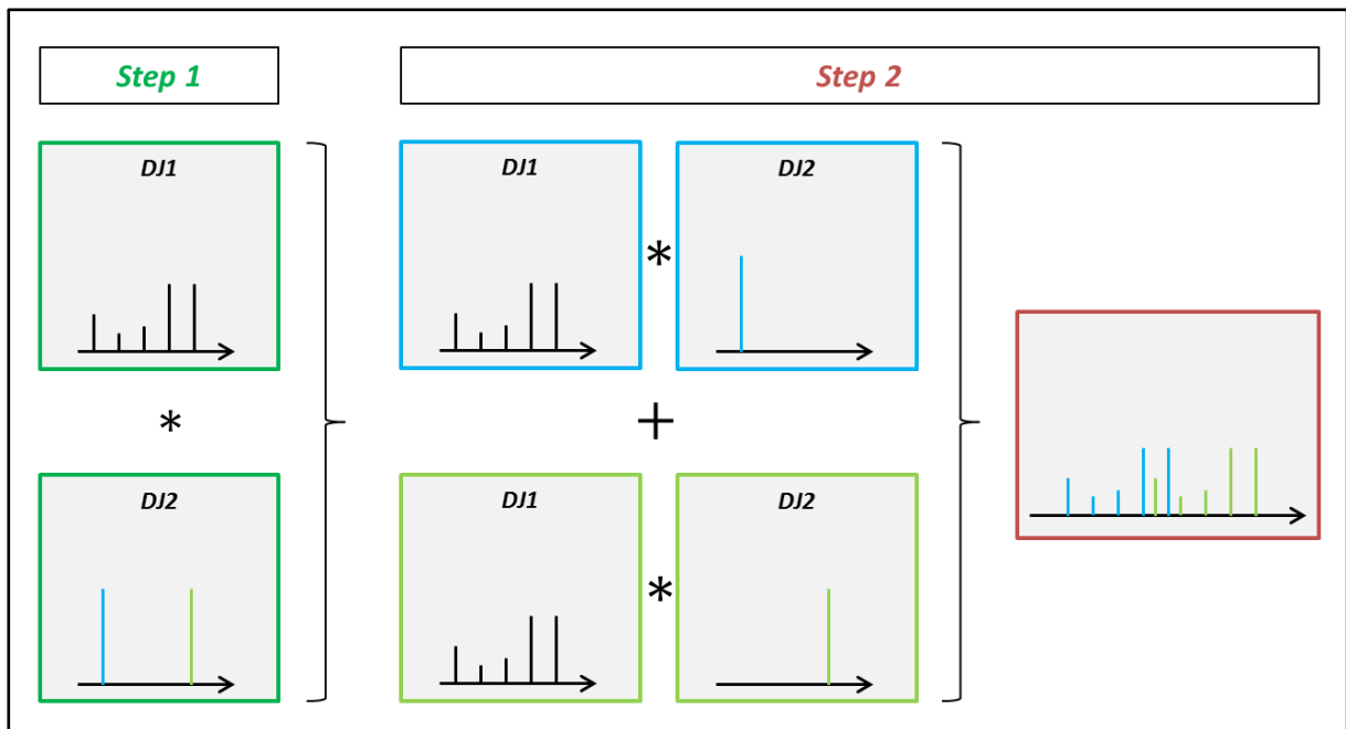
Figure 8-36: Convolution of two DJ Jitters
