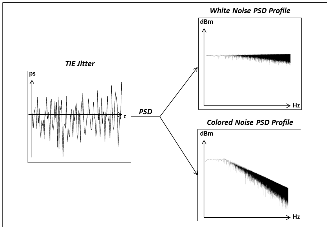
Figure 4-3: Example of a white and colored noise profile
