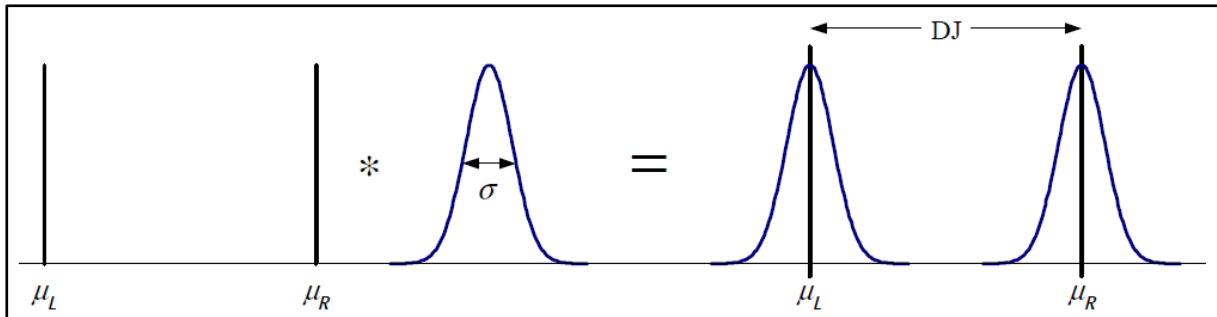
Figure 5-2: Dual-Dirac Method for Jitter Decomposition
