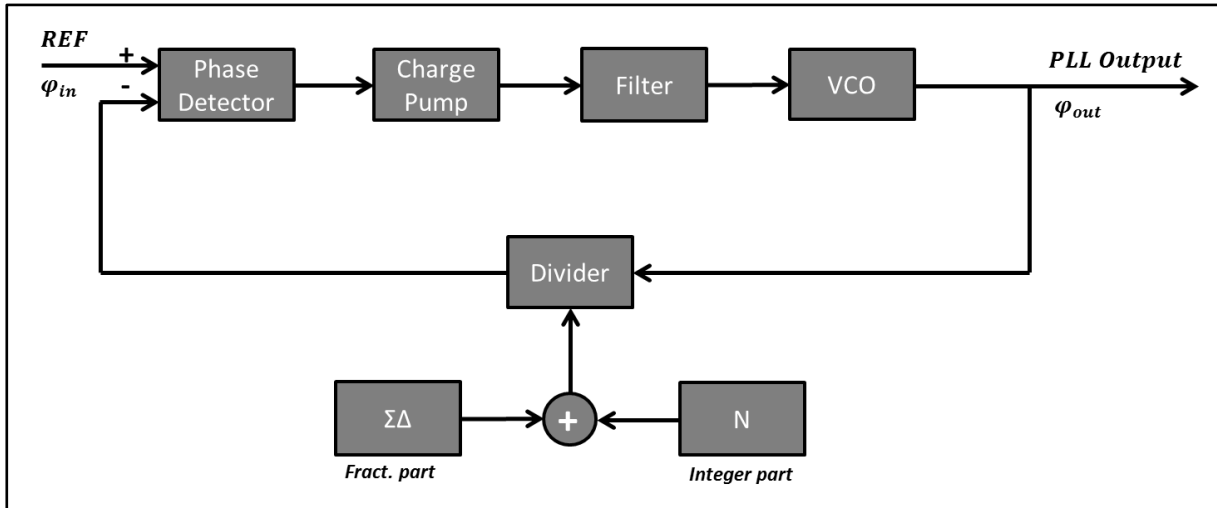
Figure 3-7: PLL schematic with Sigma Delta Modulator
