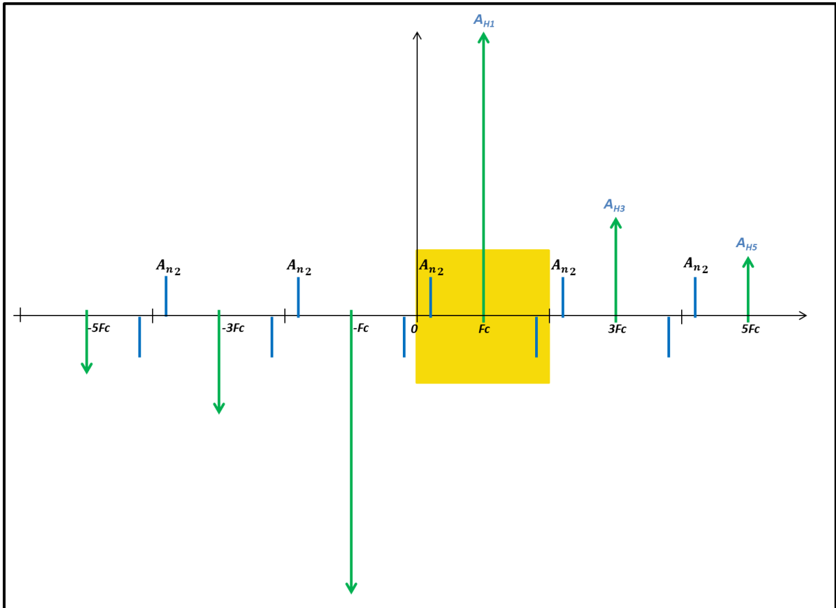
Figure 8-23: Phase Noise Modulation for Square Signal – Integration Band 0->2*Fc
