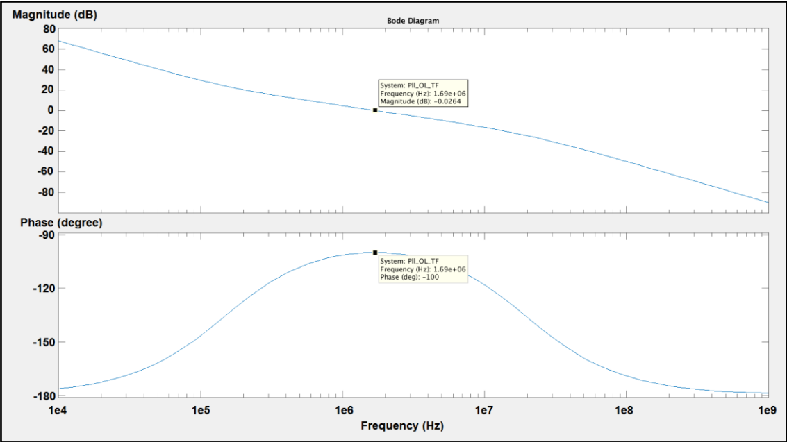
Figure 6-3: Open Loop Transfer Function
