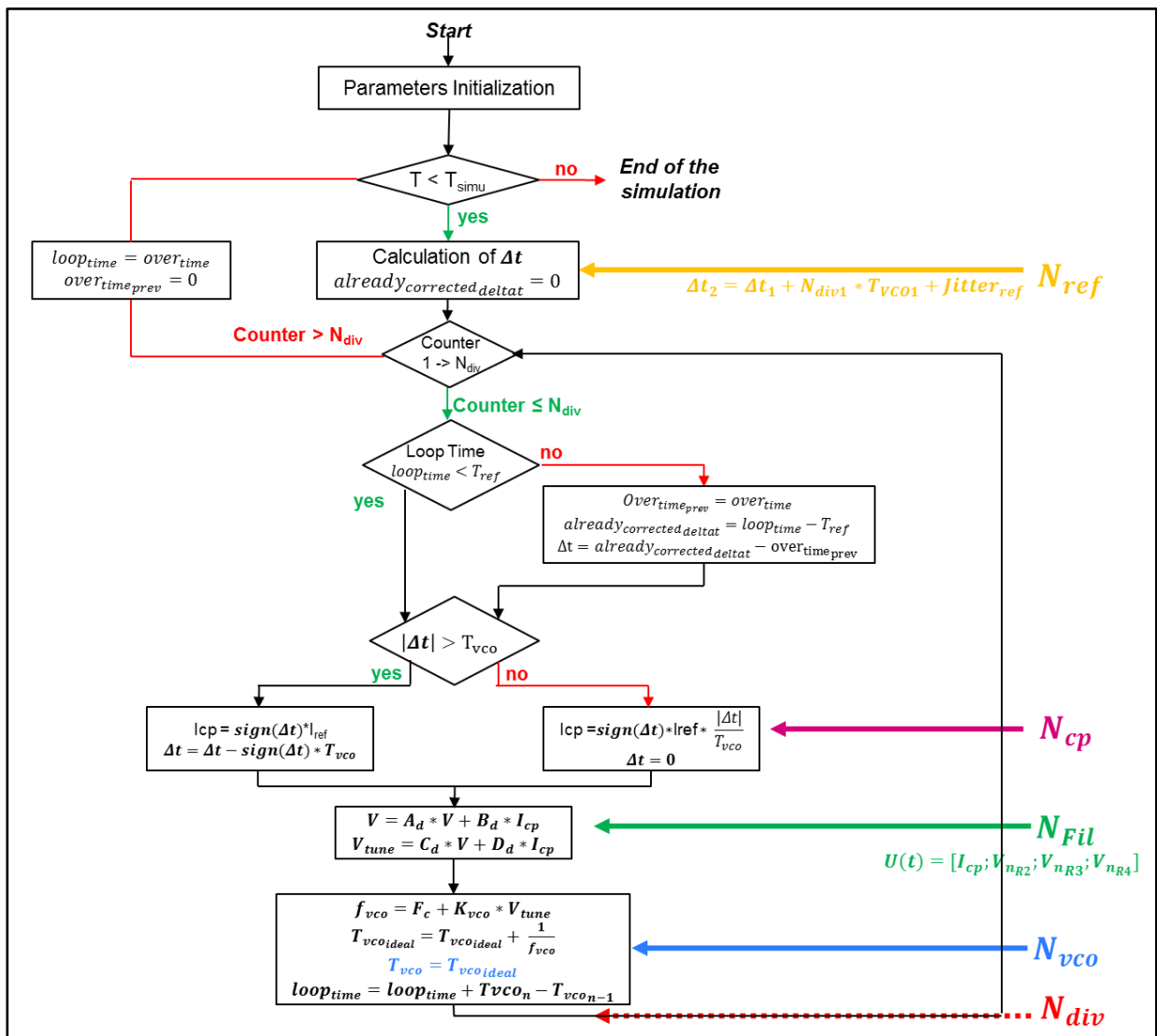
Figure 3-16: Flow Chart with Jitter injection
