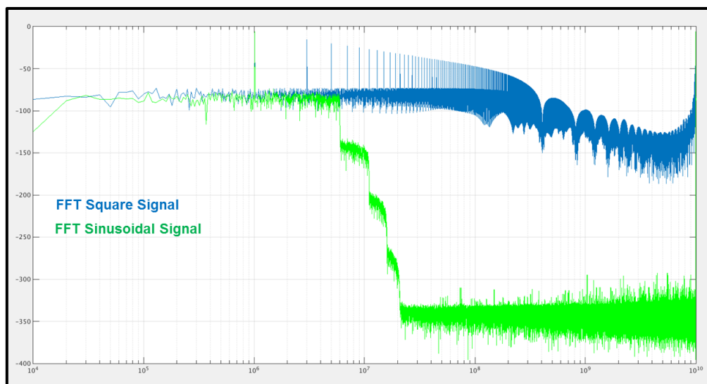
Figure 8-33: FFT of Sinusoidal & Square Noisy Signal - Matlab
