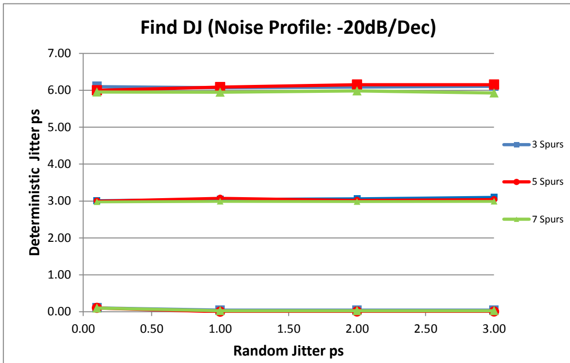
Figure 5-8: DJ for different quantities of generated RJ & DJ Jitter
