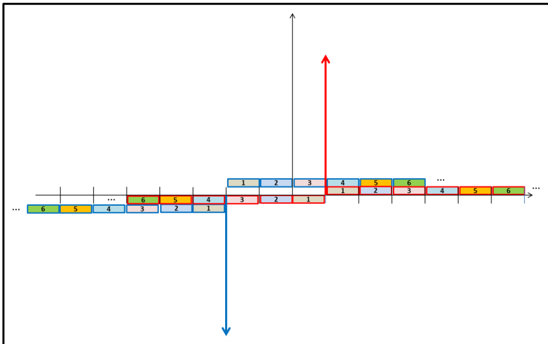
Figure 8-19: Freq. representation of flat noise on Sin. Signal with negative Freq.
