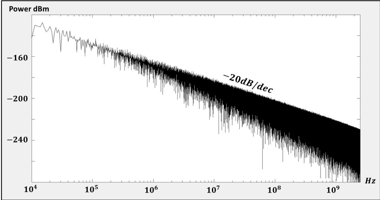
Figure 4-16: PSD of a -20dB/dec generated noise profile
