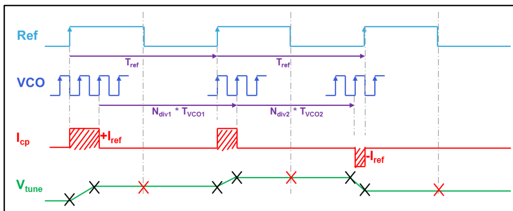
Figure 3-14: Chronogram
