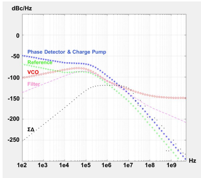
Figure 3-12: Closed-loop phase noise profiles
