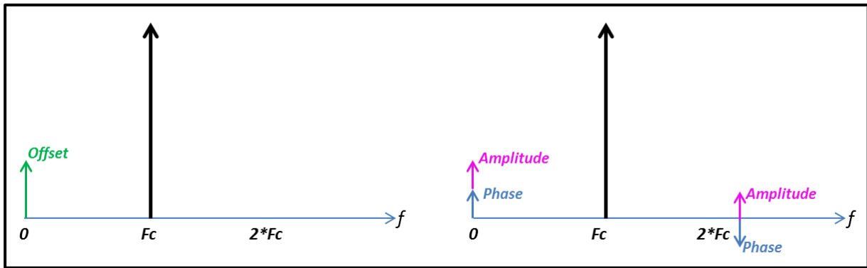
Figure 8-11: Adding an offset to the signal
