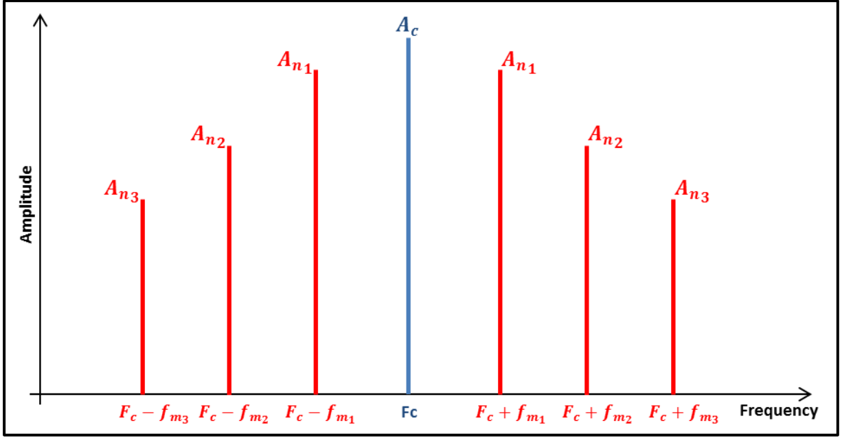
Figure 2-8: Spectral Analysis of multi-spur phase noise modulated signal
