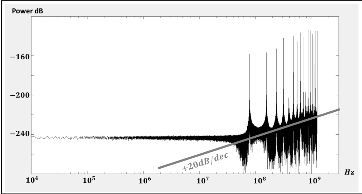
Figure 4-14: DJ Spurs added to random colored noise
