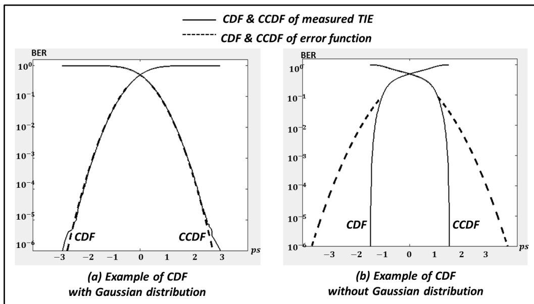
Figure 4-6: Log. scale CDF & CCDF example of a Gaussian and not Gaussian distribution
