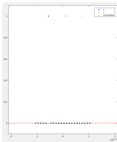
Figure 8-38: Example 2 - Convolution of 1*1 Dirac
