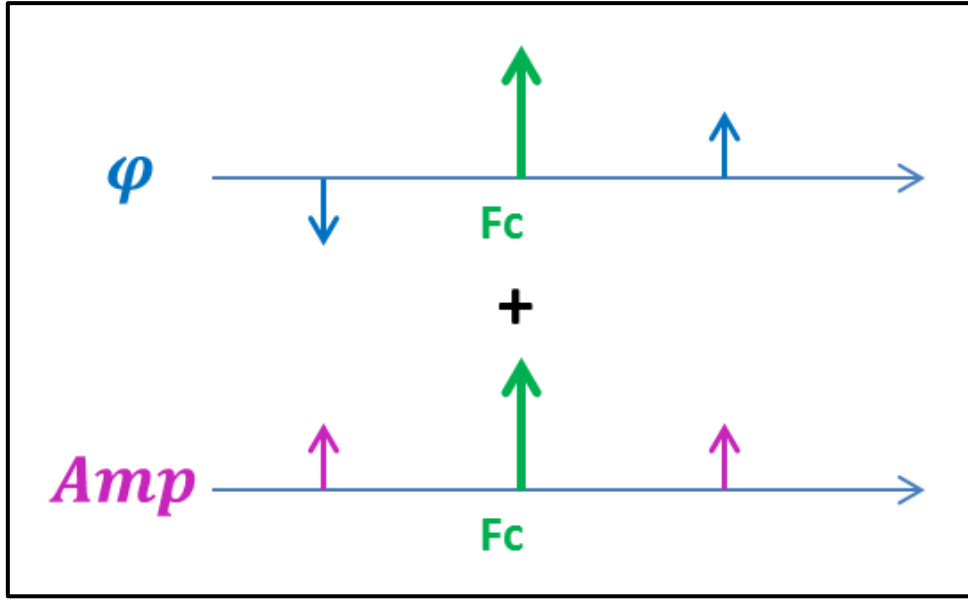
Figure 2-11: Noise decomposition into Amplitude and Phase Noise
