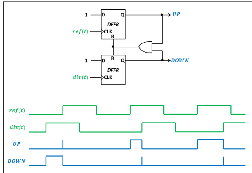
Figure 3-2: Phase-Frequency Detector Output
