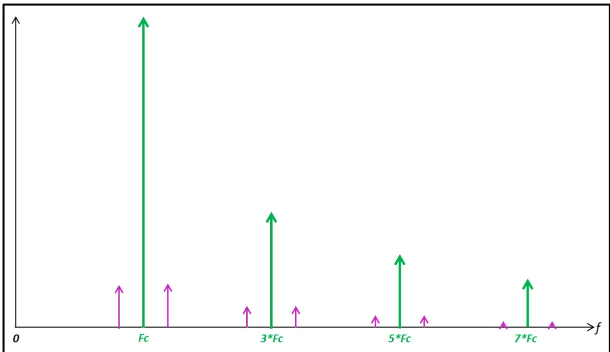
Figure 8-8: Amplitude Noise Modulation for Square Signal (Frequency Domain)
