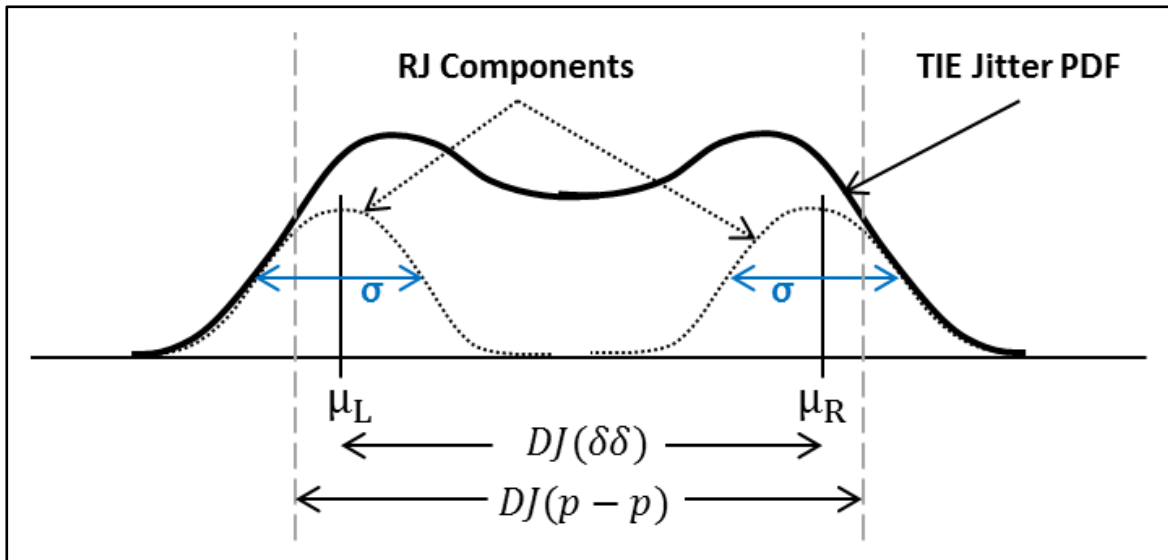
Figure 5-3: Dual-Dirac DJ is smaller than real Peak-to-Peak DJ
