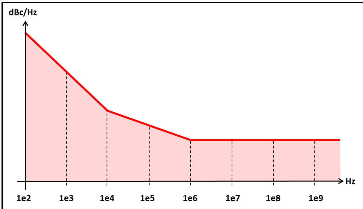
Figure 2-9: Spectral Analysis of Area Profile Phase Noise Modulated Signal
