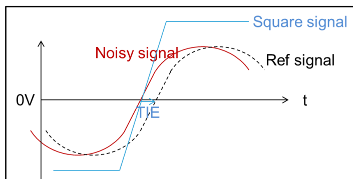
Figure 8-30: TIE for SIN/SQUARE signal
