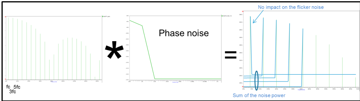
Figure 8-27: Convolute Phase noise profile with Noise Transfer Function FFT
