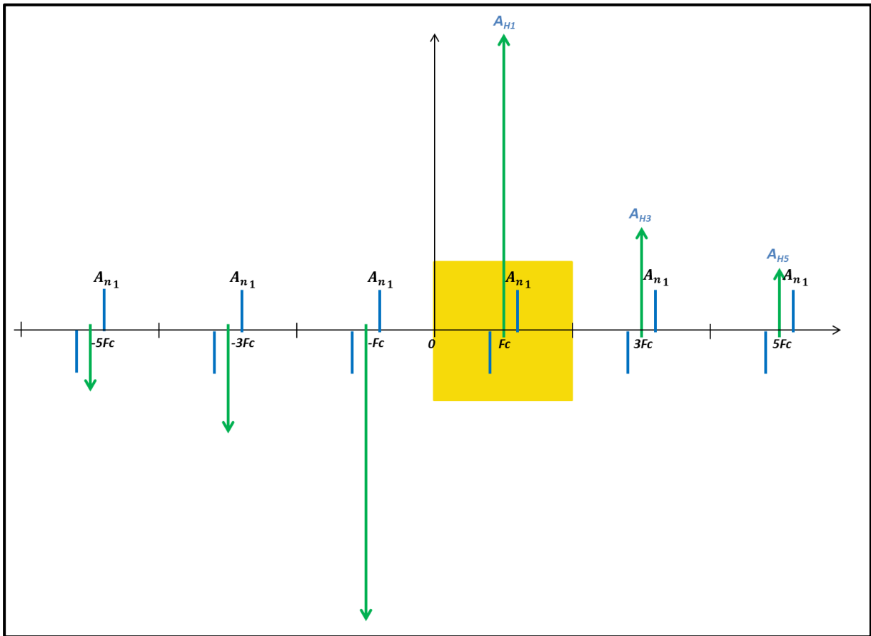
Figure 8-15: Freq. rep. of square modulated signal with Integration band 0->2*Fc
