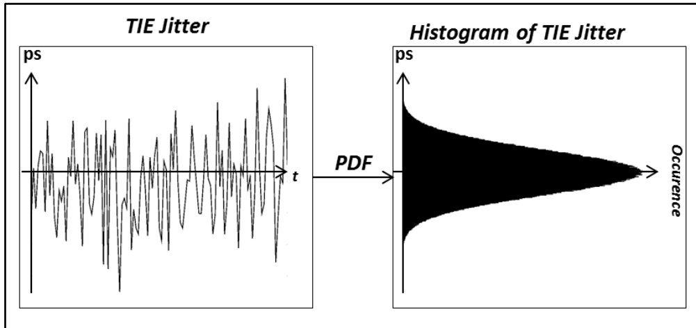
Figure 4-4: Histogram of PDF of the TIE Jitter
