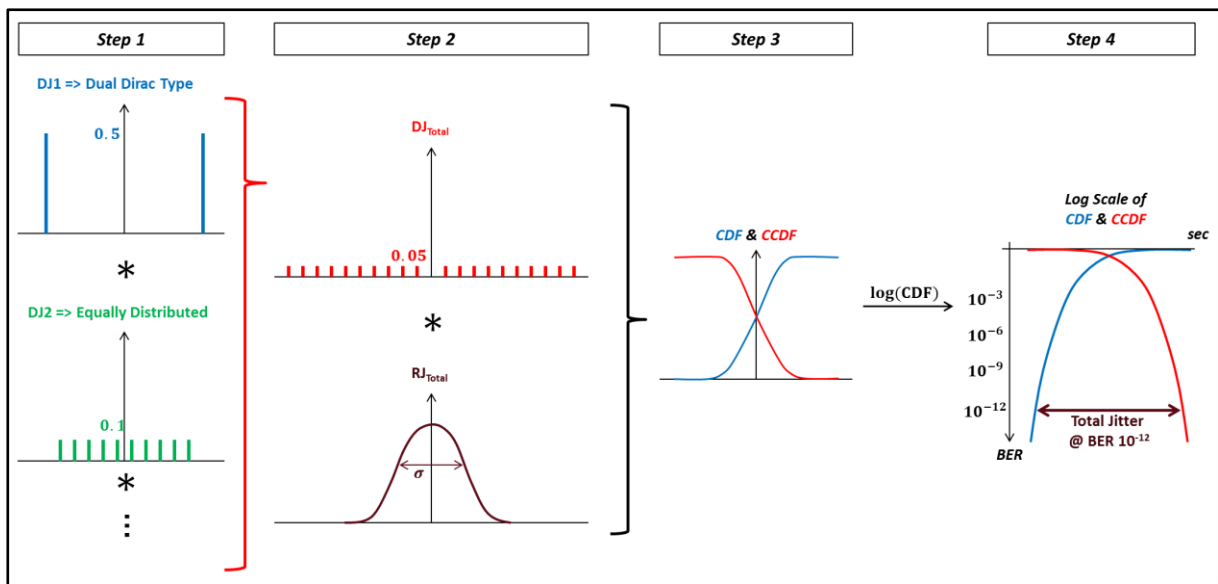
Figure 2-13: Total Jitter Estimation
