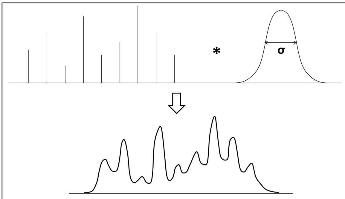
Figure 5-4: Jitter Decomposition proposed method
