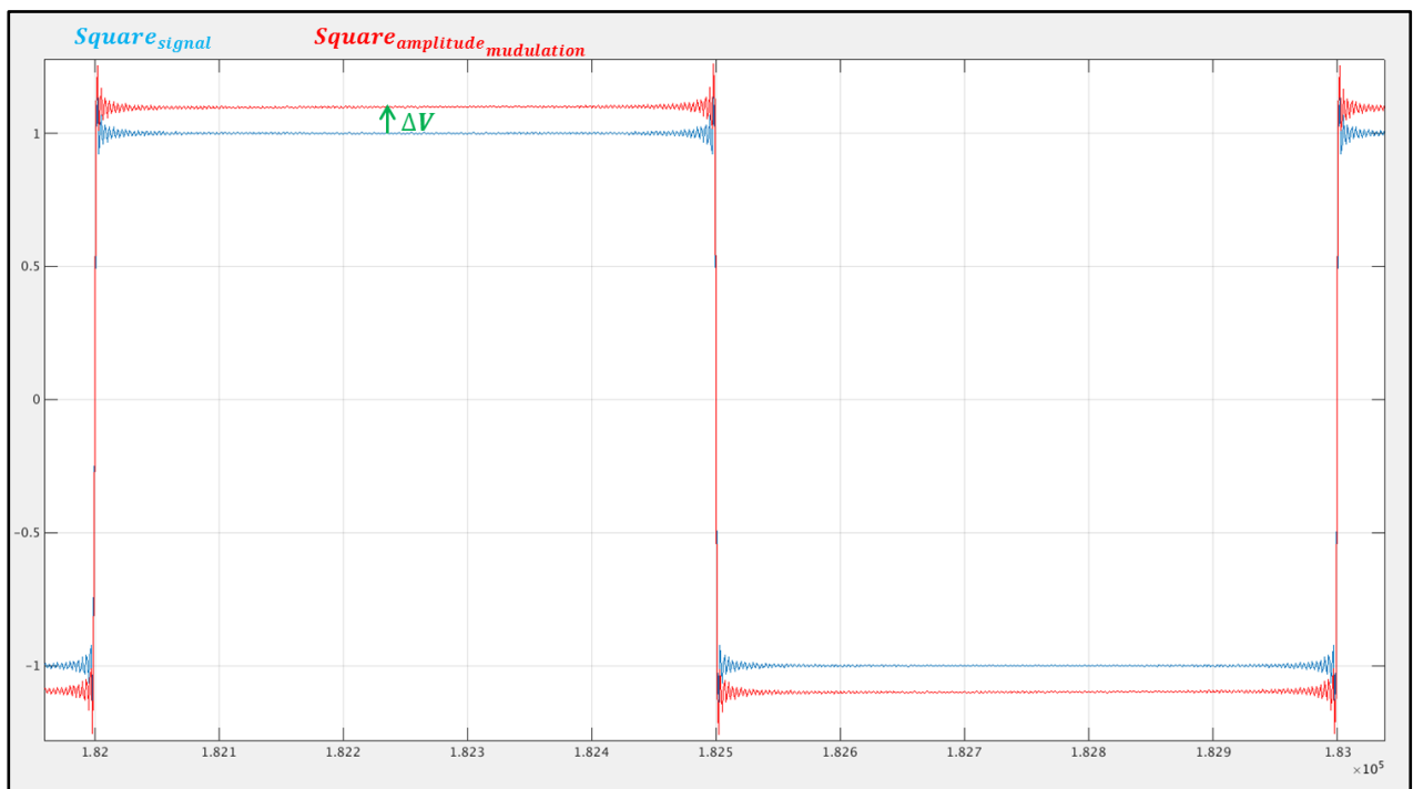
Figure 8-7: Amplitude Noise Modulation for Square Signal
