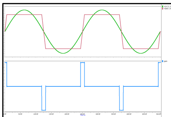
Figure 8-26: Noise Transfer Function of a square signal
