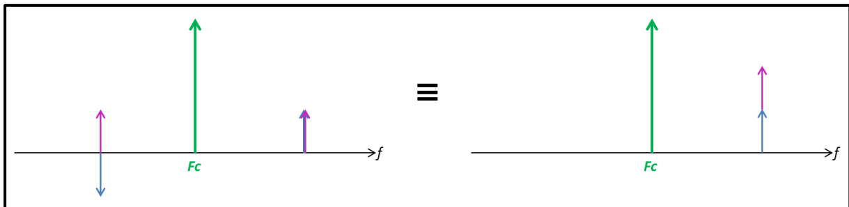
Figure 2-12: Amplitude & Phase Noise Modulation for Sinusoidal Signal
