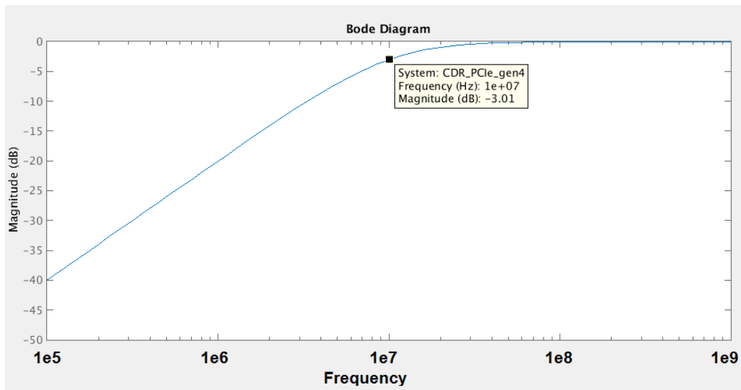
Figure 6-5: CDR Transfer Function
