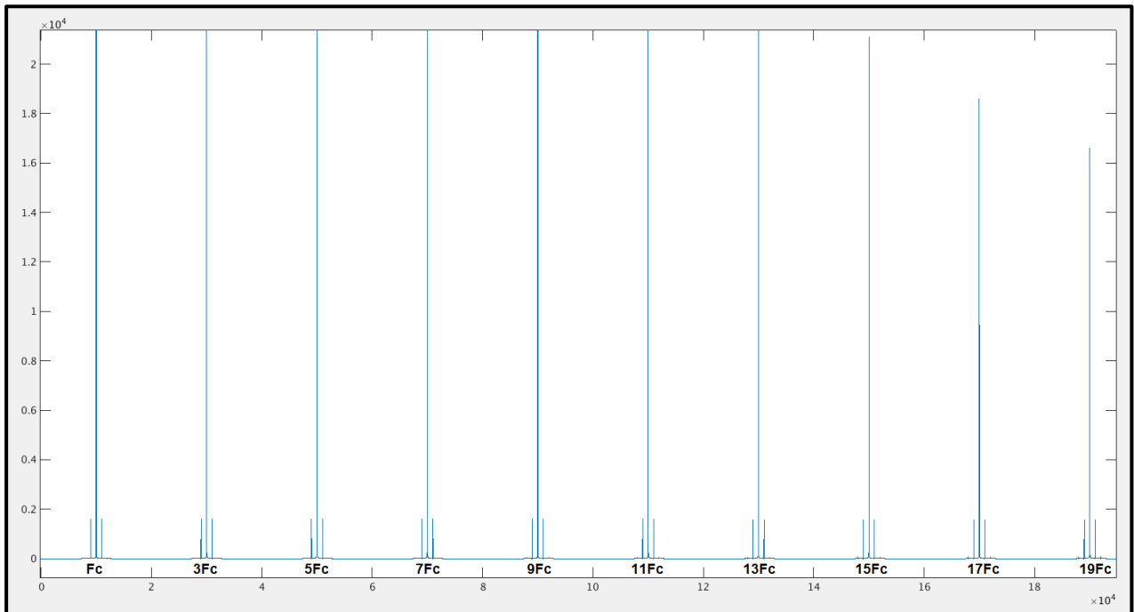
Figure 8-6: Phase Noise Modulation for Square Signal – Result of FFT
