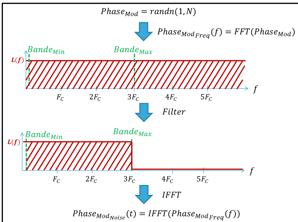
Figure 8-32: Creating frequency filtered phase noise
