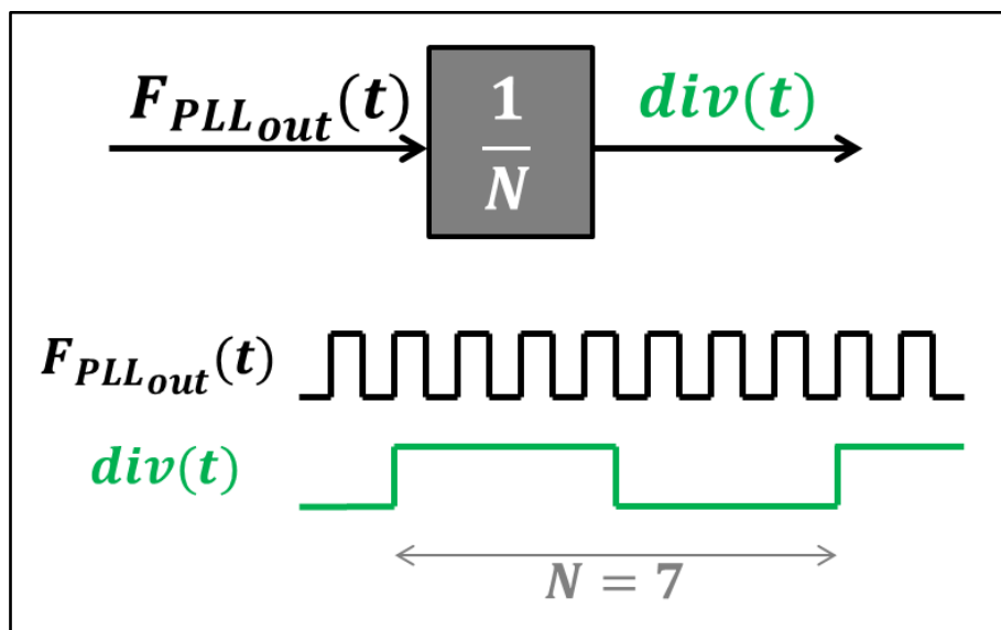
Figure 3-6: Divider
