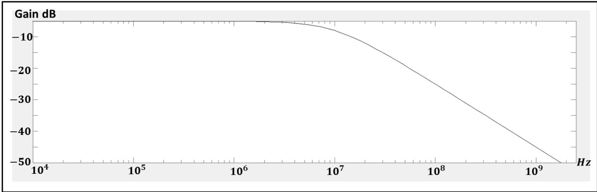
Figure 4-11: Filter Response for filtering white noise
