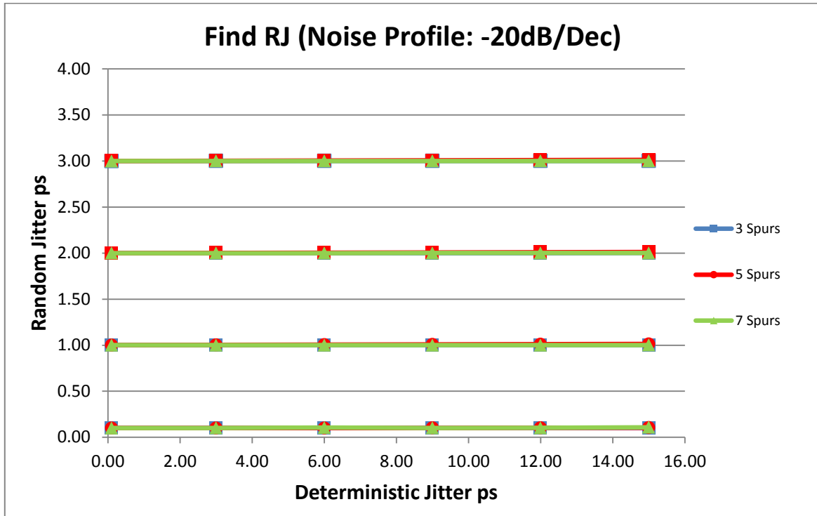
Figure 5-7: RJ for different quantities of generated RJ & DJ Jitter
