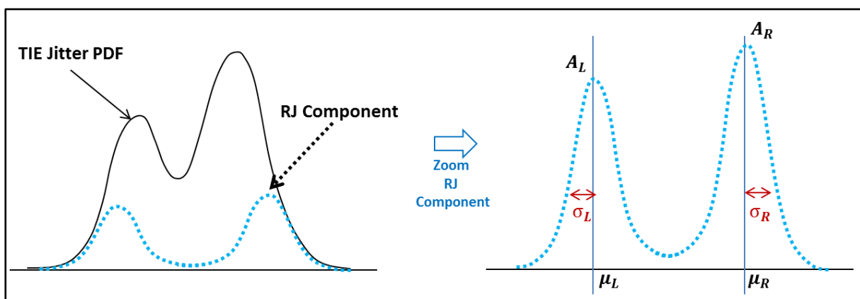
Figure 5-1: Tail Fitting Method for Jitter Decomposition
