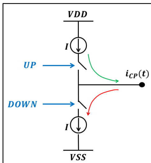
Figure 3-3: Charge Pump schematic
