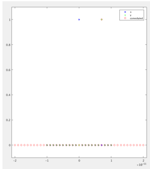
Figure 8-37: Example 1 - Convolution of 1*1 Dirac
