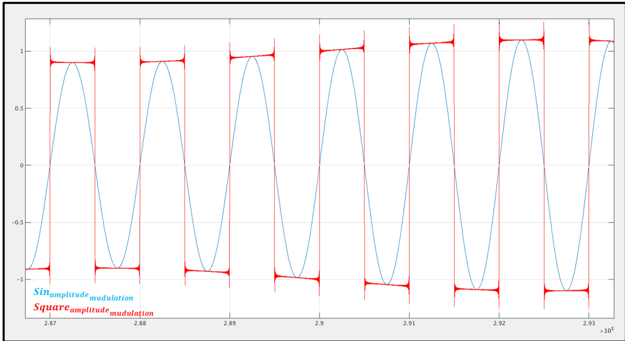
Figure 8-9: Time simulation of Amplitude Noise Sinusoidal & Square signal
