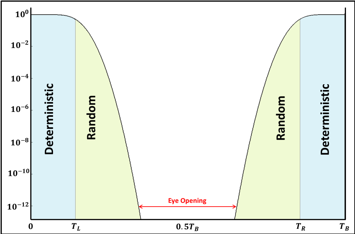
Figure 2-5: BER Graph
