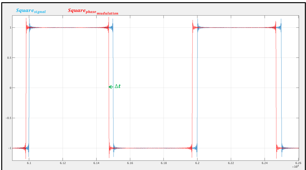
Figure 8-3: Phase Noise Modulation for Square Signal (Time Domain)
