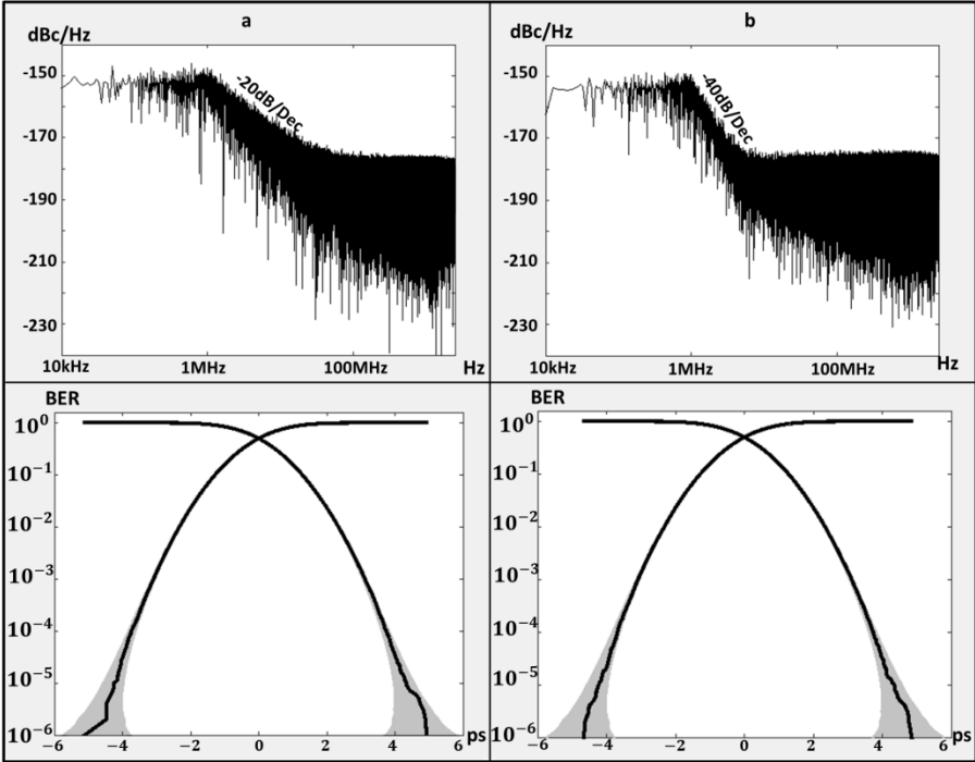
Figure 4-22: Generated colored noise profiles with Gaussian distribution.
