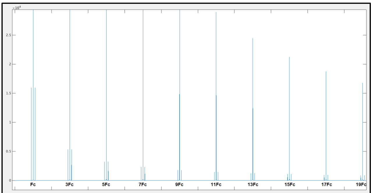
Figure 8-10: Amplitude Noise Modulation for Square Signal – Result of FFT
