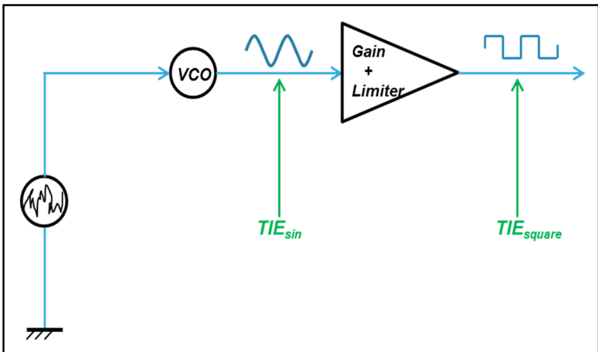
Figure 8-12: Convert Noisy Sinusoidal signal to Noisy Square Signal
