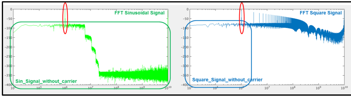
Figure 8-34: FFT of Sinusoidal & Square Noisy Signal - Matlab
