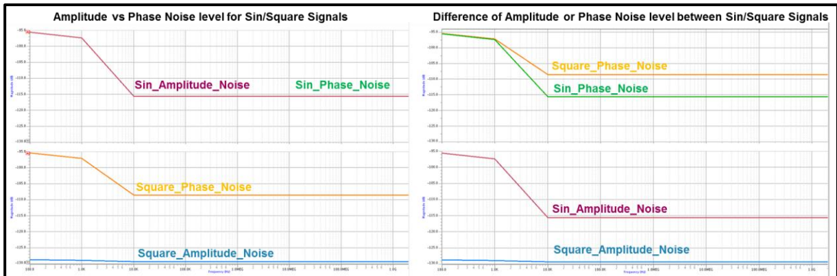
Figure 8-25: Amplitude & Phase noise for Sinusoidal/Square signal
