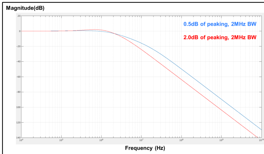
Figure 6-6: Comparison between 2 different PLL BW
