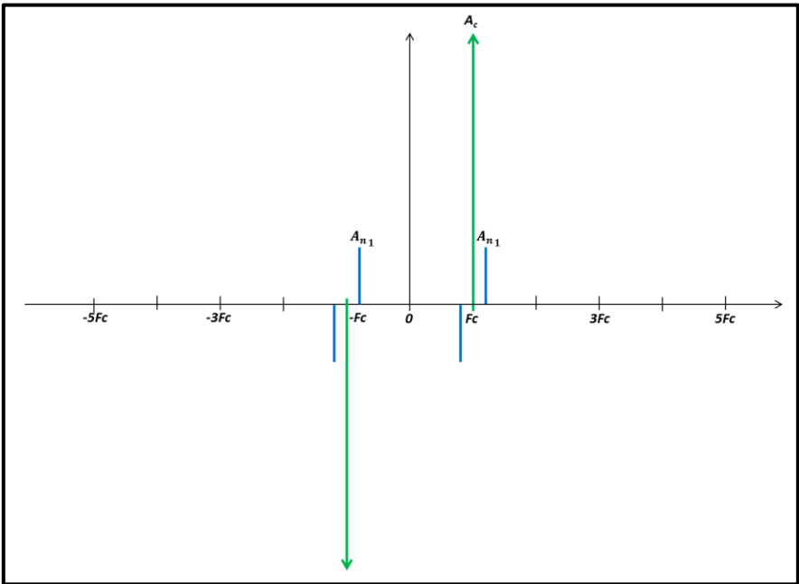
Figure 8-13: Frequency representation of the sinusoidal modulated signal
