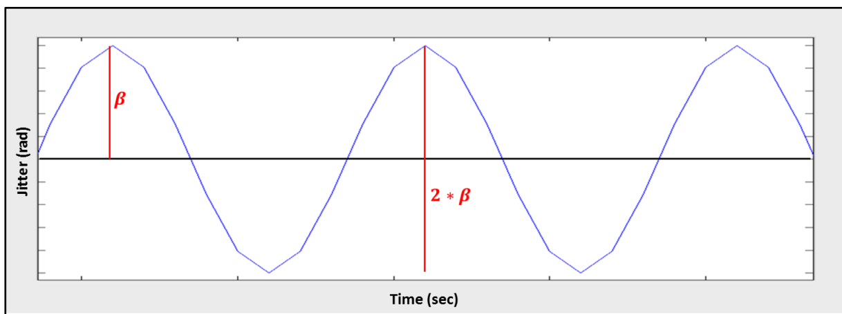
Figure 2-6: Time Domain Phase Modulation
