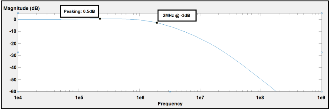
Figure 6-4: Closed Loop Response
