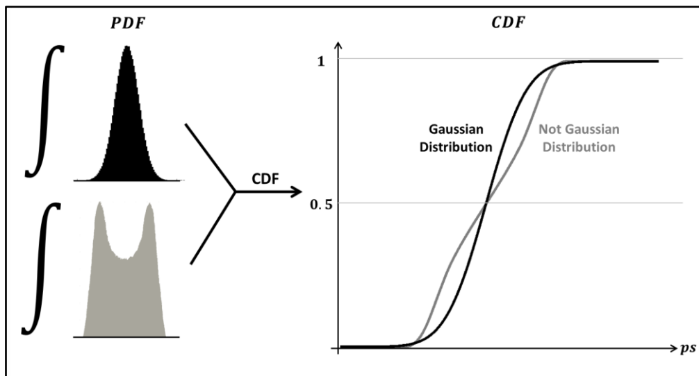
Figure 4-5: CDF Calculation from PDF
