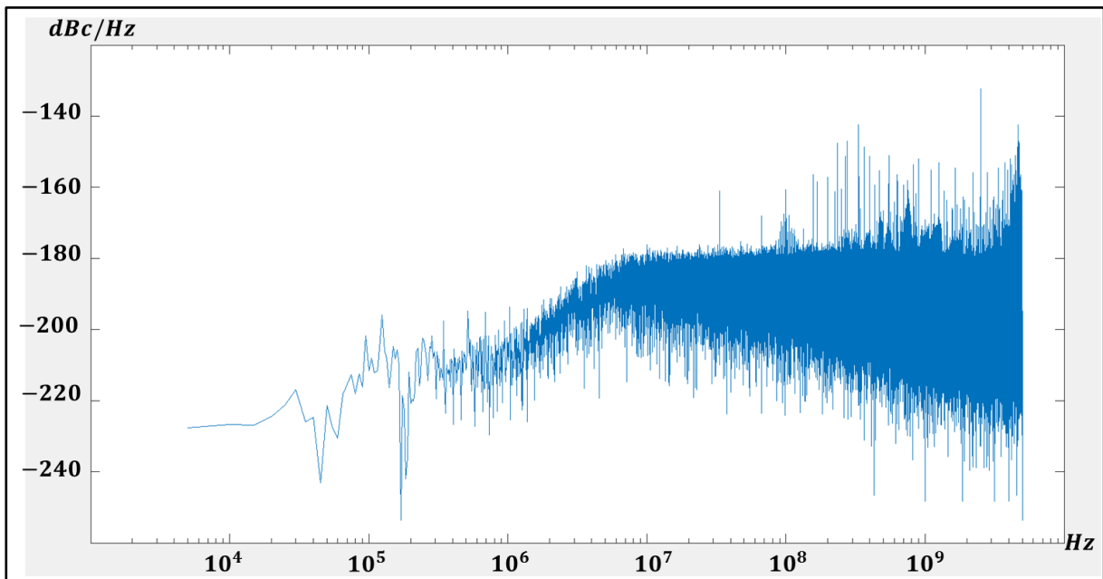
Figure 5-9: DJ Spurs when no DJ is injected
