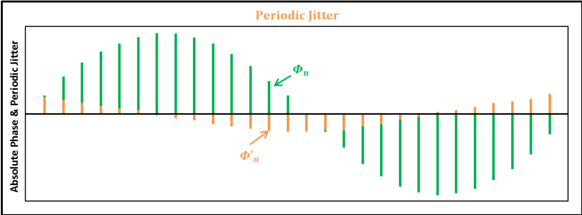
Figure 2-3: Periodic Jitter
