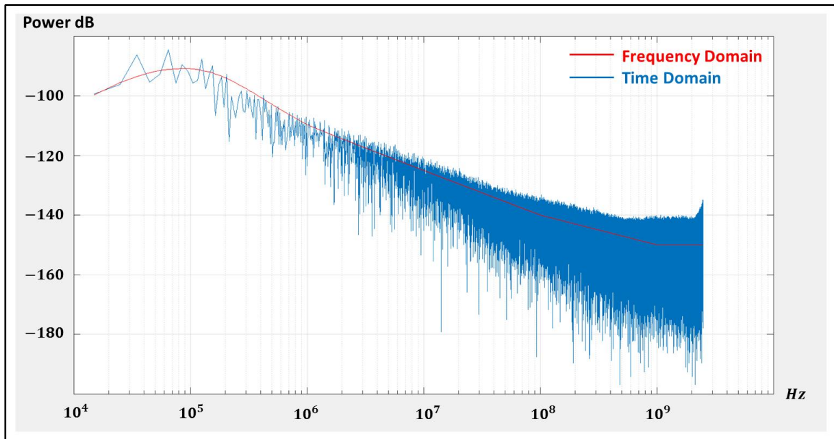
Figure 3-17: VCO Phase Noise at the PLL Output for Frequency & Time Domain Models
