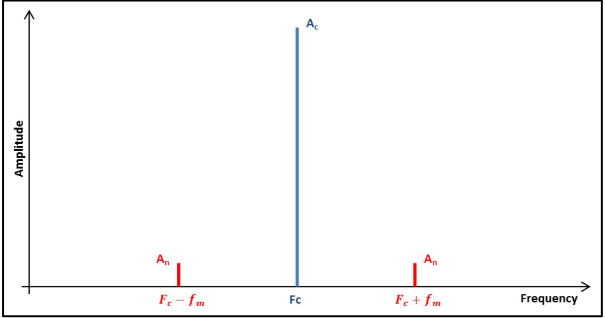
Figure 2-7: Frequency Representation of the modulated signal
