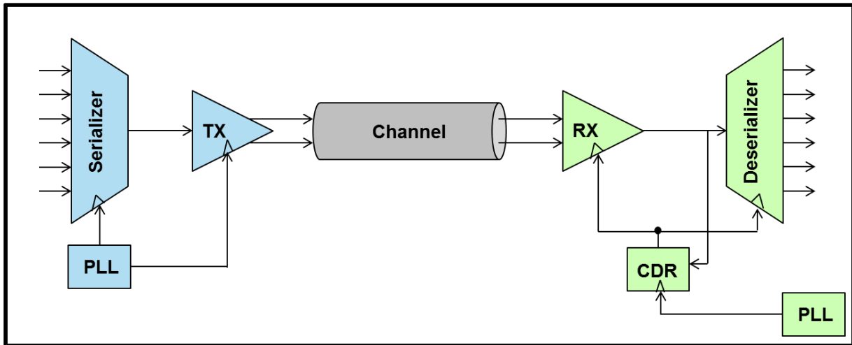
Figure 1-7: High Speed Serial Links System
