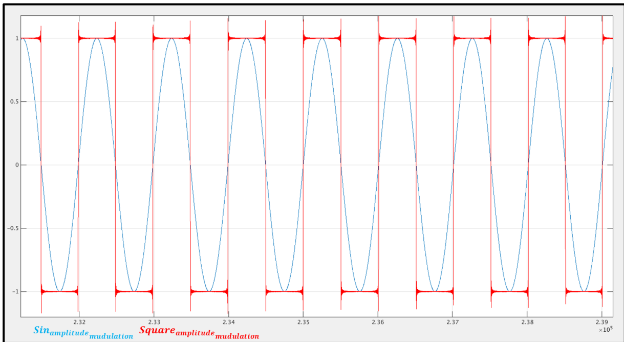
Figure 8-5: Time simulation of Phase Noise Sinusoidal & Square signal
