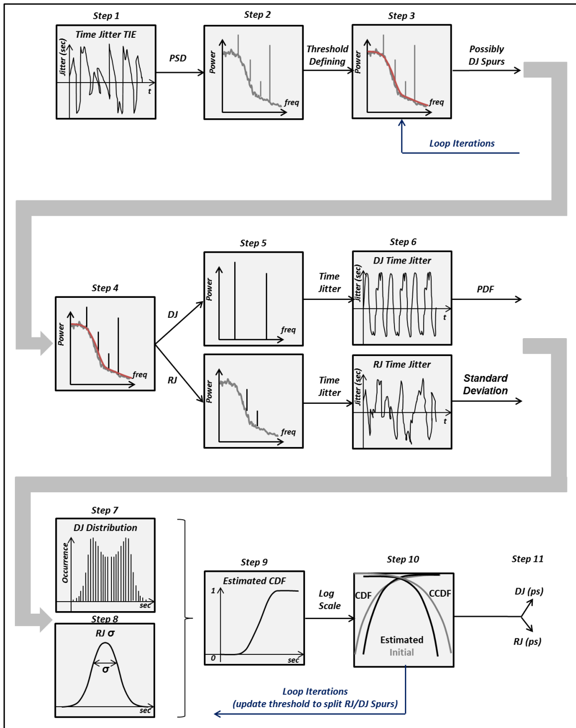
Figure 5-5: Jitter Decomposition Algorithm
