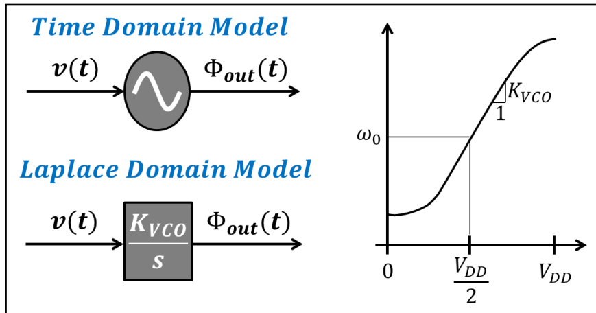
Figure 3-5: VCO
