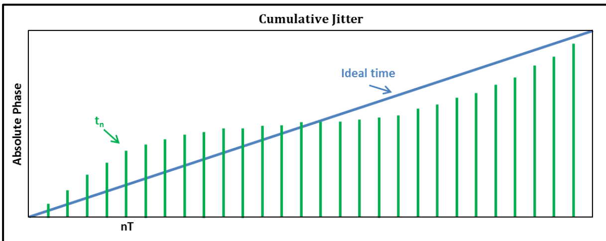
Figure 2-2: Cumulative Jitter
