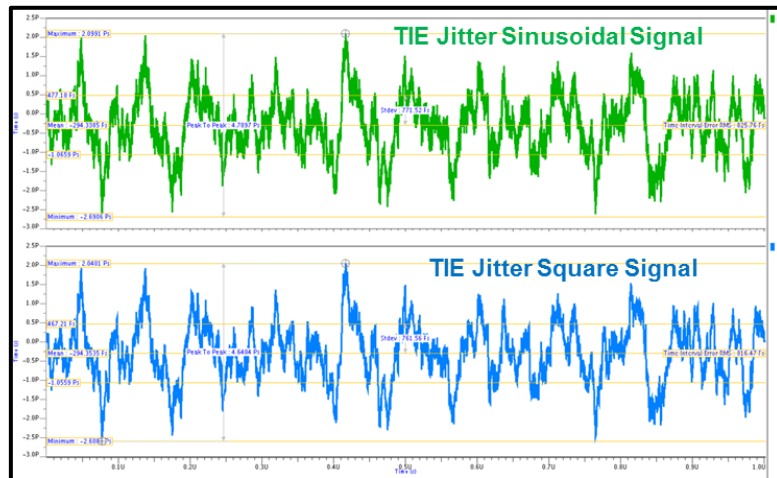
Figure 8-29: Sin/Square Signals TIE Jitter
