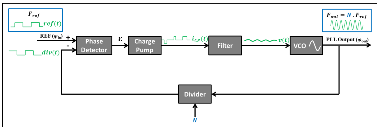
Figure 3-1: PLL Architecture
