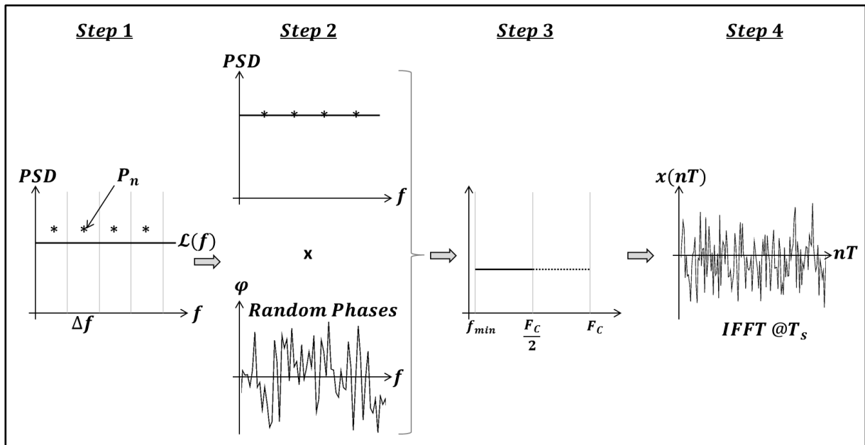
Figure 4-8: Time jitter generation from phase noise profiles.
