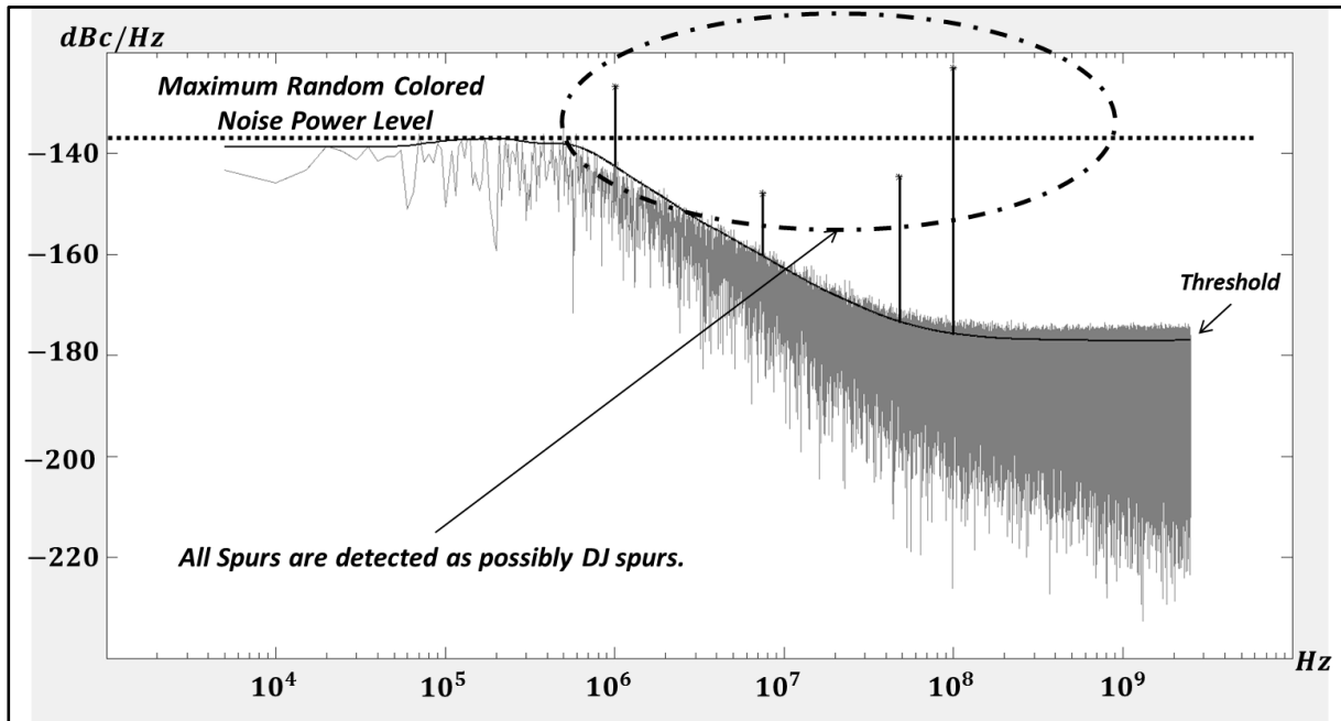
Figure 5-6: All DJ spurs detected by algorithm
