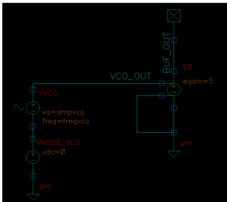
Figure 8-24: Eldo Simulation Schematic
