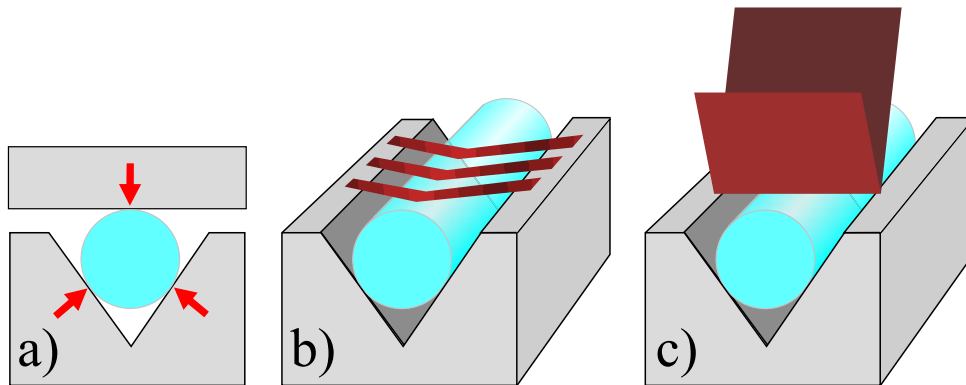
Figure 3.6: Multi fiber holder with v-grooves. a) shows the widely used principle of v-grooves for fiber fixation. The three red arrows mark the contact lines that align the fiber. The gray rectangle on top depicts the glass or silica piece that is normally glued on top. b) shows the possibility of fixing the fiber temporarily with metallic micro clamps and c) shows the solution with macroscopic clamps not directly attached to the groove substrate.
