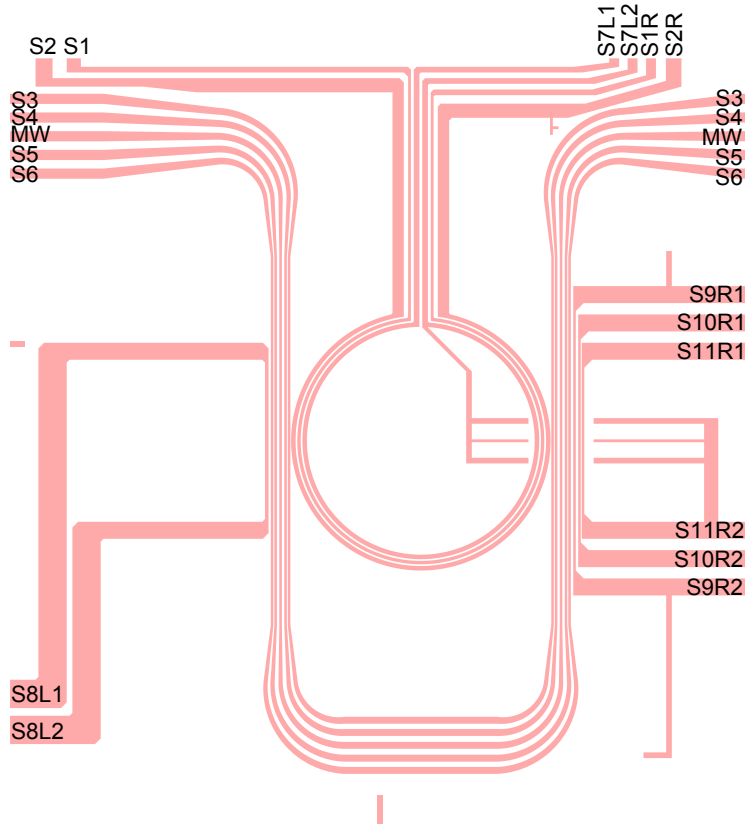
Figure A.6: Labeled science chip (cf. Sec. 5.2).
