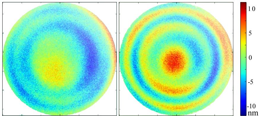
Figure 3.4: Residual depending on profilometry position. The same surface was scanned twice with a distance offset of \lambda_P/8 and fitted with a 2D-paraboloid, the edge length is 60 \mu\text{m} . The residuals shown have a sinusoidal modulation, dependent on the initial profilometry position. Averaging two profiles with such a distance offset reduces strongly the spurious effects of the reconstruction algorithm.
