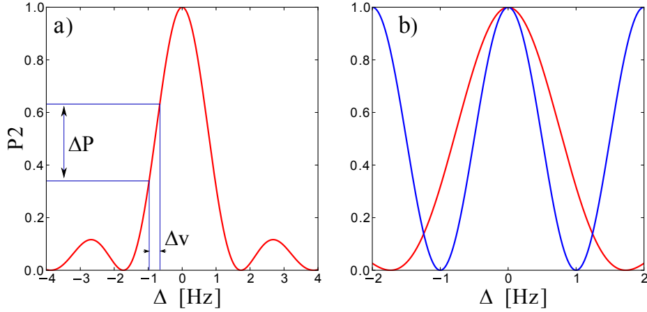
Figure 1.2: a) Rabi pulse following Eq. 1.1.3 with \Omega_R = 1 and t = \pi . For \Delta = 0 , the atomic state is fully transferred to |2\rangle . A pulse realizing the full transfer is referred to as a \pi -pulse. b) Comparing the spectroscopic response of the Rabi pulse from a) (red) with a Ramsey sequence (blue) with the same duration T_R = \pi .
