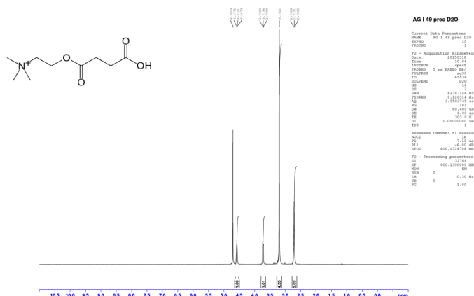
Figure 10 : Spectre RMN de la succinyl-monocholine.
